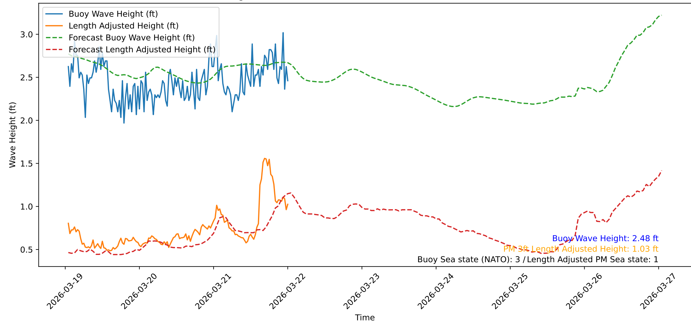
Wave Heights over Time for Oceanside Harbor at 2026-03-22 00:50:32
