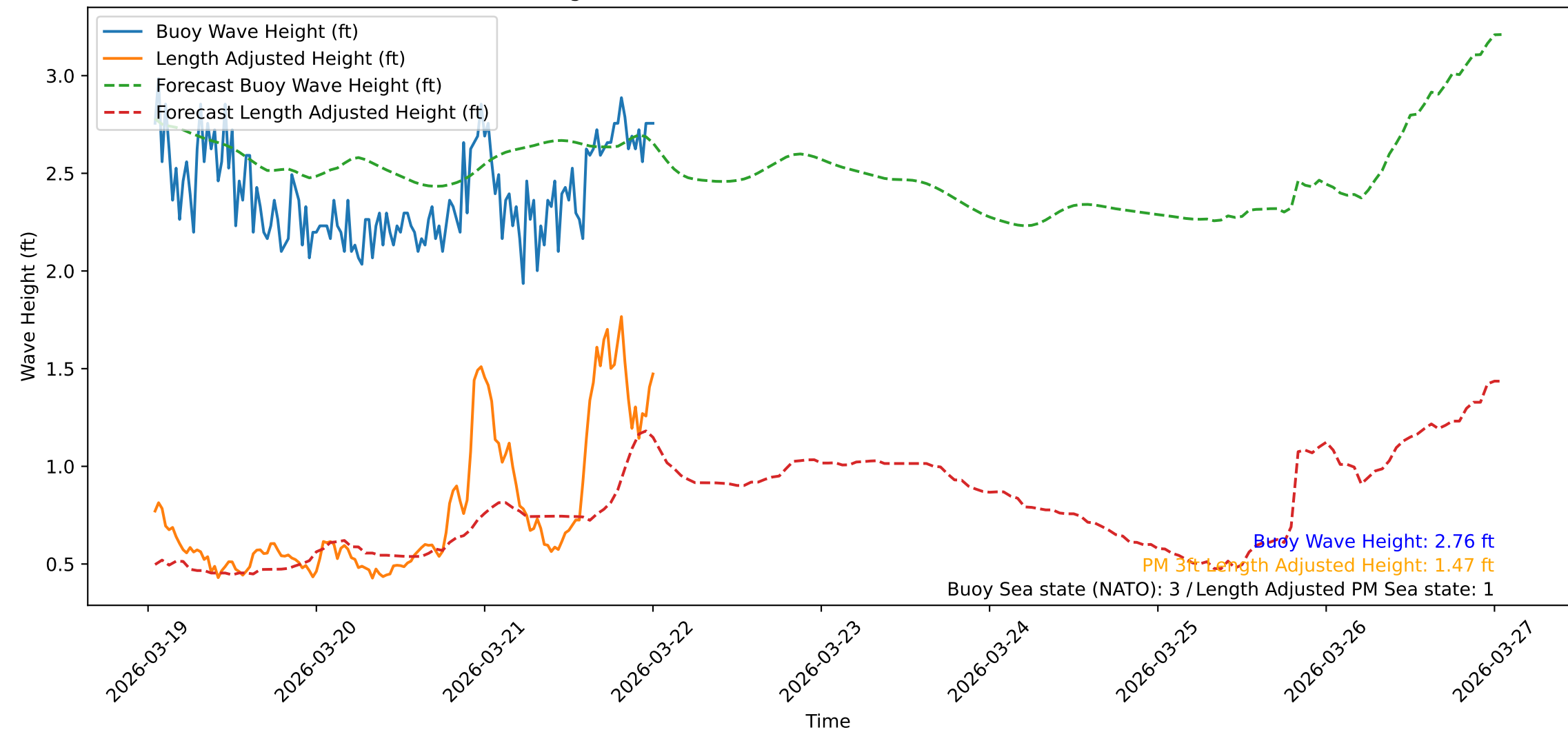
Wave Heights over Time for Green Beach at 2026-03-22 00:51:11
