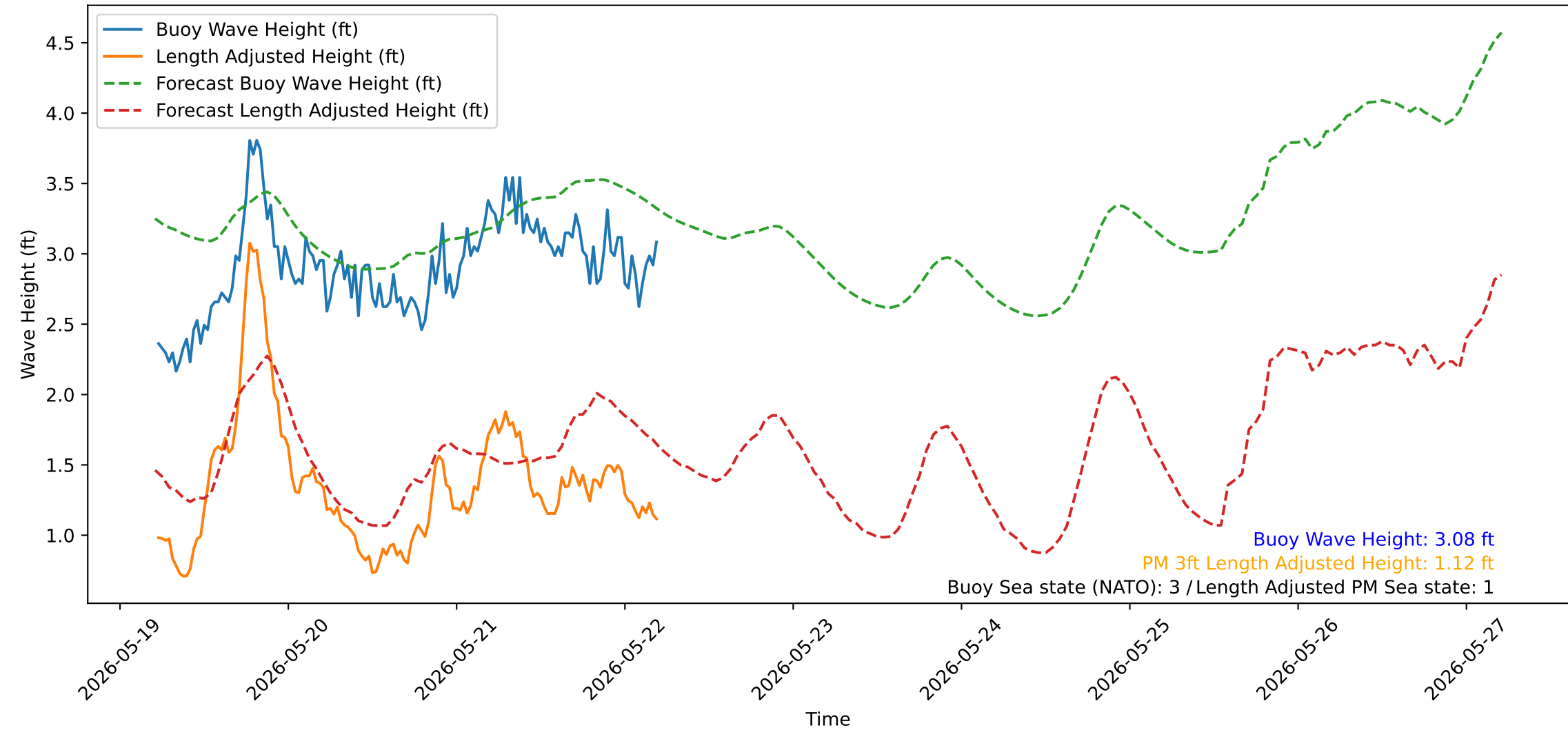
Wave Heights over Time for Green Beach at 2026-05-22 05:21:14
