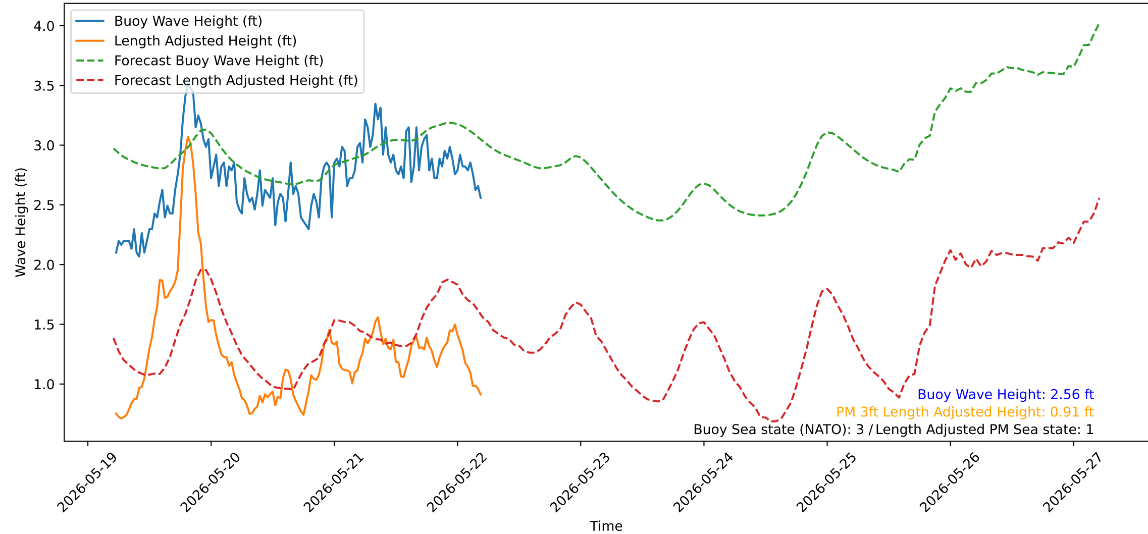
Wave Heights over Time for Red Beach at 2026-05-22 05:20:52
