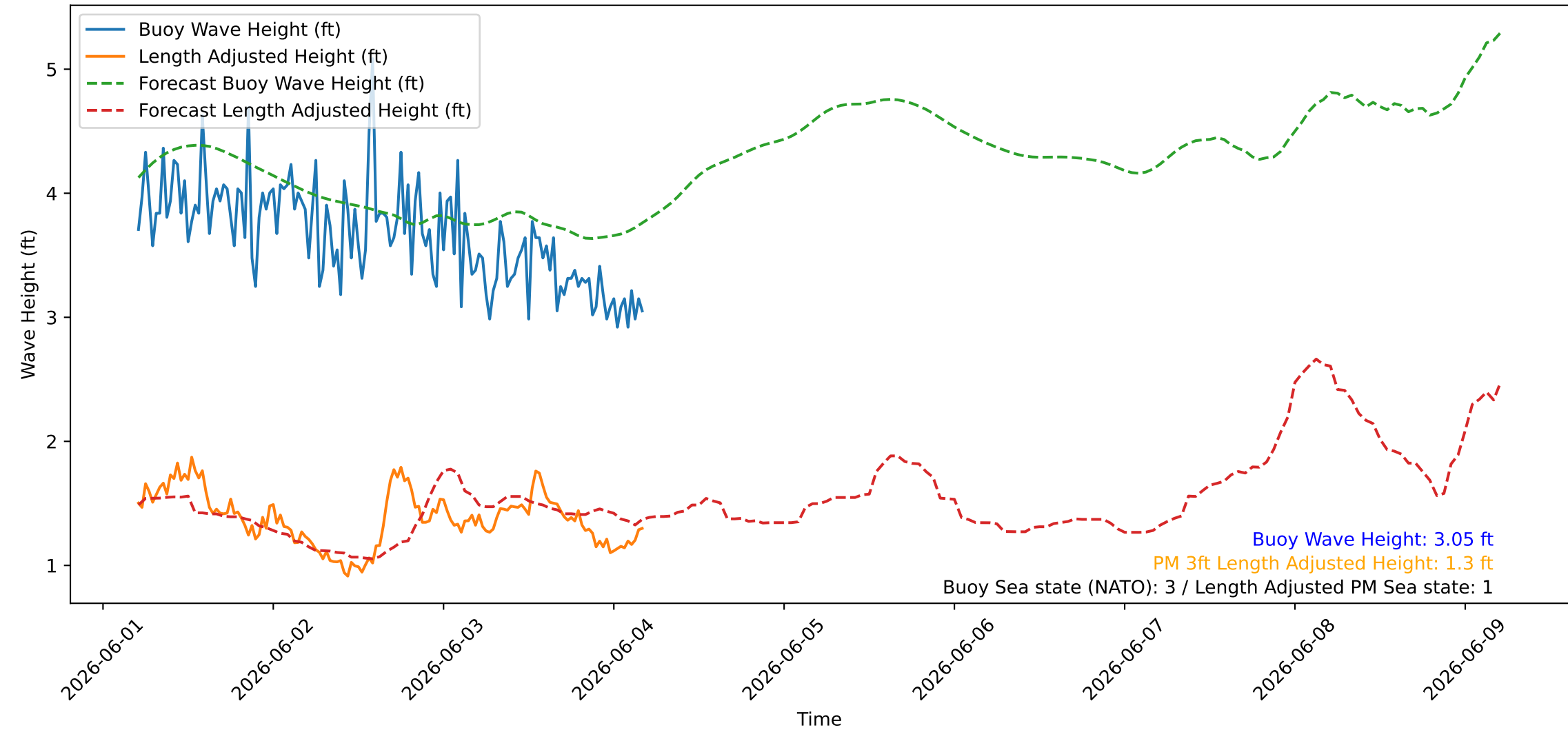
Wave Heights over Time for Oceanside Harbor at 2026-06-04 04:50:26
