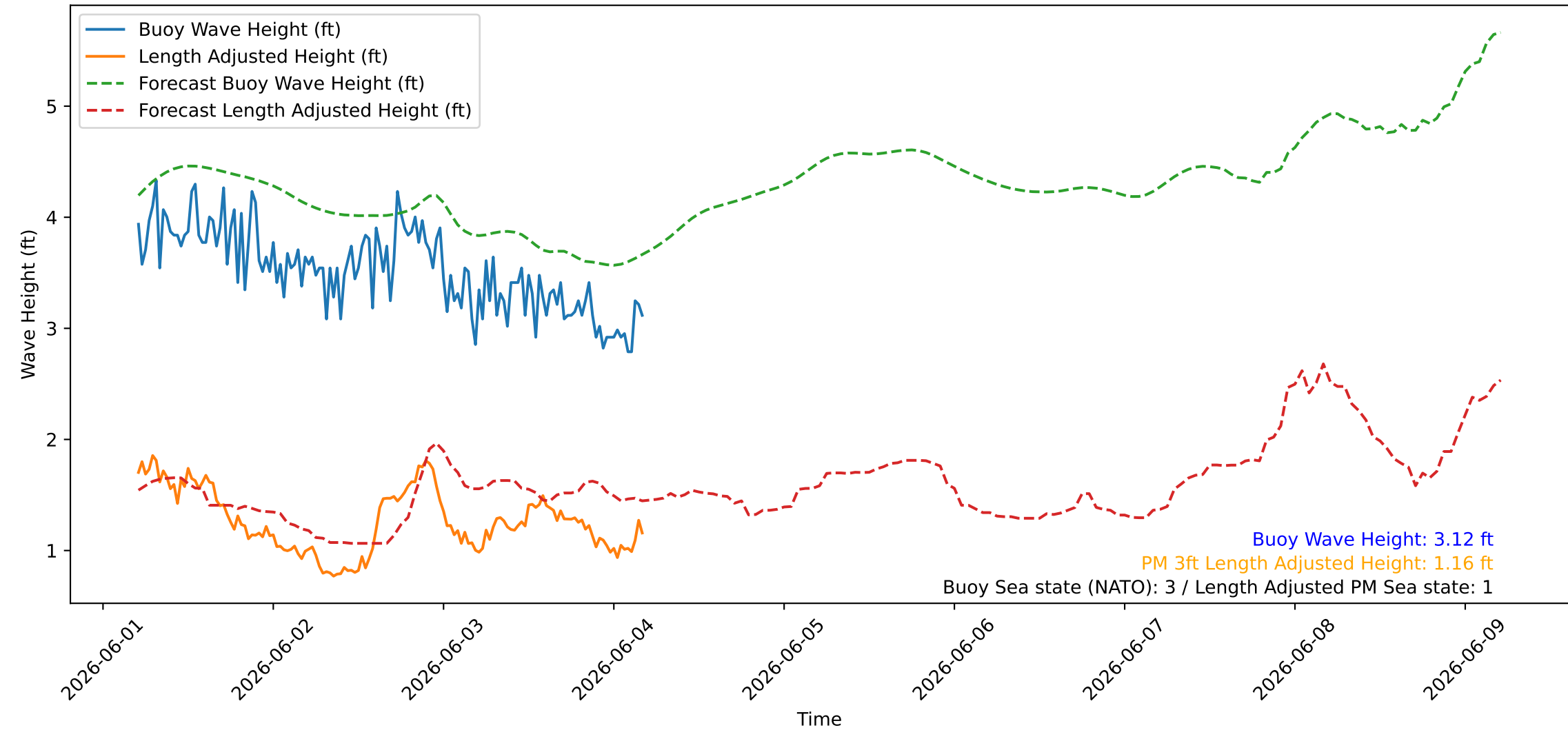
Wave Heights over Time for Green Beach at 2026-06-04 04:51:09
