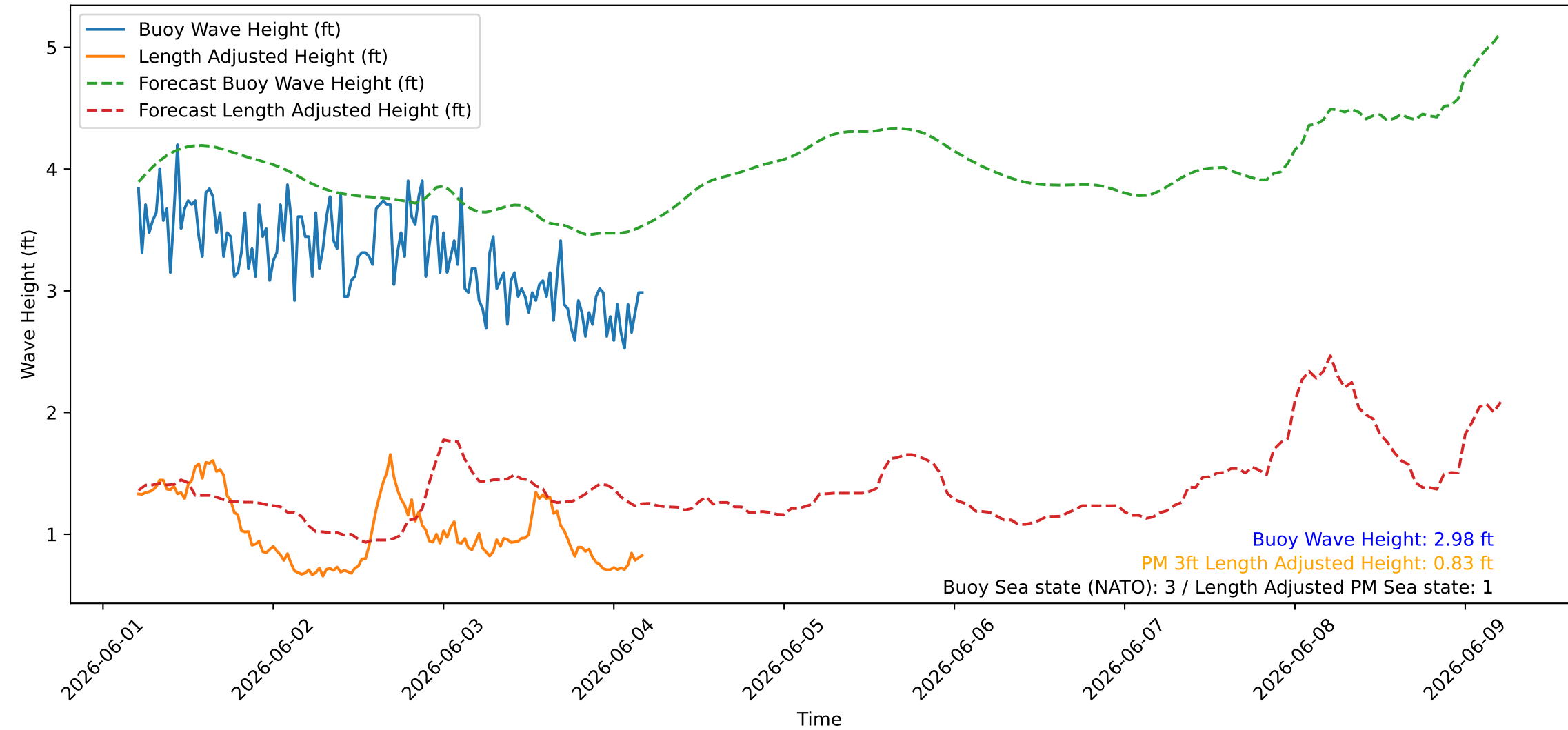
Wave Heights over Time for Red Beach at 2026-06-04 04:50:47
