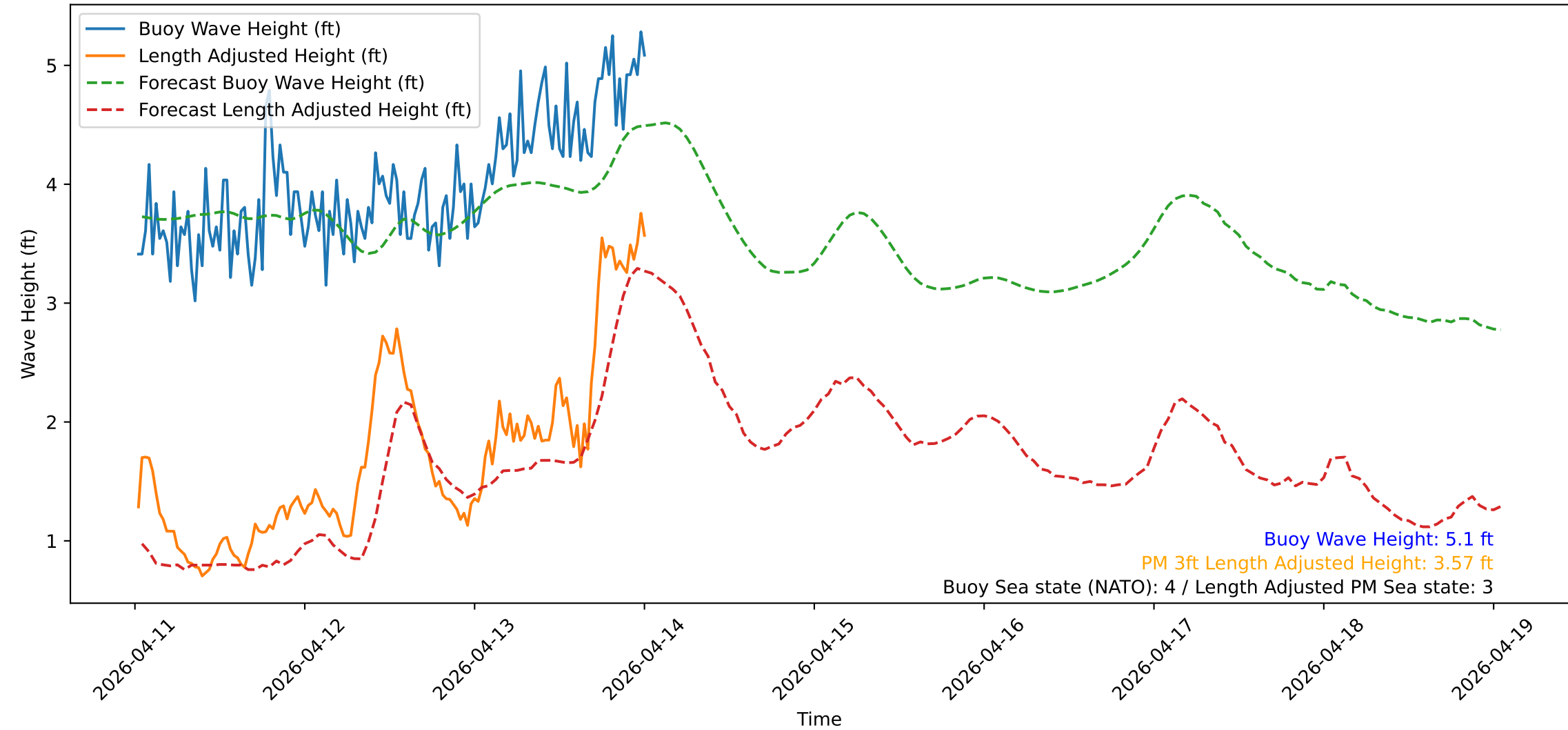
Wave Heights over Time for Oceanside Harbor at 2026-04-14 00:40:32
