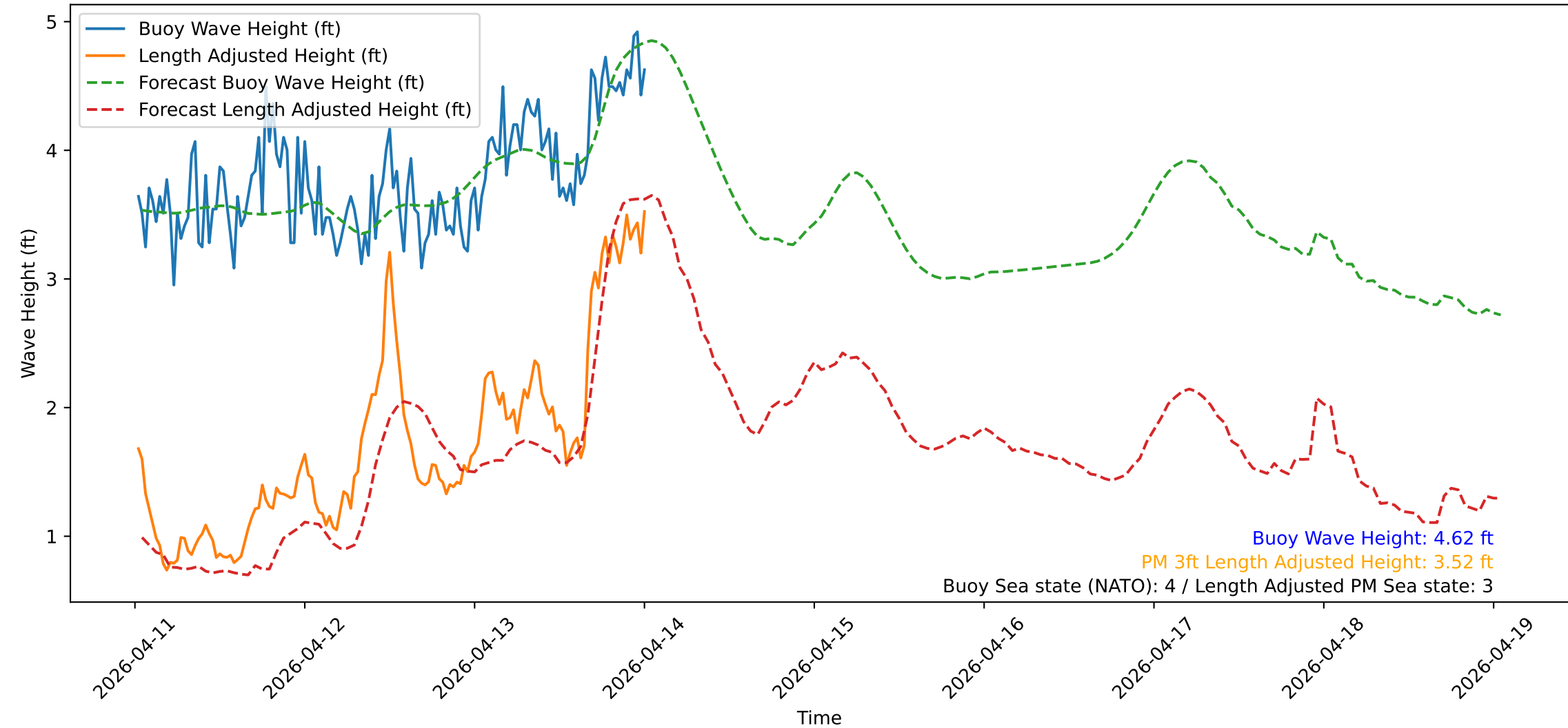
Wave Heights over Time for Green Beach at 2026-04-14 00:41:14
