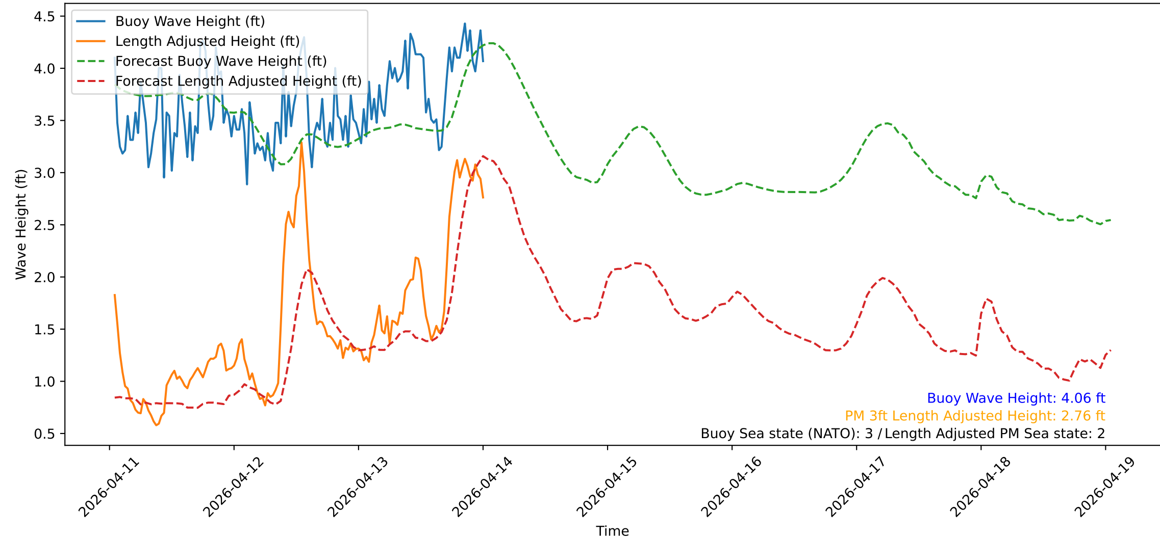
Wave Heights over Time for Red Beach at 2026-04-14 00:40:51
