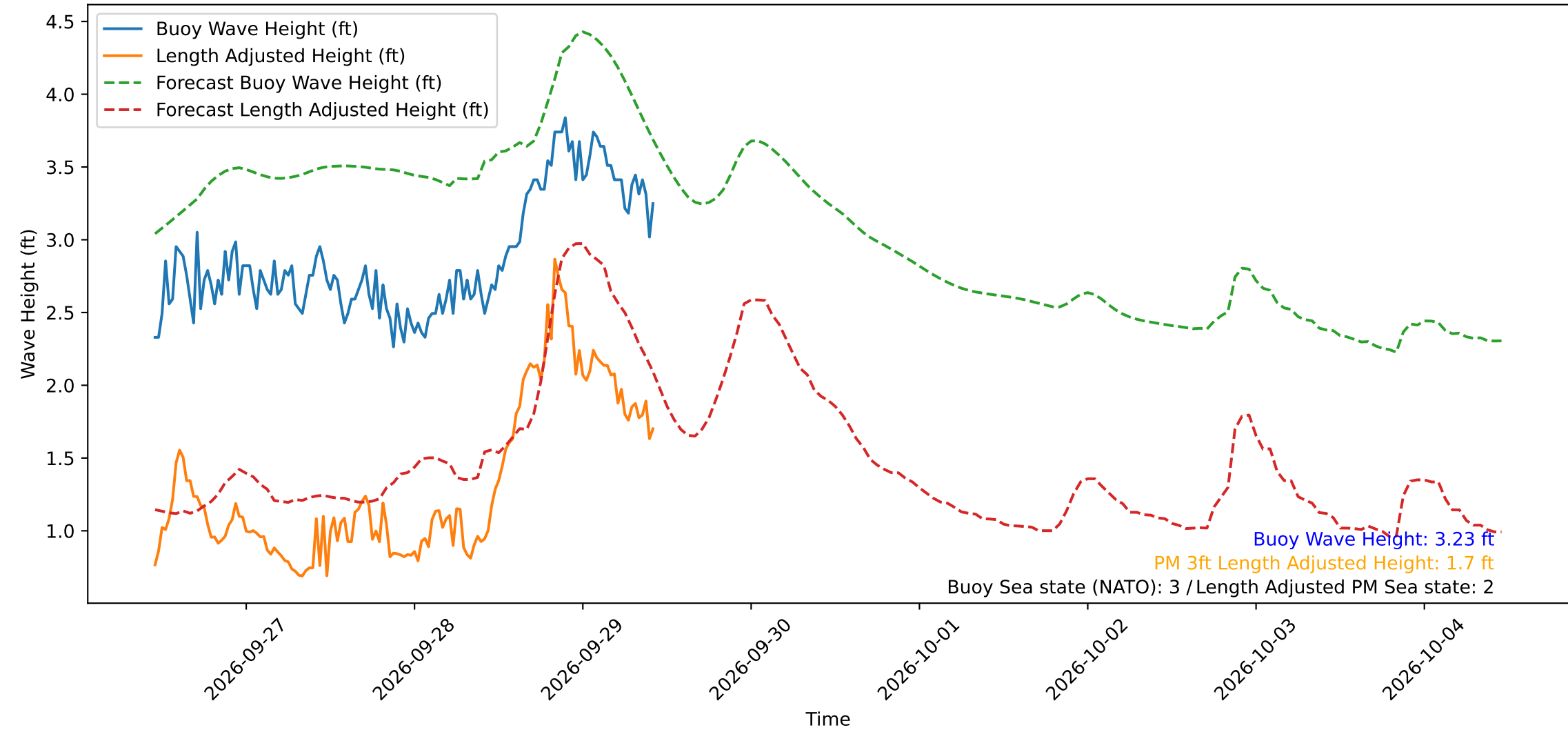
Wave Heights over Time for Red Beach at 2026-09-29 10:50:50
