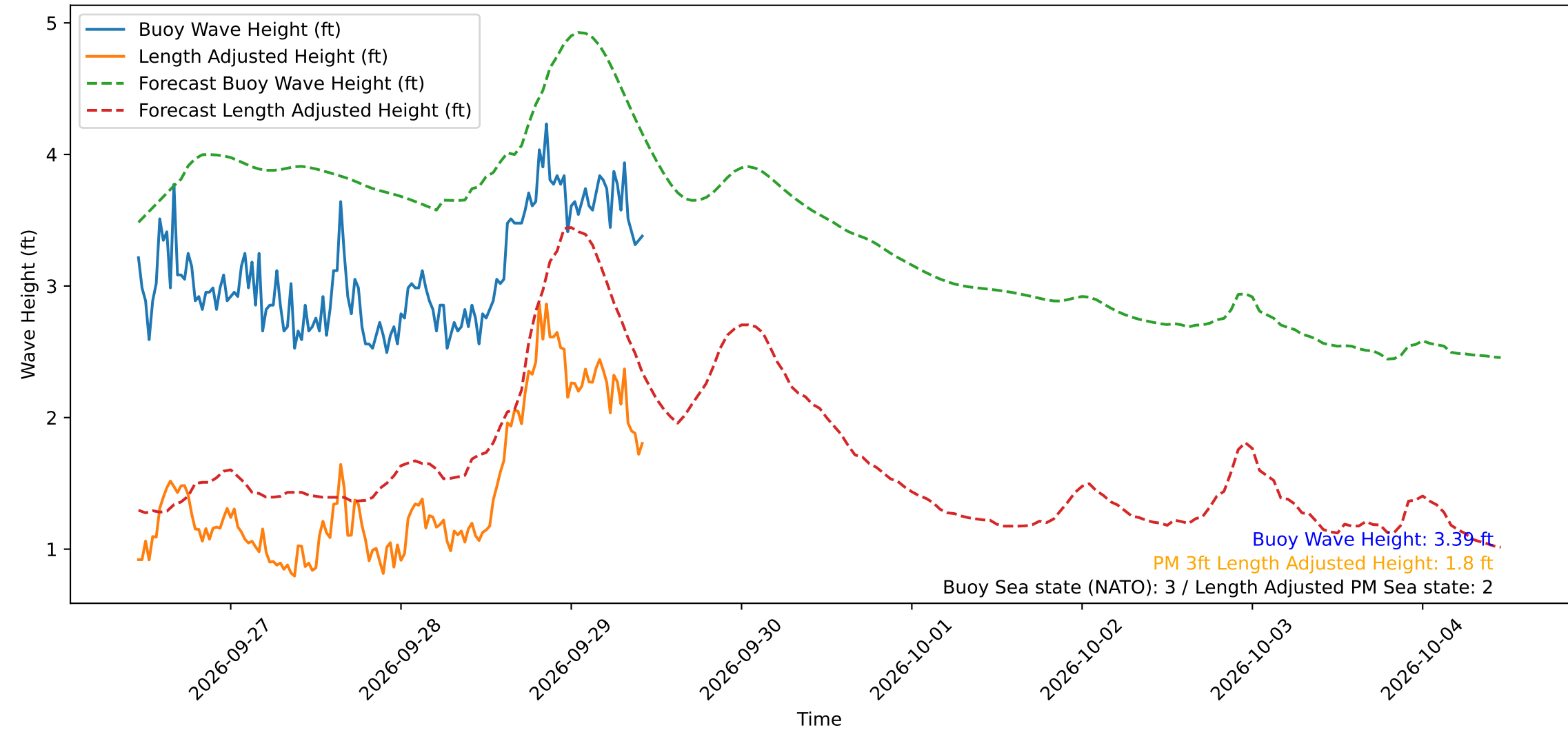
Wave Heights over Time for Oceanside Harbor at 2026-09-29 10:50:29
