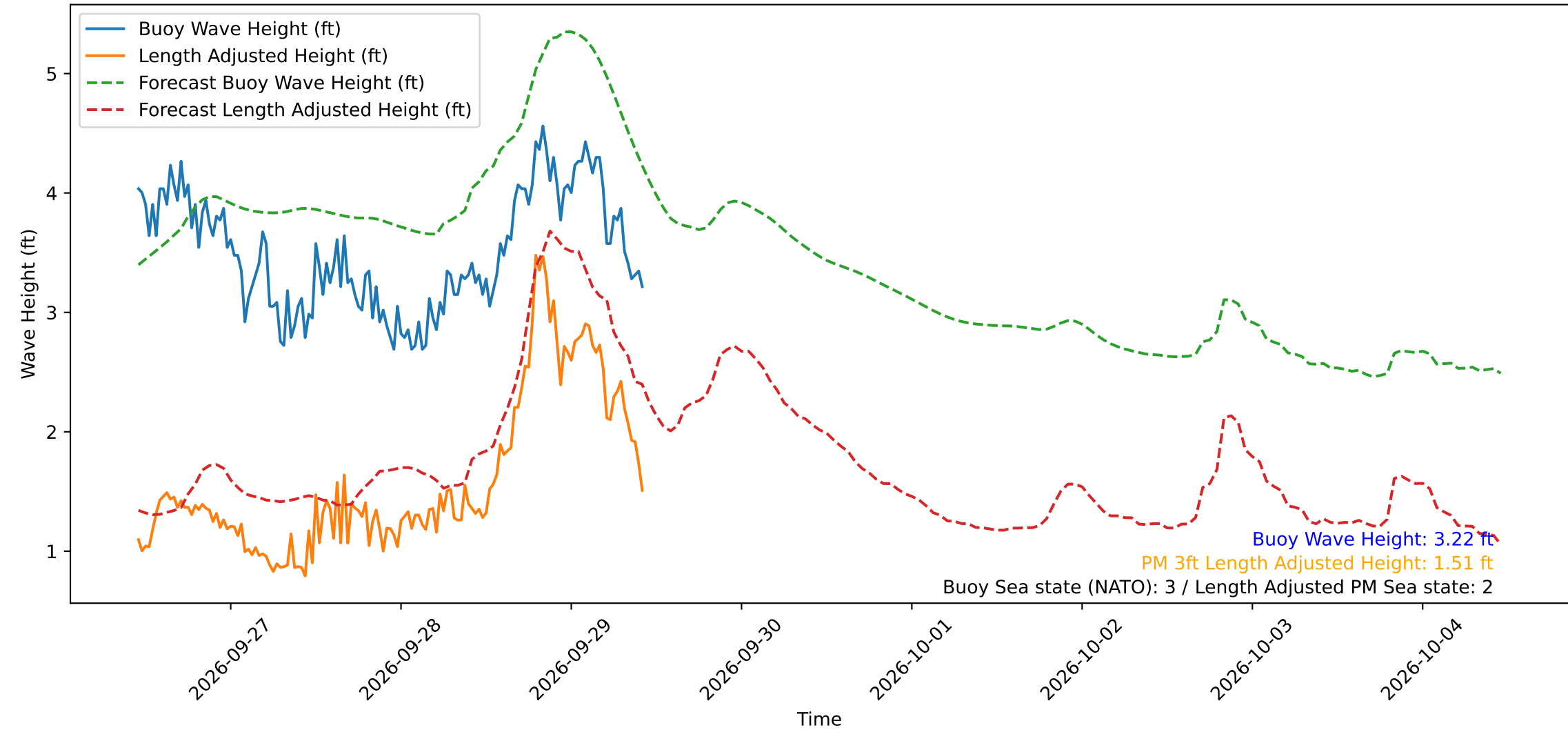
Wave Heights over Time for Green Beach at 2026-09-29 10:51:15
