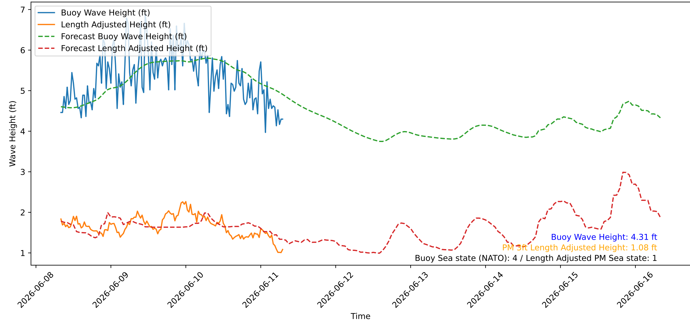
Wave Heights over Time for Green Beach at 2026-06-11 08:01:09
