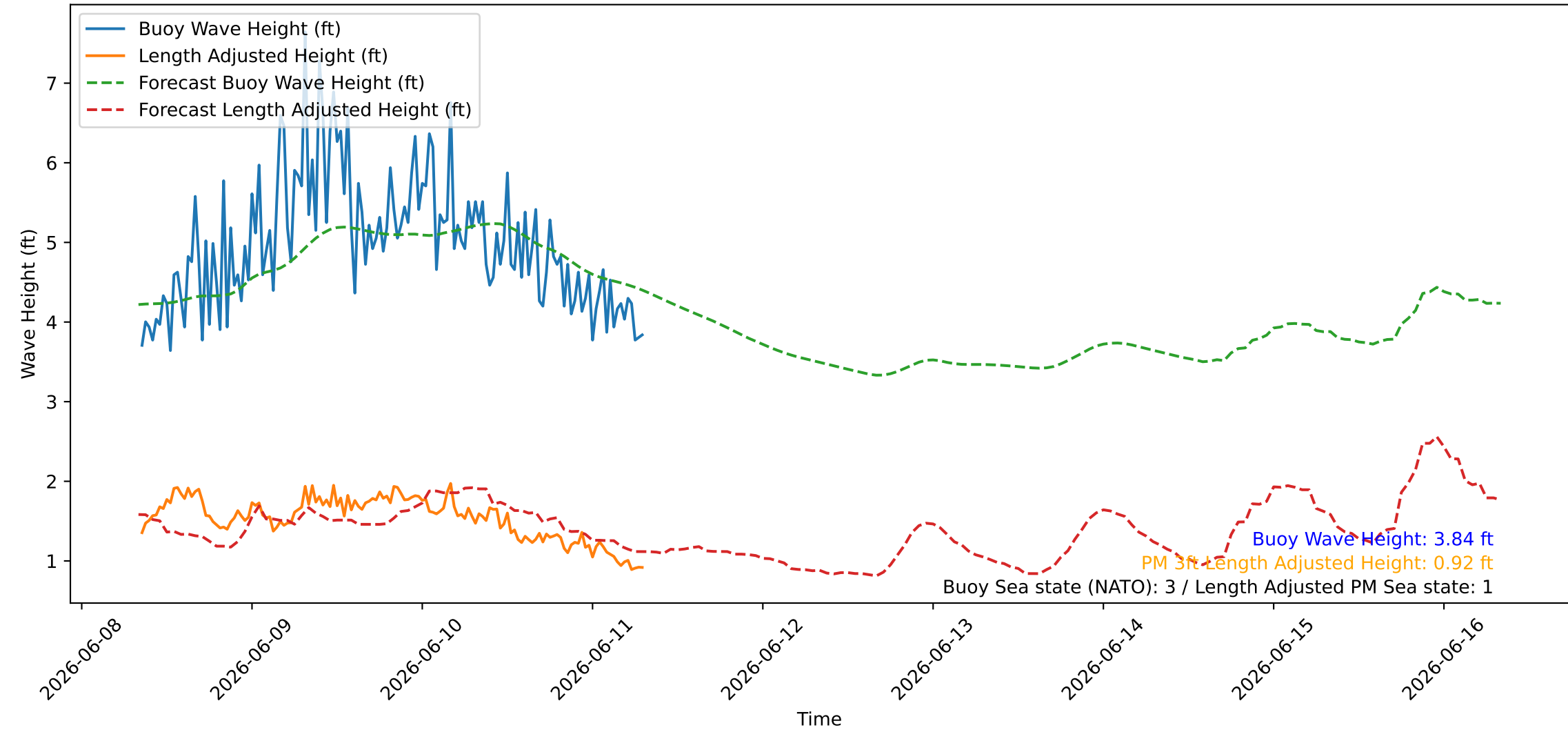
Wave Heights over Time for Red Beach at 2026-06-11 08:00:46
