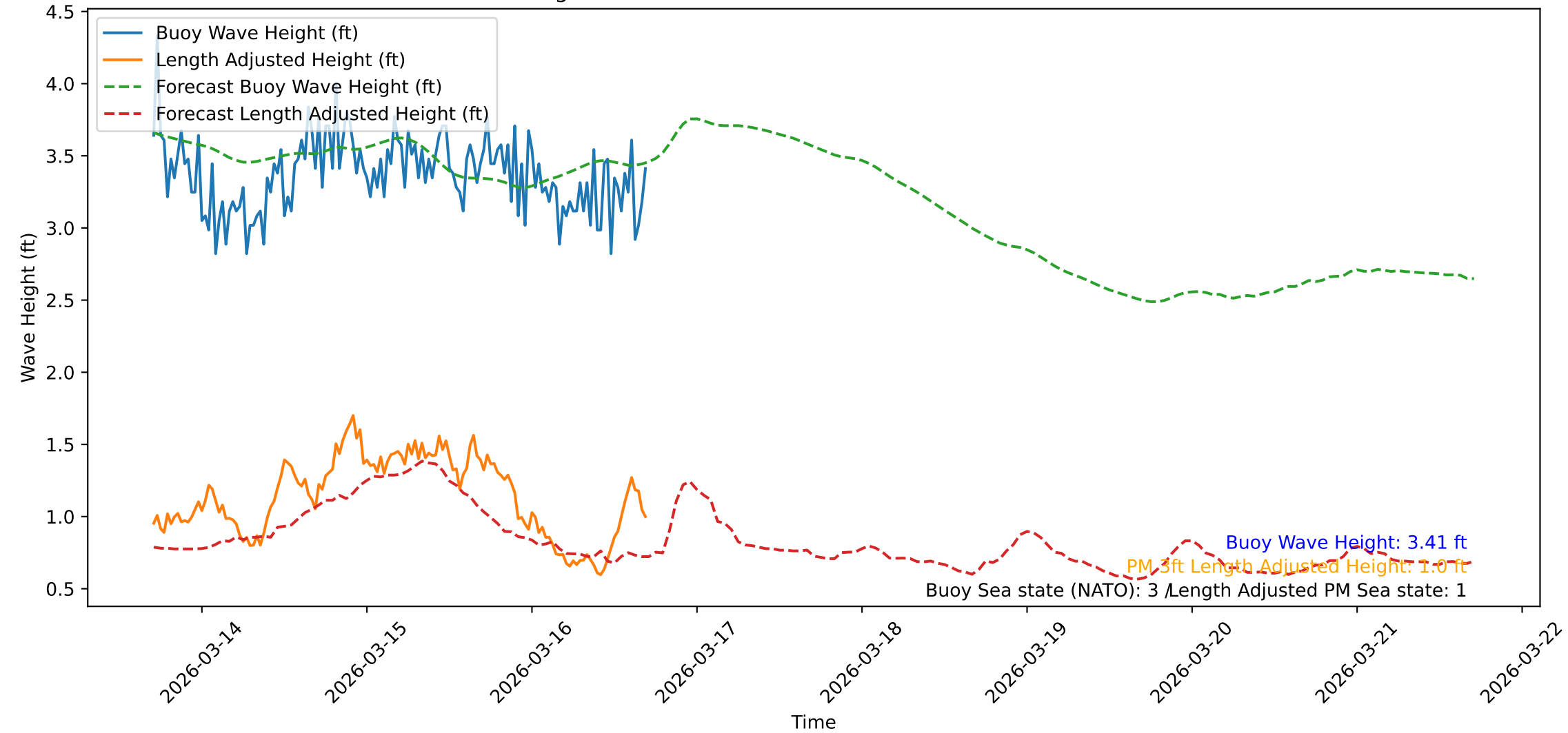
Wave Heights over Time for Green Beach at 2026-03-16 17:11:40
