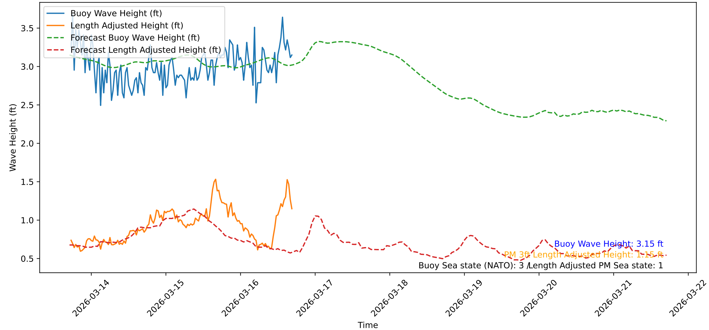
Wave Heights over Time for Red Beach at 2026-03-16 17:11:07
