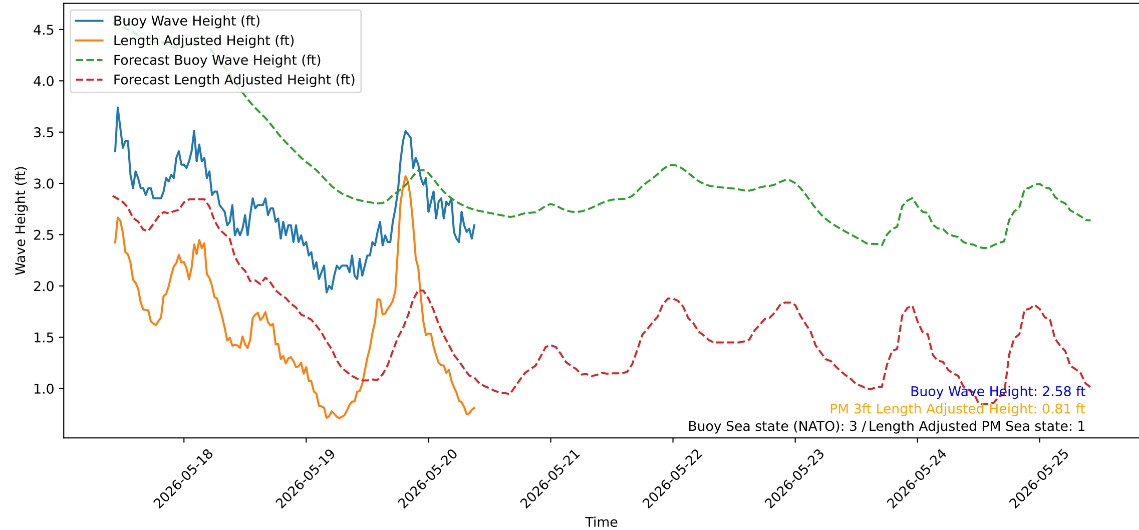
Wave Heights over Time for Red Beach at 2026-05-20 10:20:52
