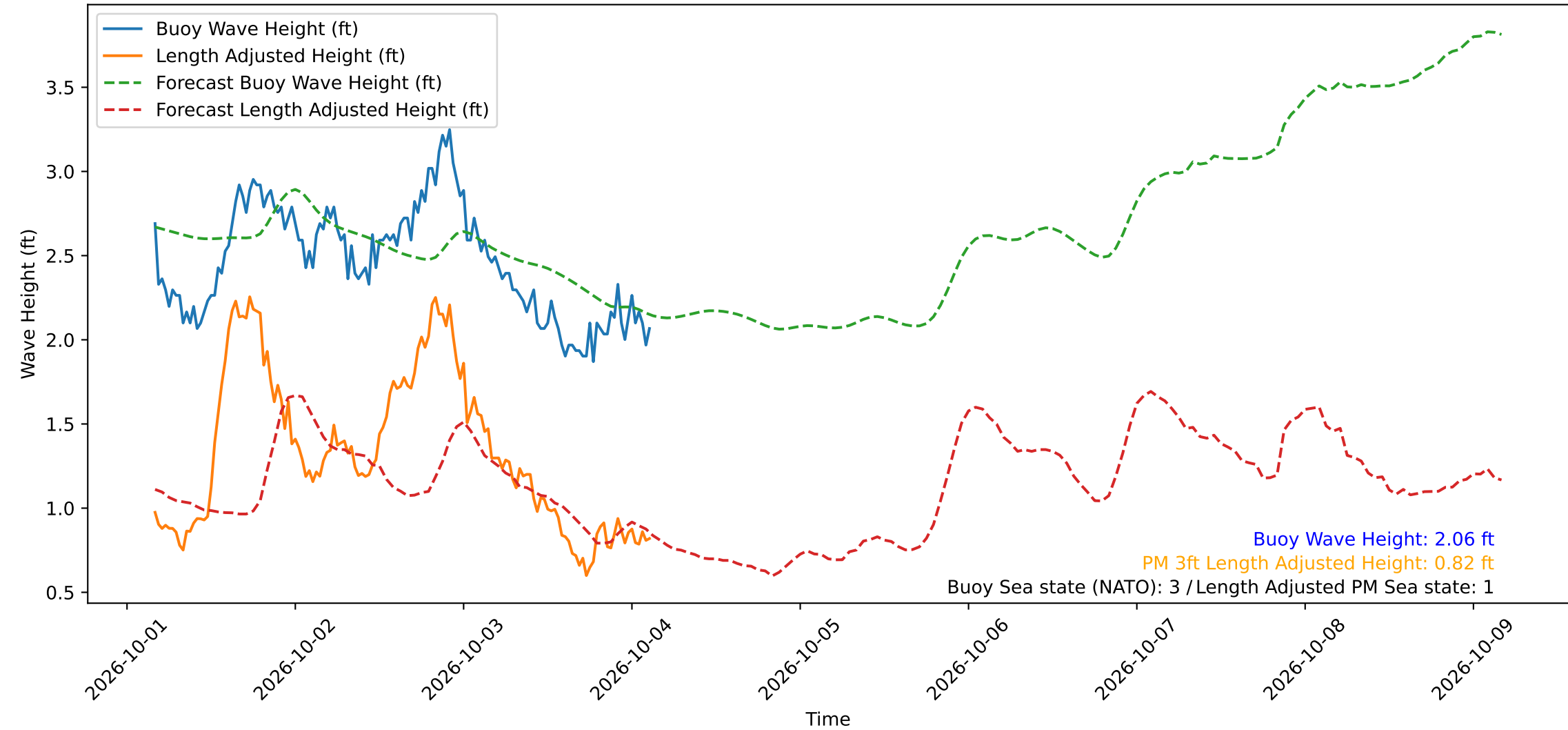
Wave Heights over Time for Red Beach at 2026-10-04 03:30:50
