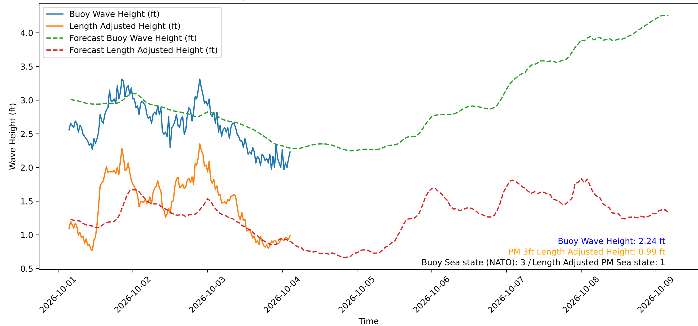
Wave Heights over Time for Oceanside Harbor at 2026-10-04 03:30:30
