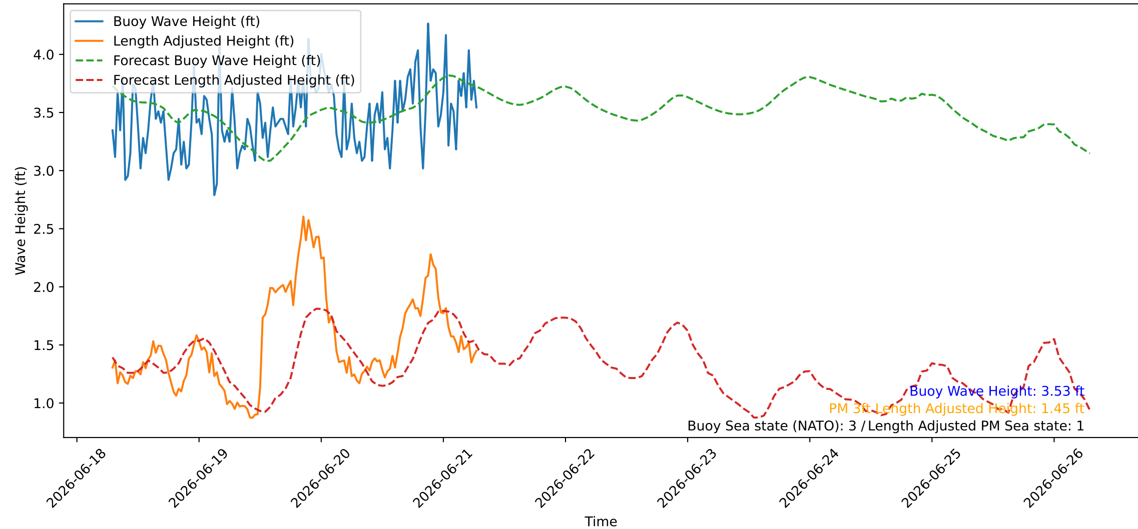
Wave Heights over Time for Oceanside Harbor at 2026-06-21 07:10:26
