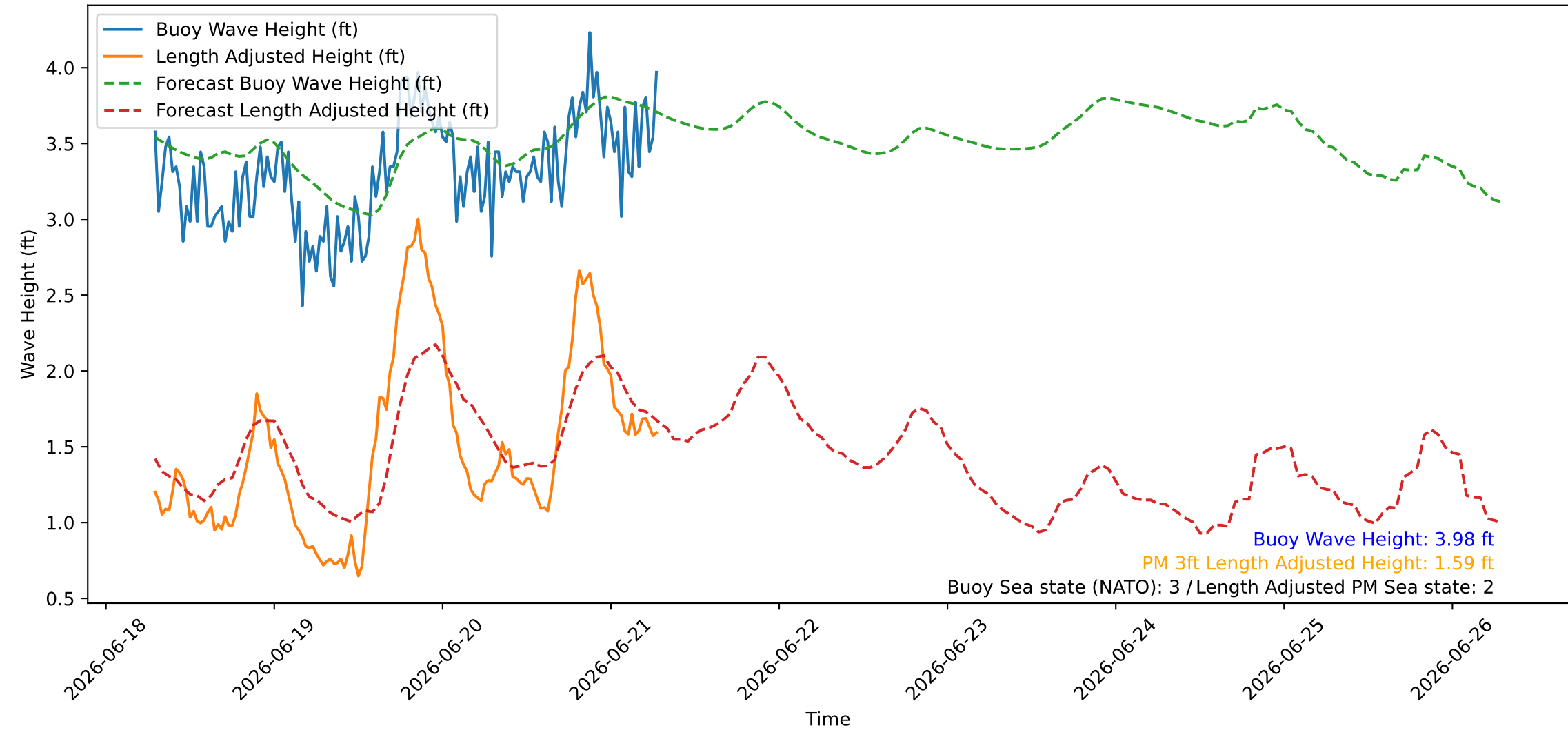
Wave Heights over Time for Green Beach at 2026-06-21 07:11:08
