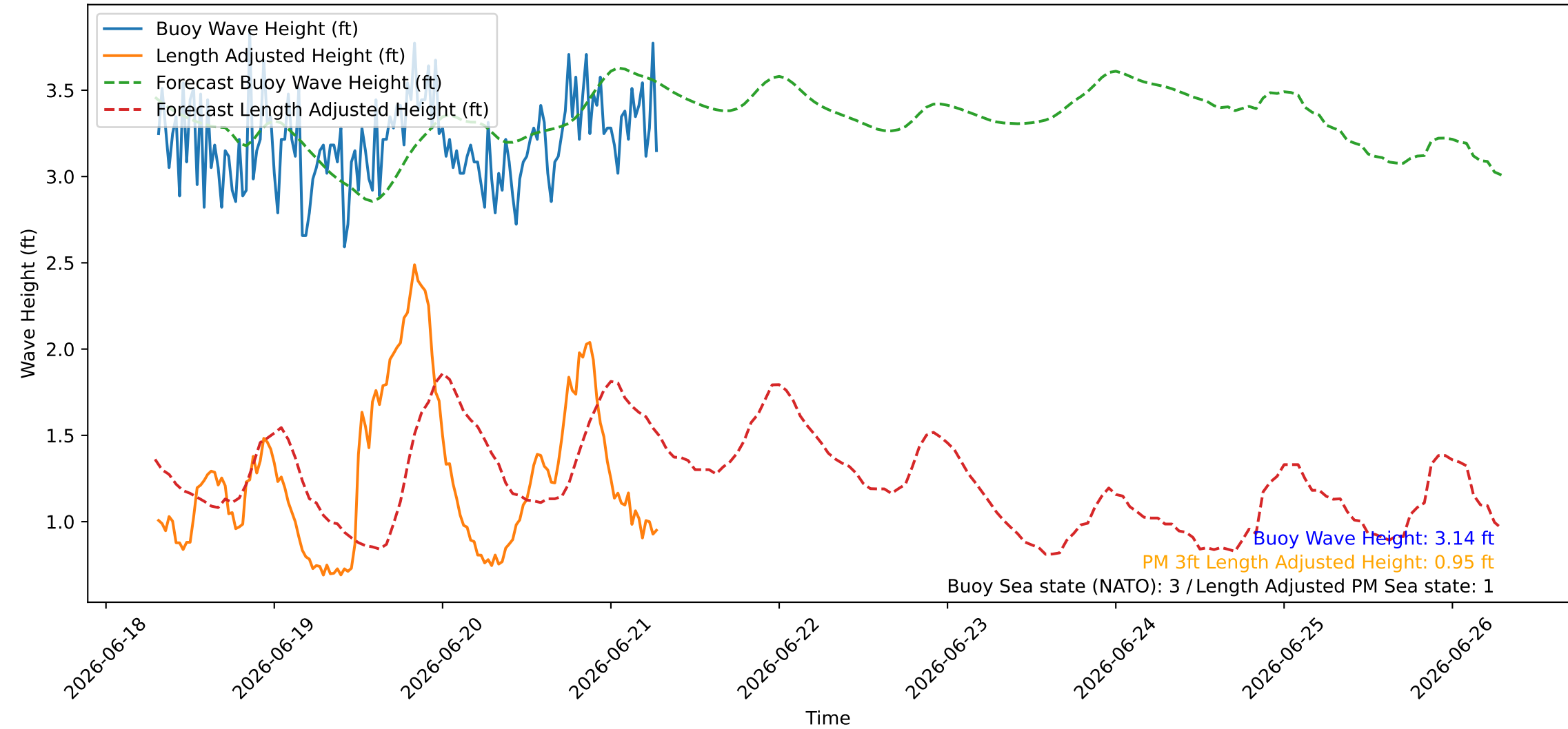
Wave Heights over Time for Red Beach at 2026-06-21 07:10:46
