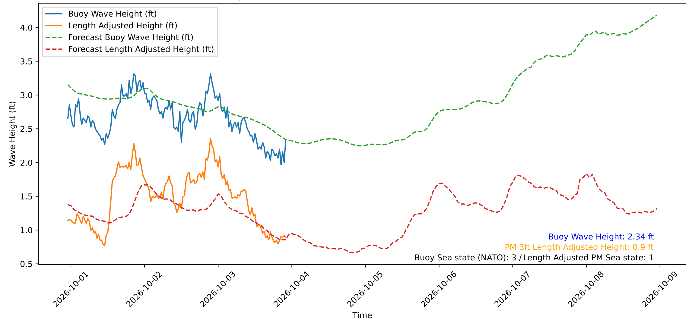
Wave Heights over Time for Oceanside Harbor at 2026-10-03 23:00:29
