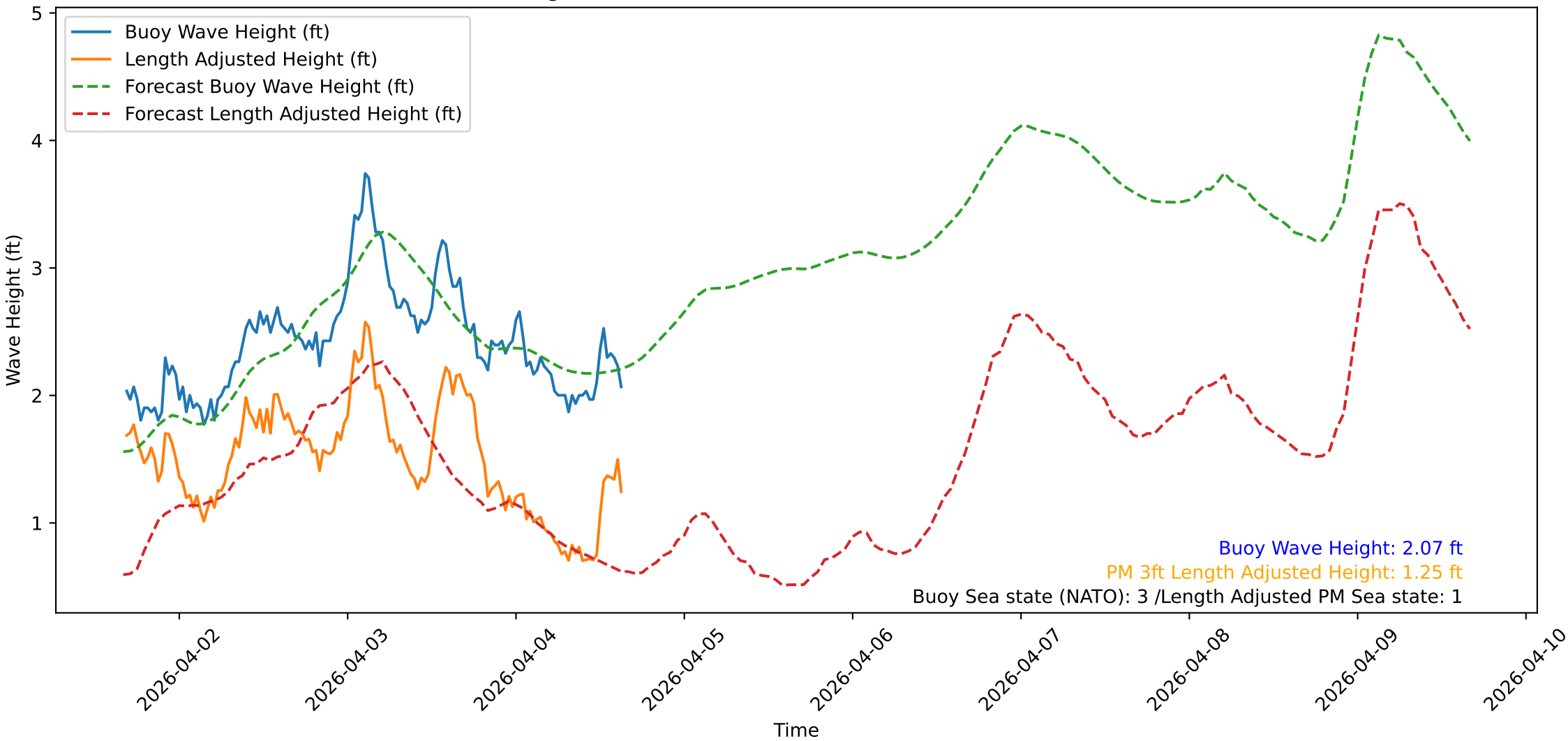
Wave Heights over Time for Red Beach at 2026-04-04 16:00:52
