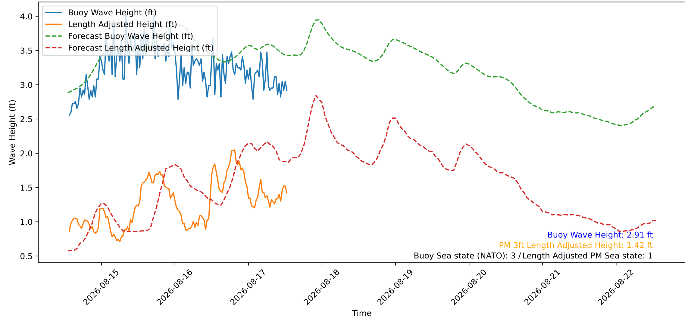
Wave Heights over Time for Red Beach at 2026-08-17 13:20:48
