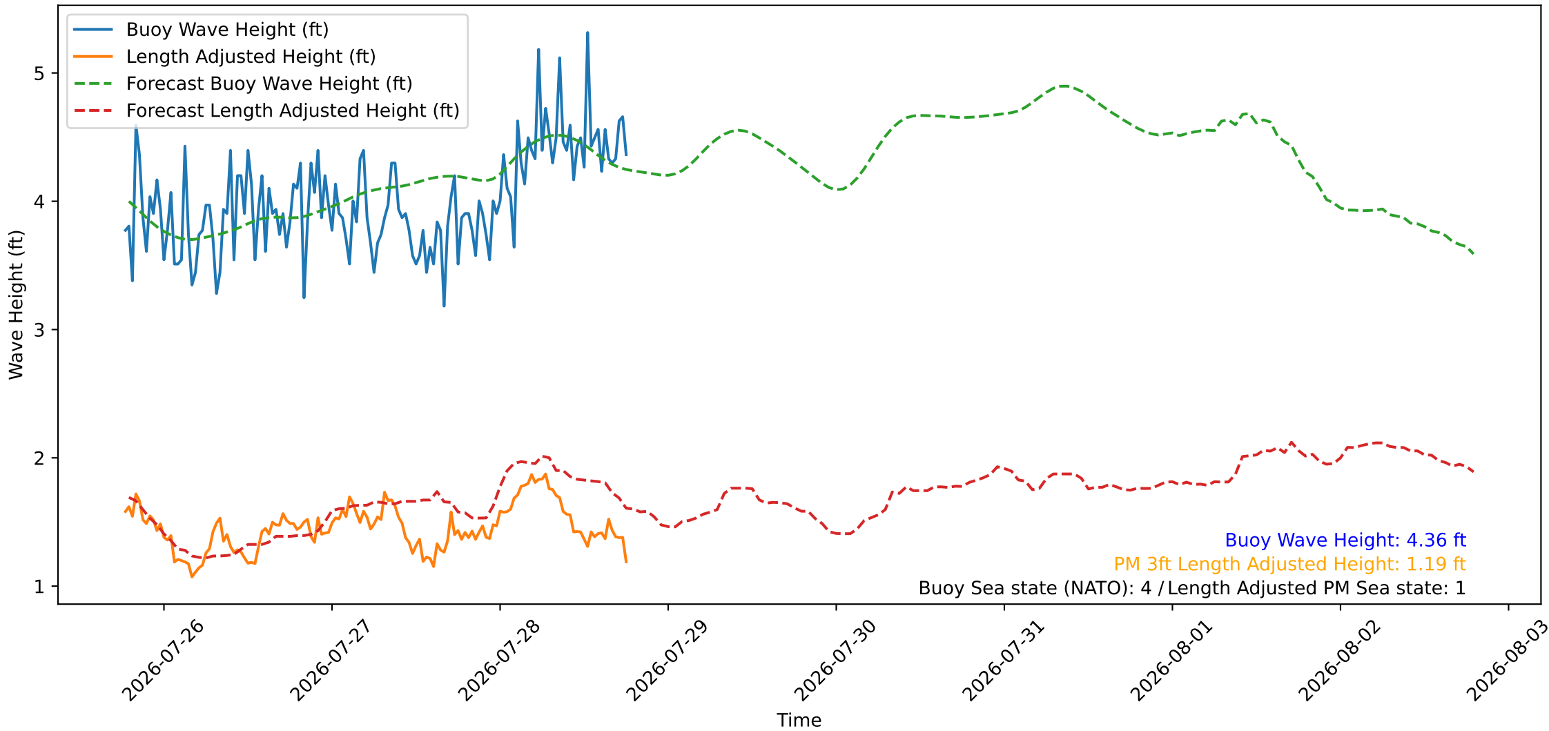
Wave Heights over Time for Oceanside Harbor at 2026-07-28 18:40:26
