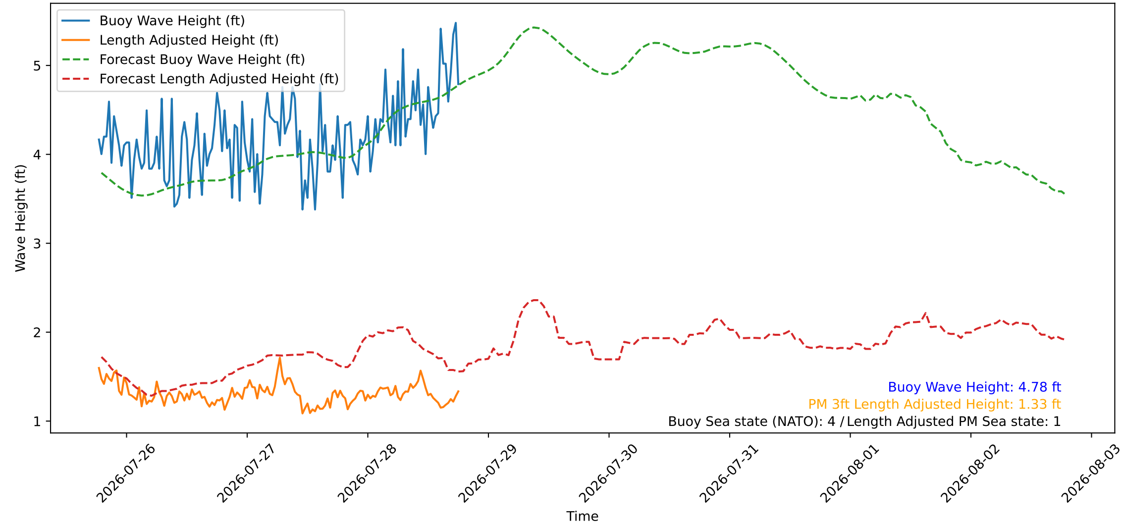
Wave Heights over Time for Green Beach at 2026-07-28 18:41:08
