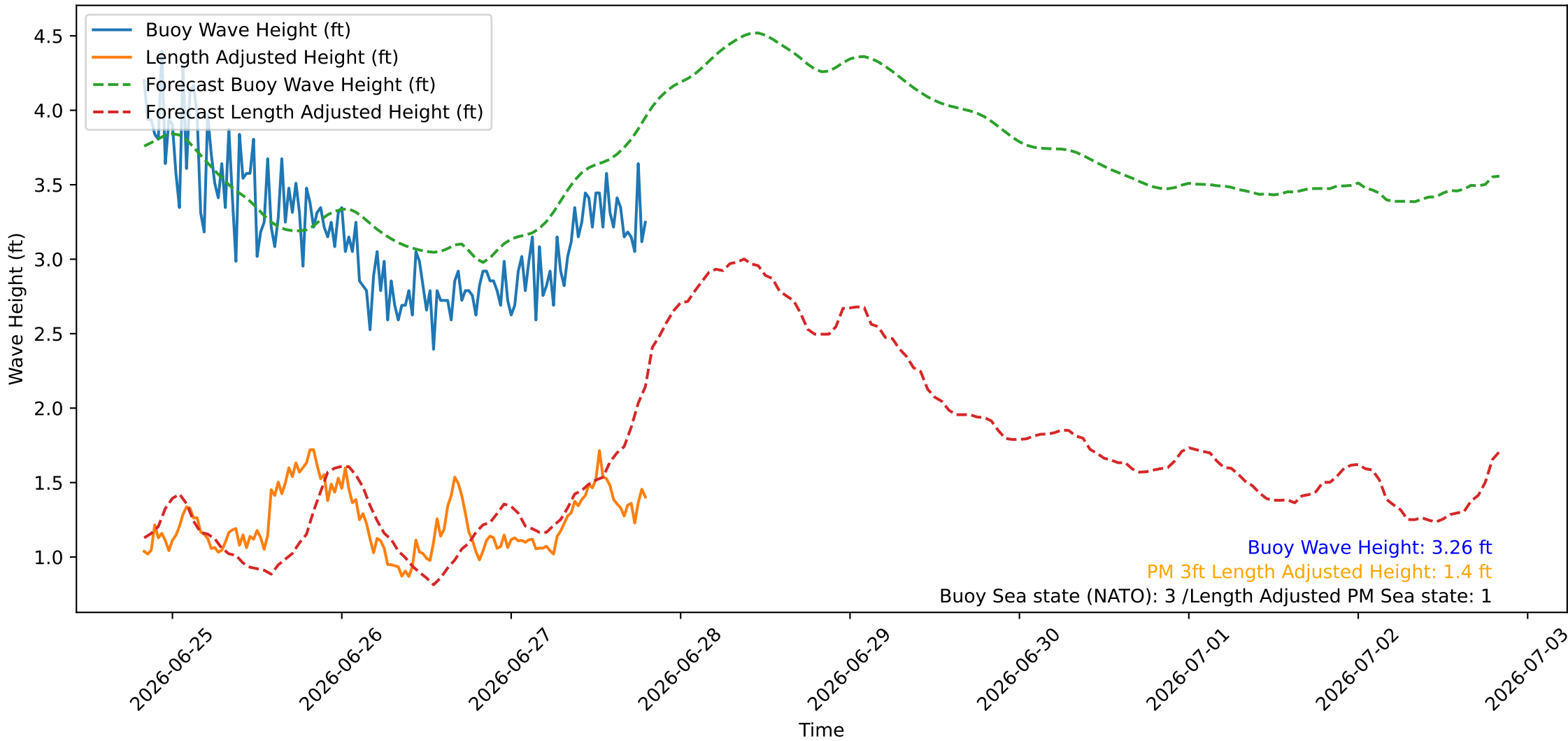
Wave Heights over Time for Oceanside Harbor at 2026-06-27 19:50:25
