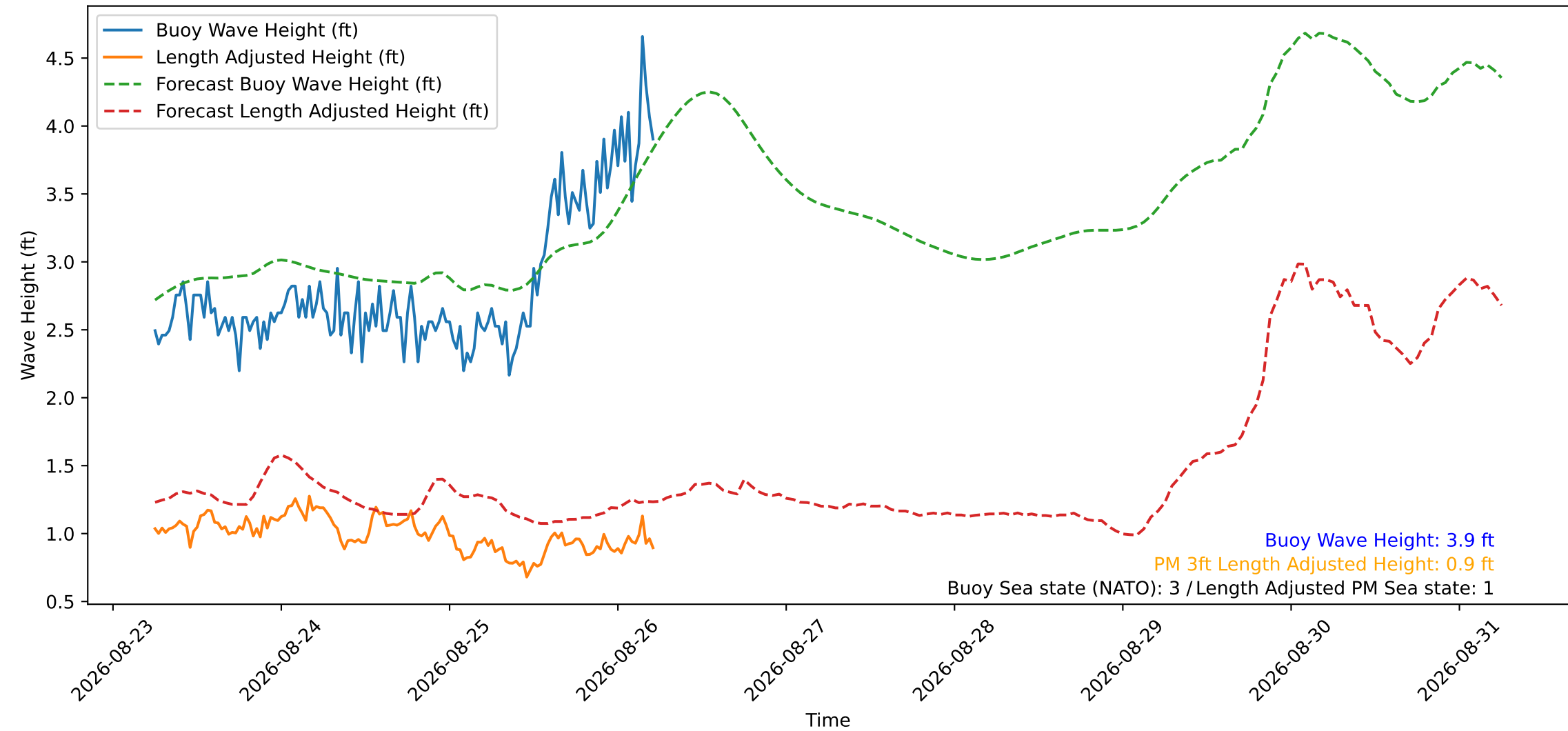
Wave Heights over Time for Red Beach at 2026-08-26 05:50:51
