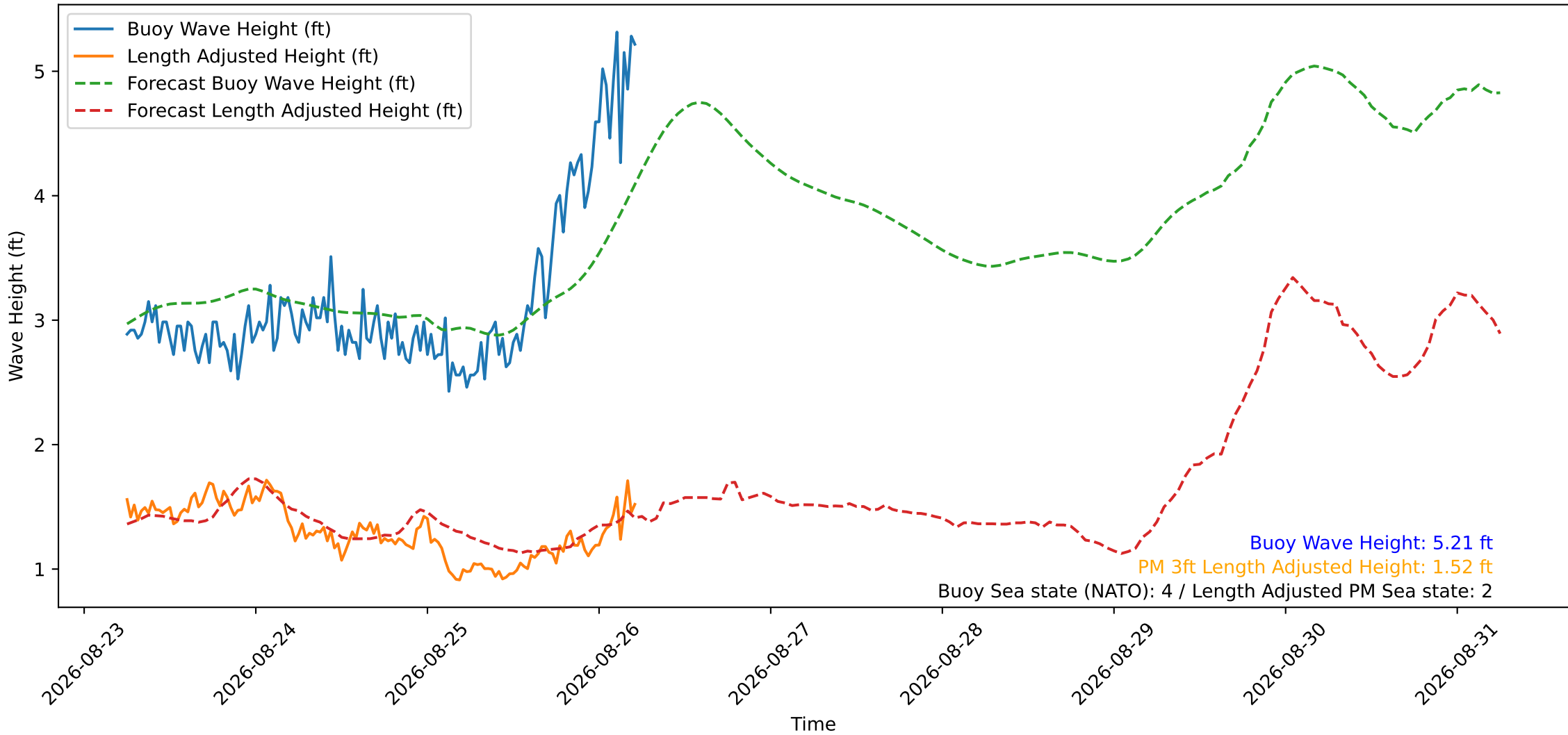
Wave Heights over Time for Oceanside Harbor at 2026-08-26 05:50:30
