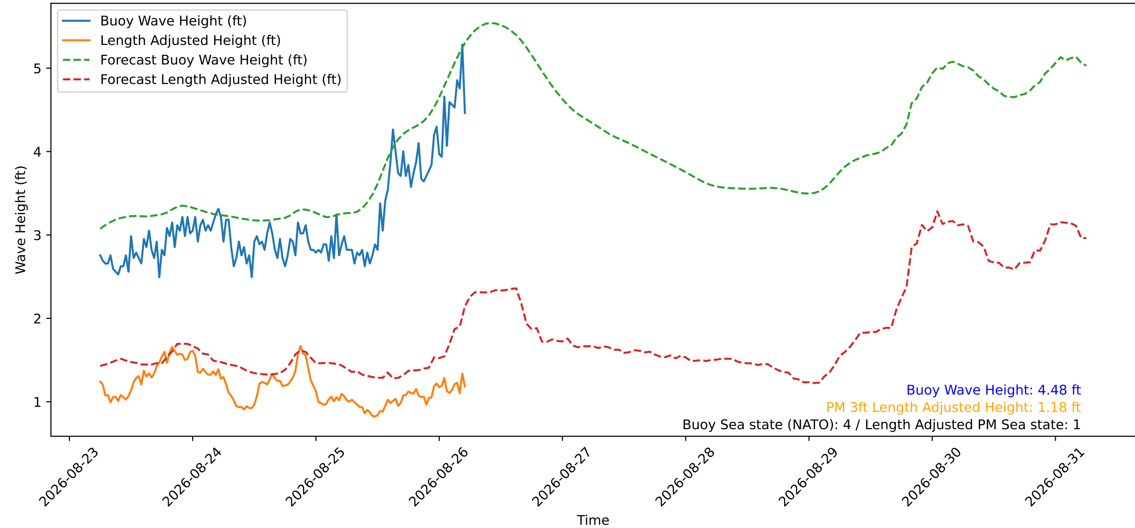
Wave Heights over Time for Green Beach at 2026-08-26 05:51:16
