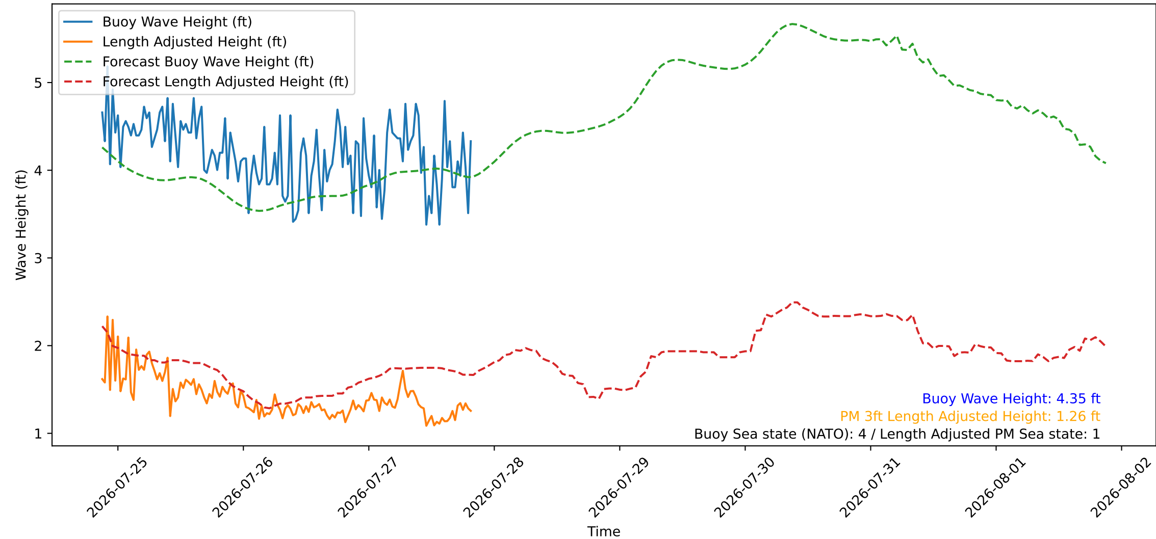
Wave Heights over Time for Green Beach at 2026-07-27 20:51:10
