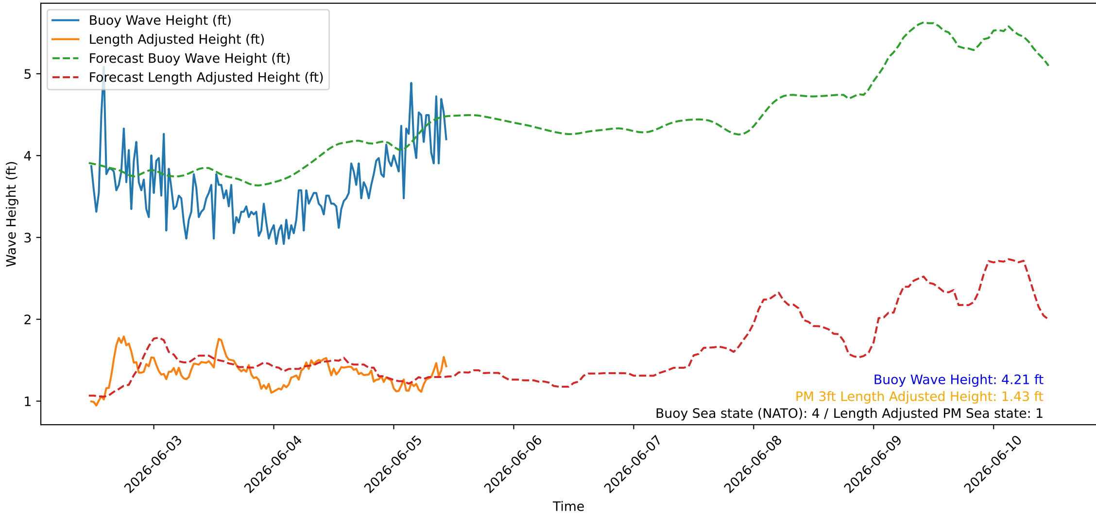
Wave Heights over Time for Oceanside Harbor at 2026-06-05 11:20:26
