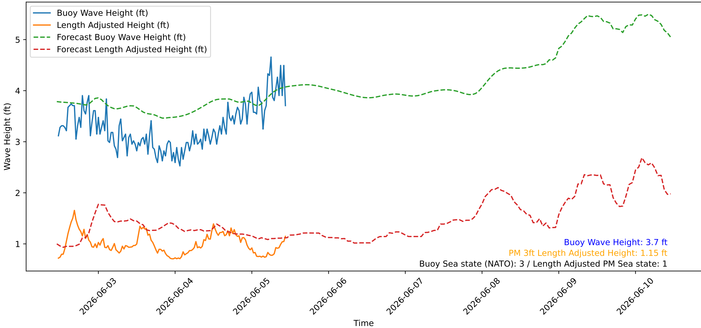
Wave Heights over Time for Red Beach at 2026-06-05 11:20:47
