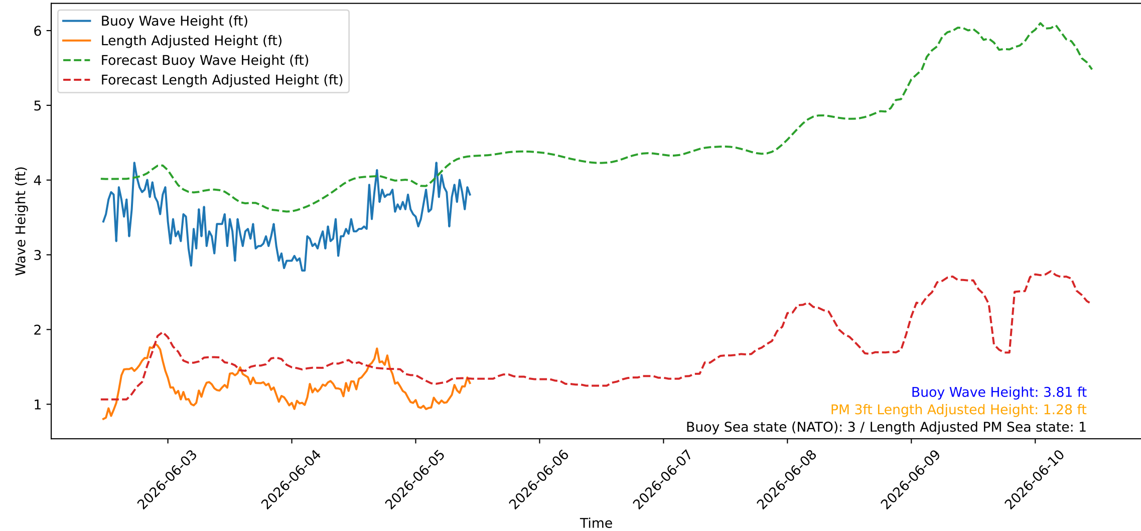
Wave Heights over Time for Green Beach at 2026-06-05 11:21:09
