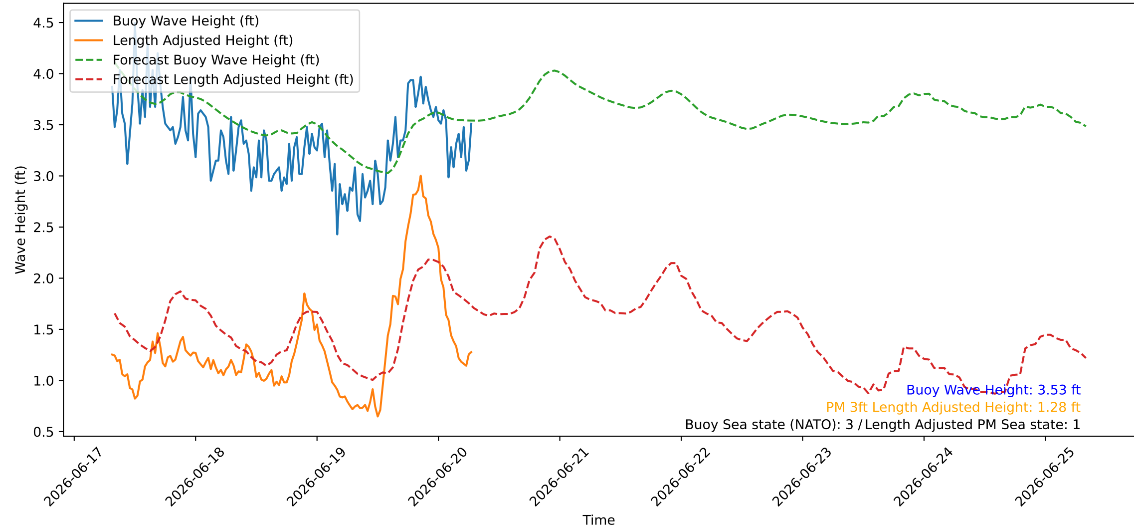
Wave Heights over Time for Green Beach at 2026-06-20 07:31:07
