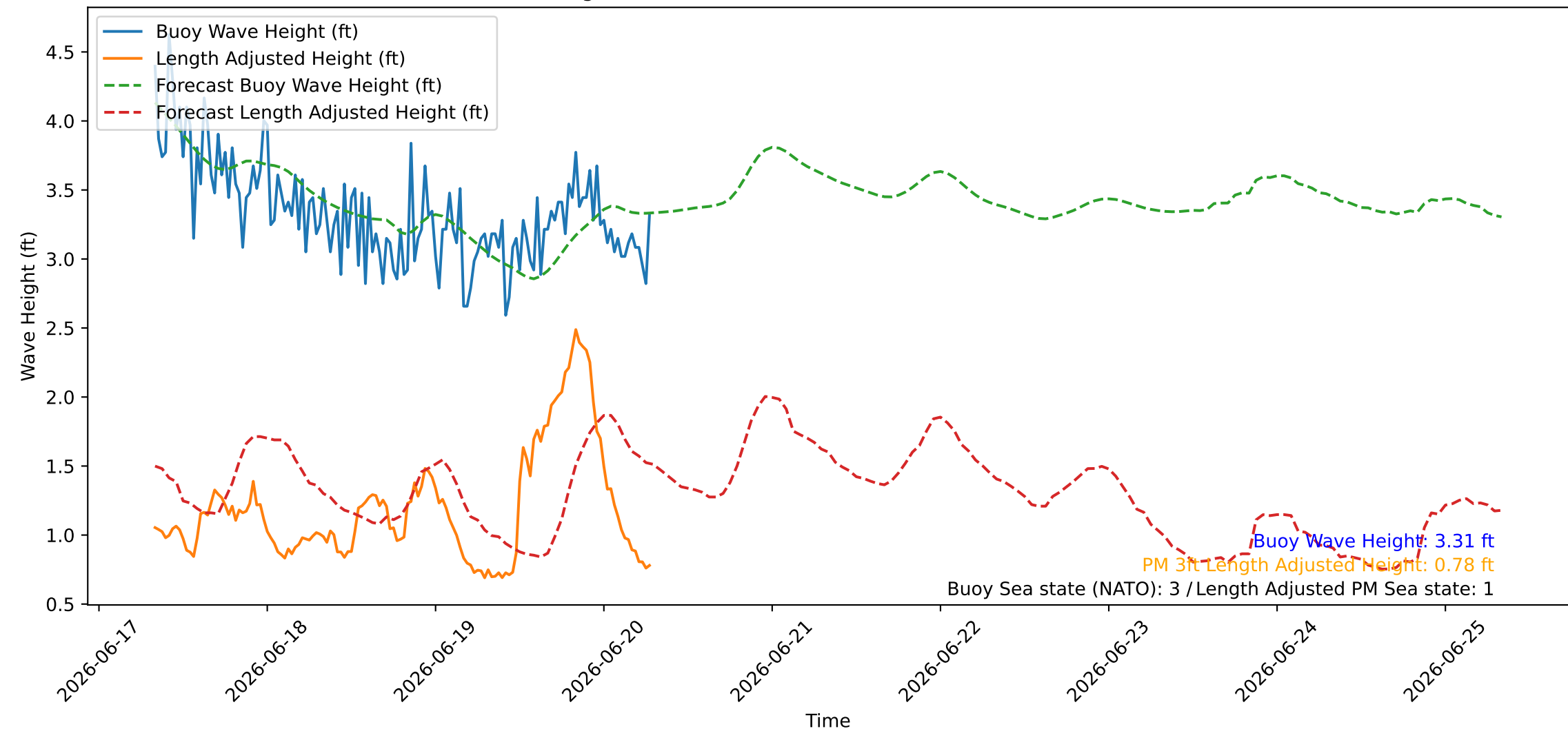
Wave Heights over Time for Red Beach at 2026-06-20 07:30:44
