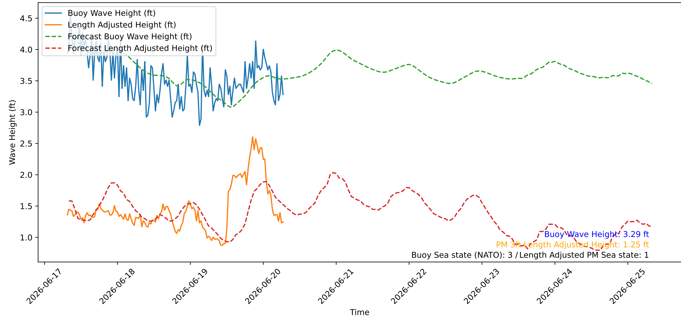
Wave Heights over Time for Oceanside Harbor at 2026-06-20 07:30:25
