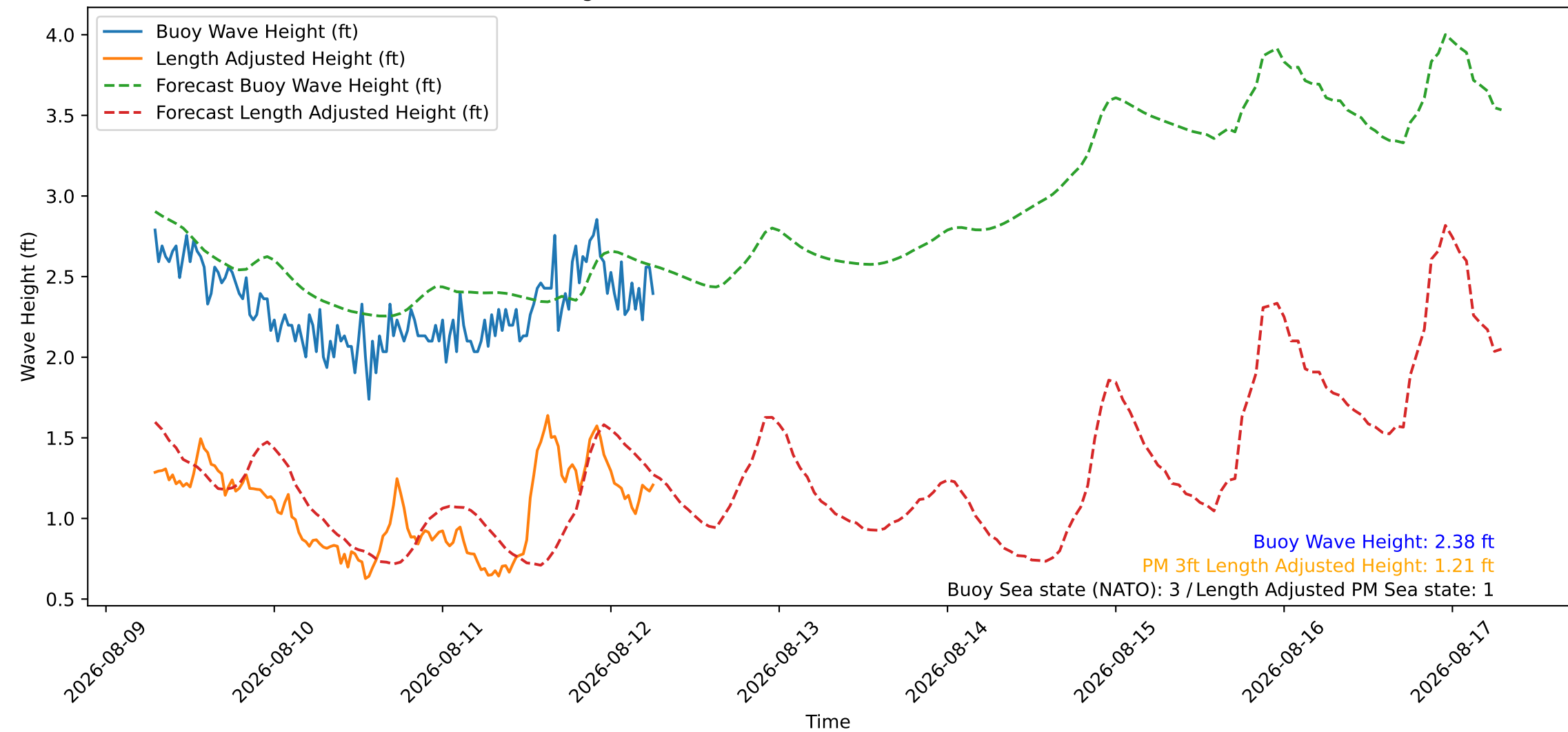
Wave Heights over Time for Red Beach at 2026-08-12 06:40:47
