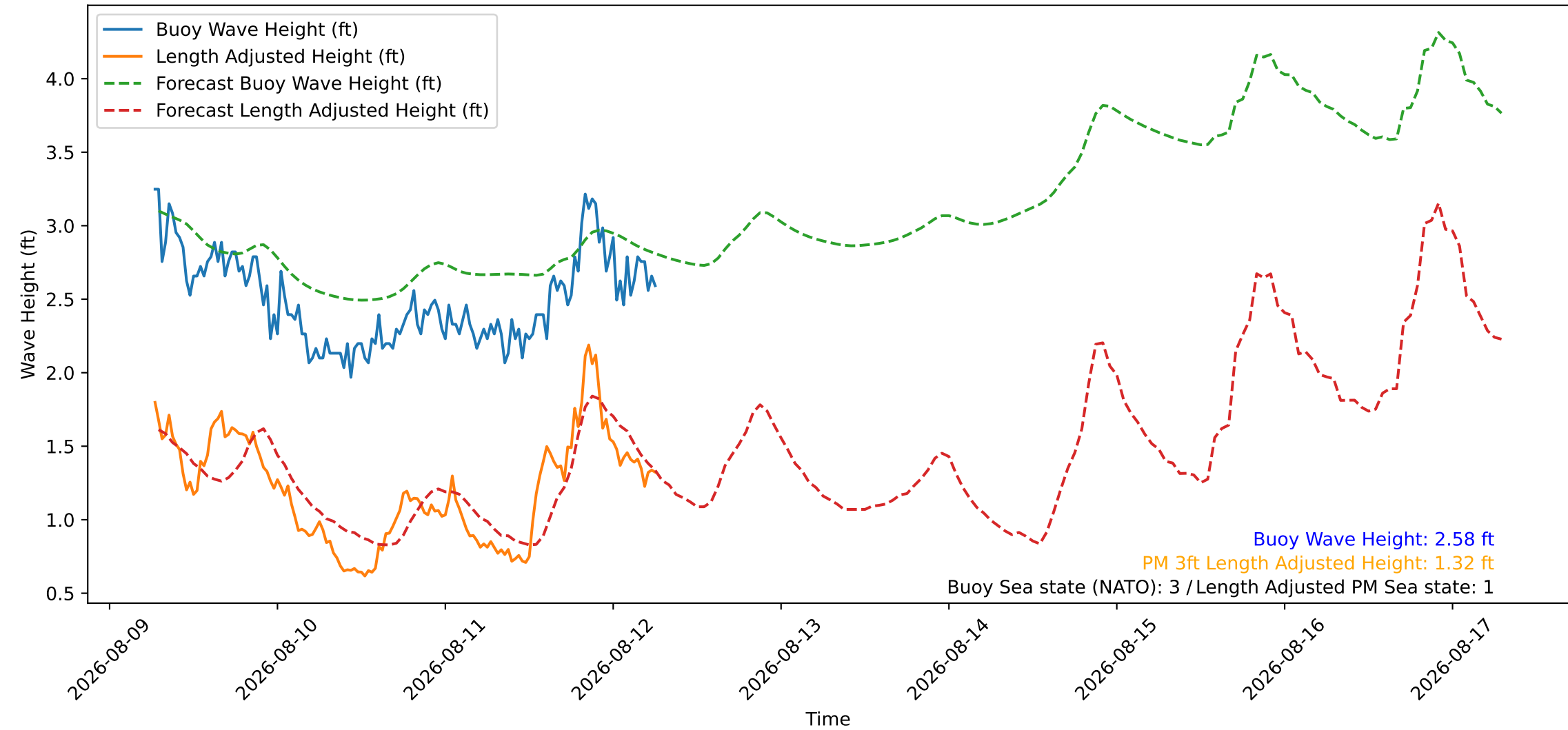
Wave Heights over Time for Green Beach at 2026-08-12 06:41:09
