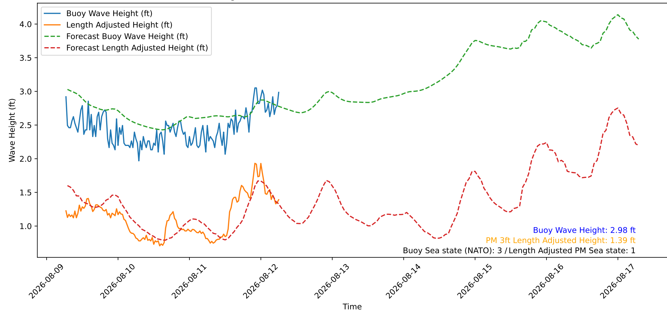
Wave Heights over Time for Oceanside Harbor at 2026-08-12 06:40:27
