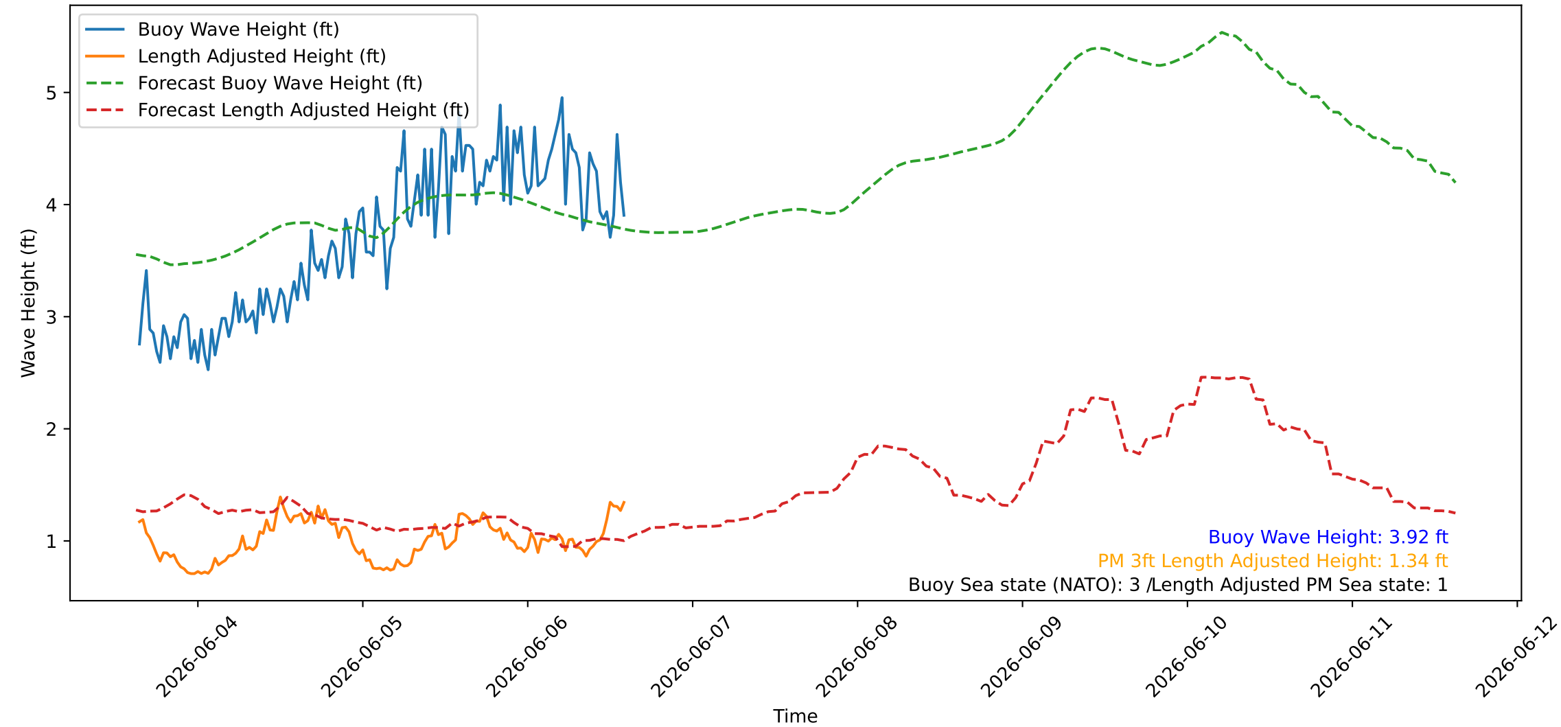
Wave Heights over Time for Red Beach at 2026-06-06 15:00:45
