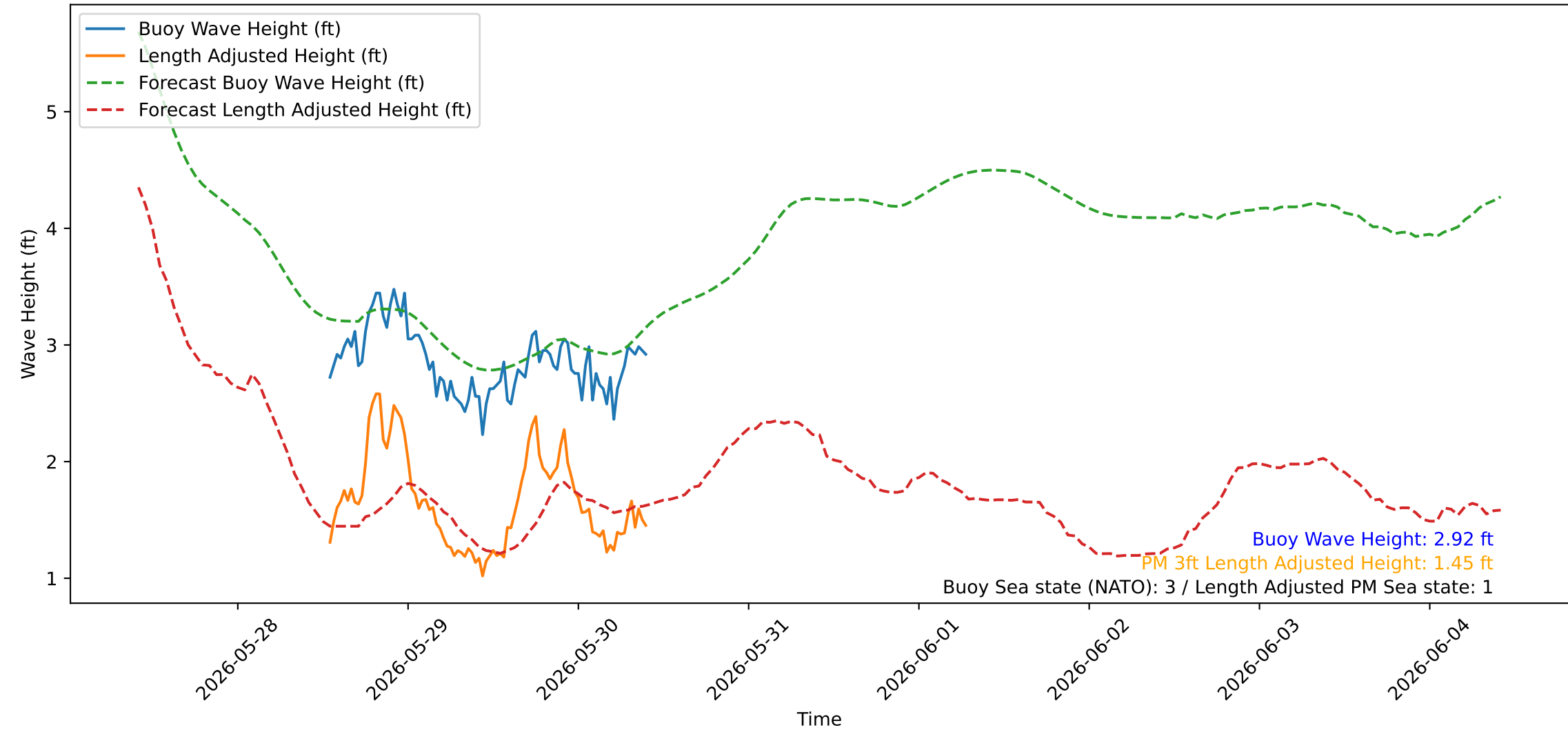
Wave Heights over Time for Oceanside Harbor at 2026-05-30 10:10:23
