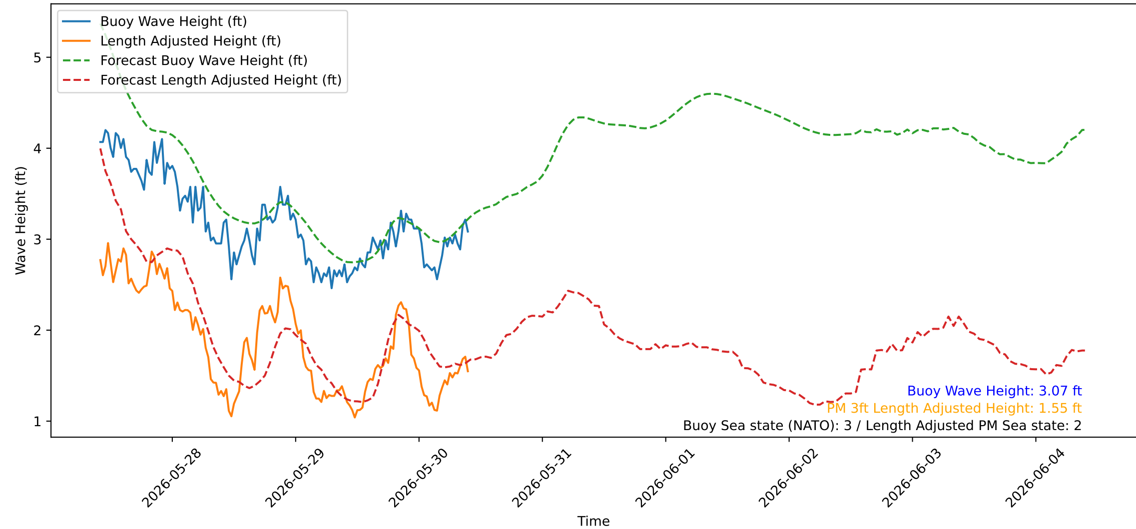
Wave Heights over Time for Green Beach at 2026-05-30 10:11:05
