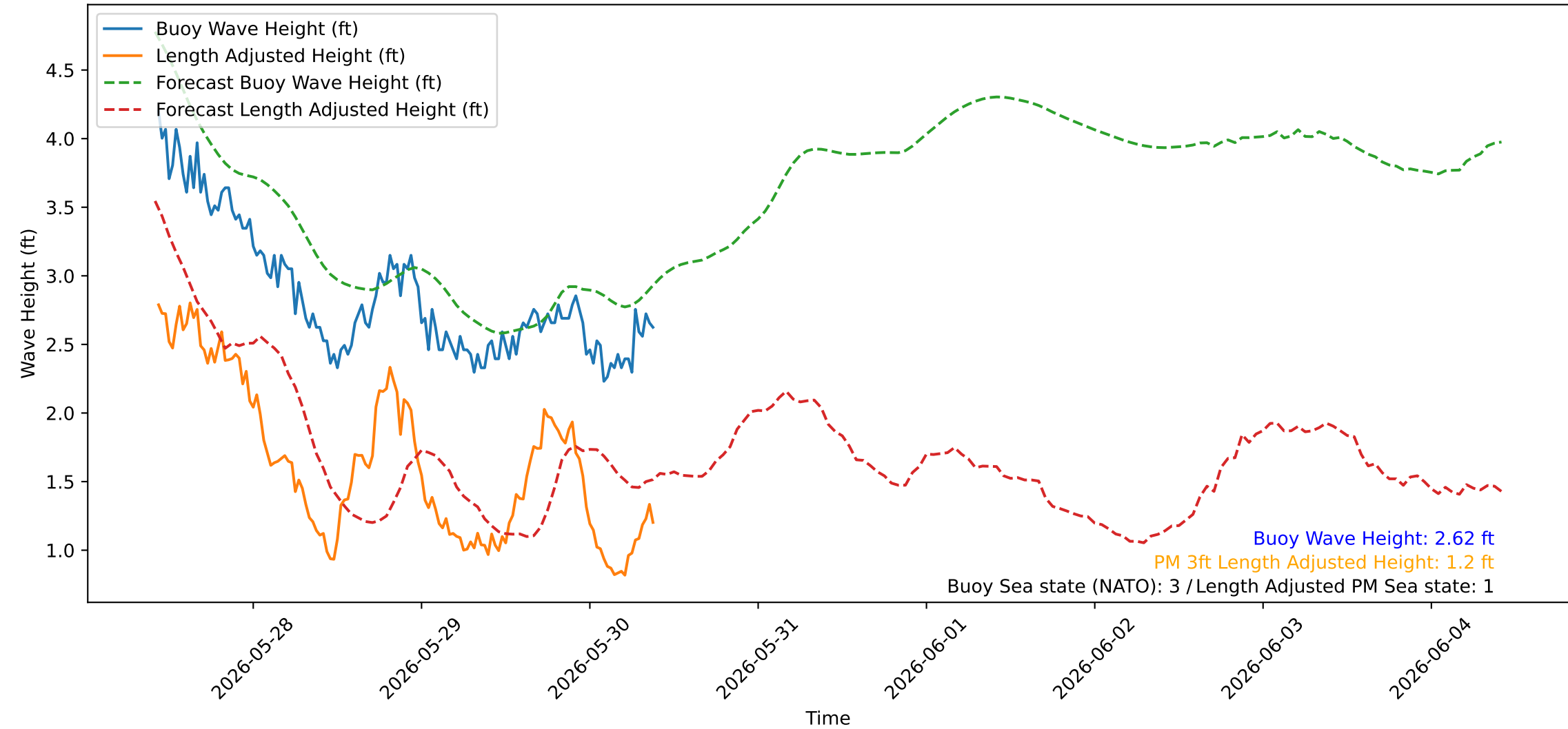
Wave Heights over Time for Red Beach at 2026-05-30 10:10:42
