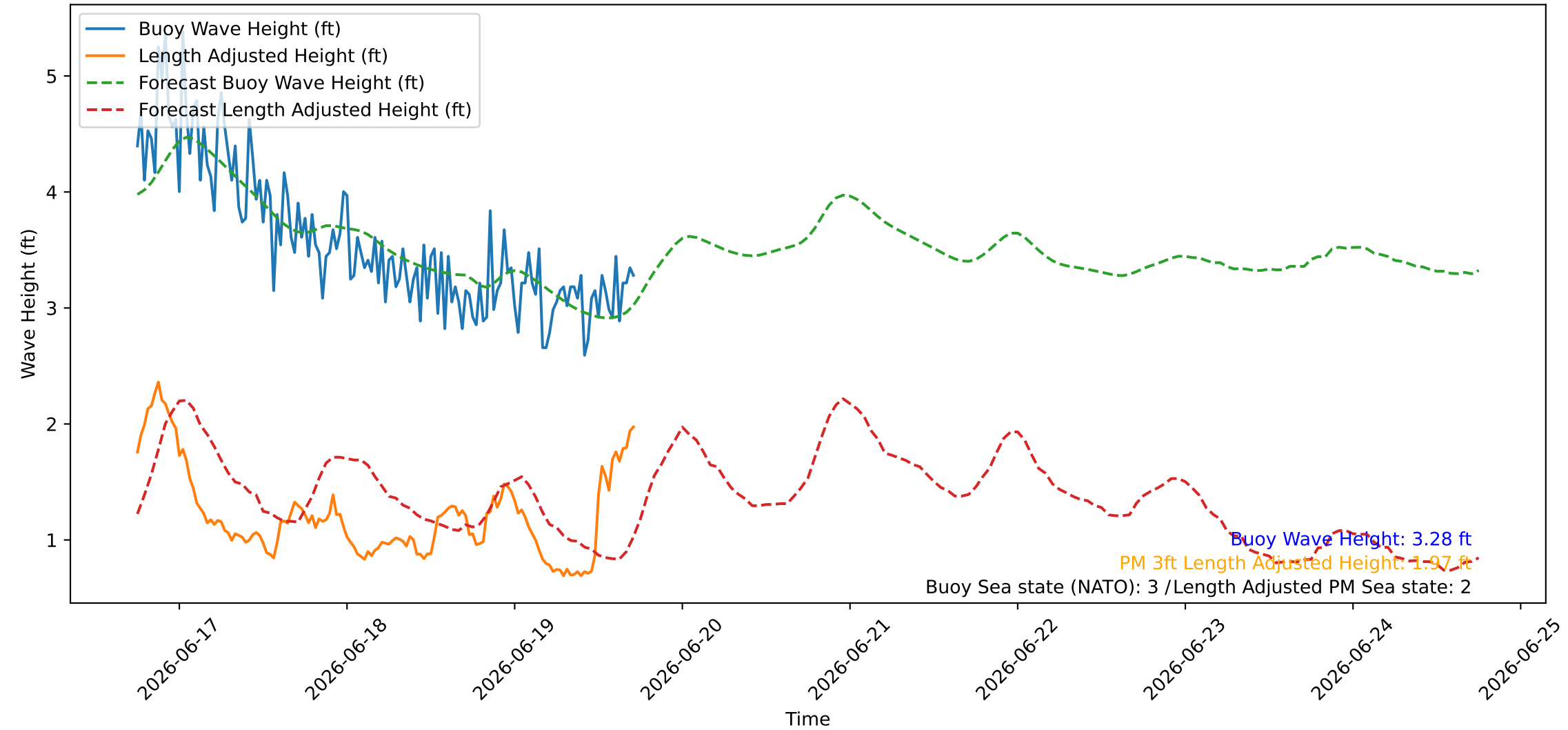
Wave Heights over Time for Red Beach at 2026-06-19 17:40:45
