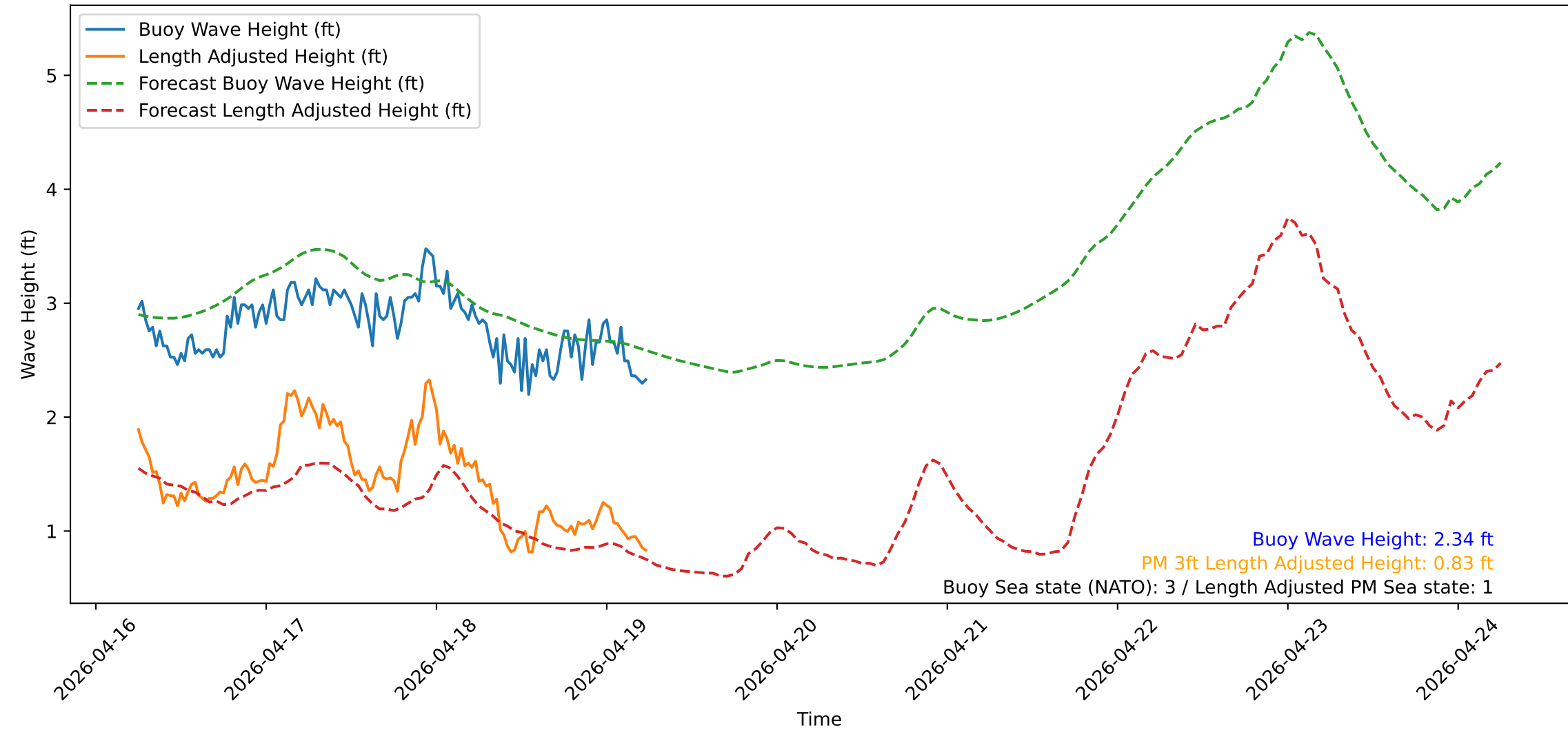
Wave Heights over Time for Green Beach at 2026-04-19 06:11:12
