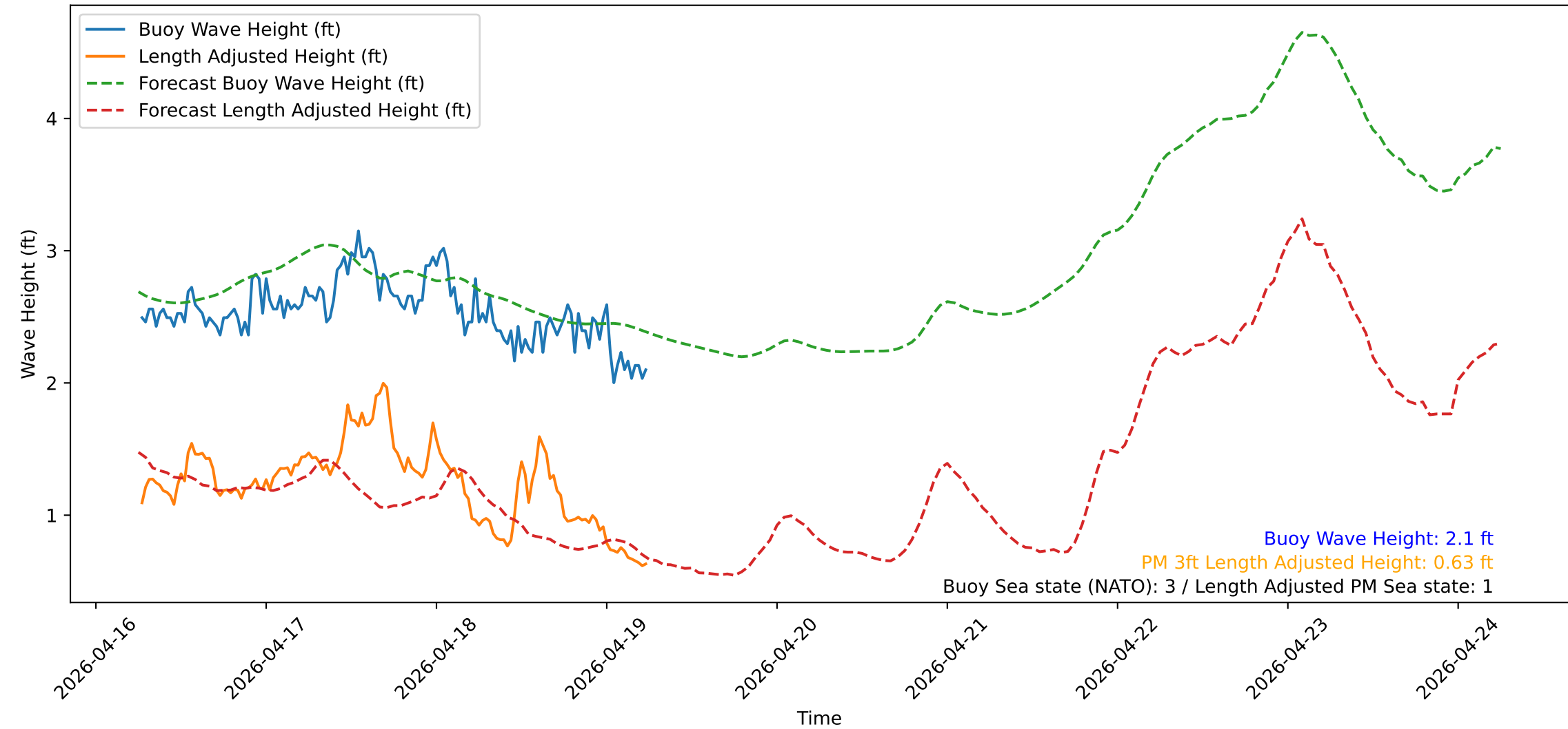
Wave Heights over Time for Red Beach at 2026-04-19 06:10:50
