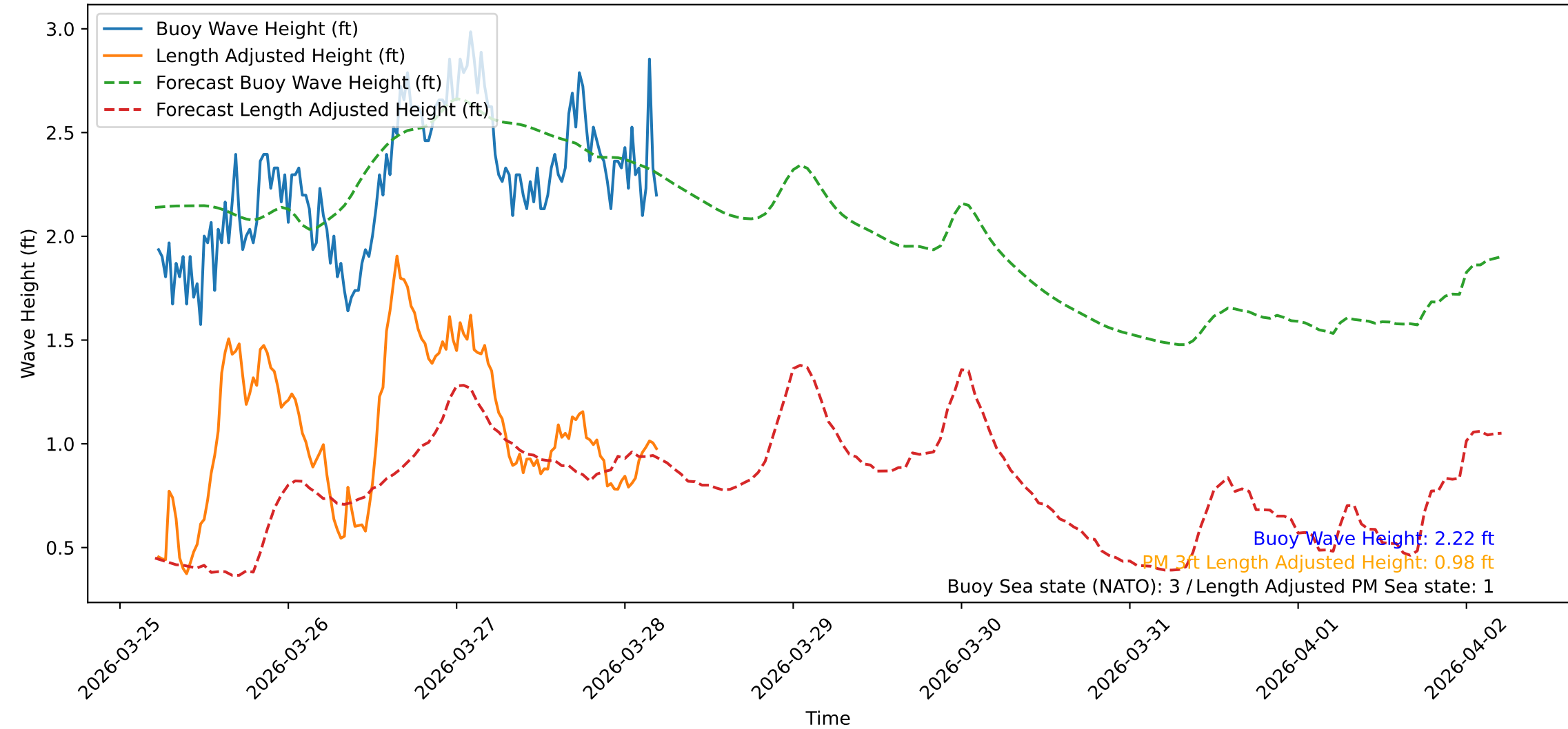
Wave Heights over Time for Red Beach at 2026-03-28 05:10:47
