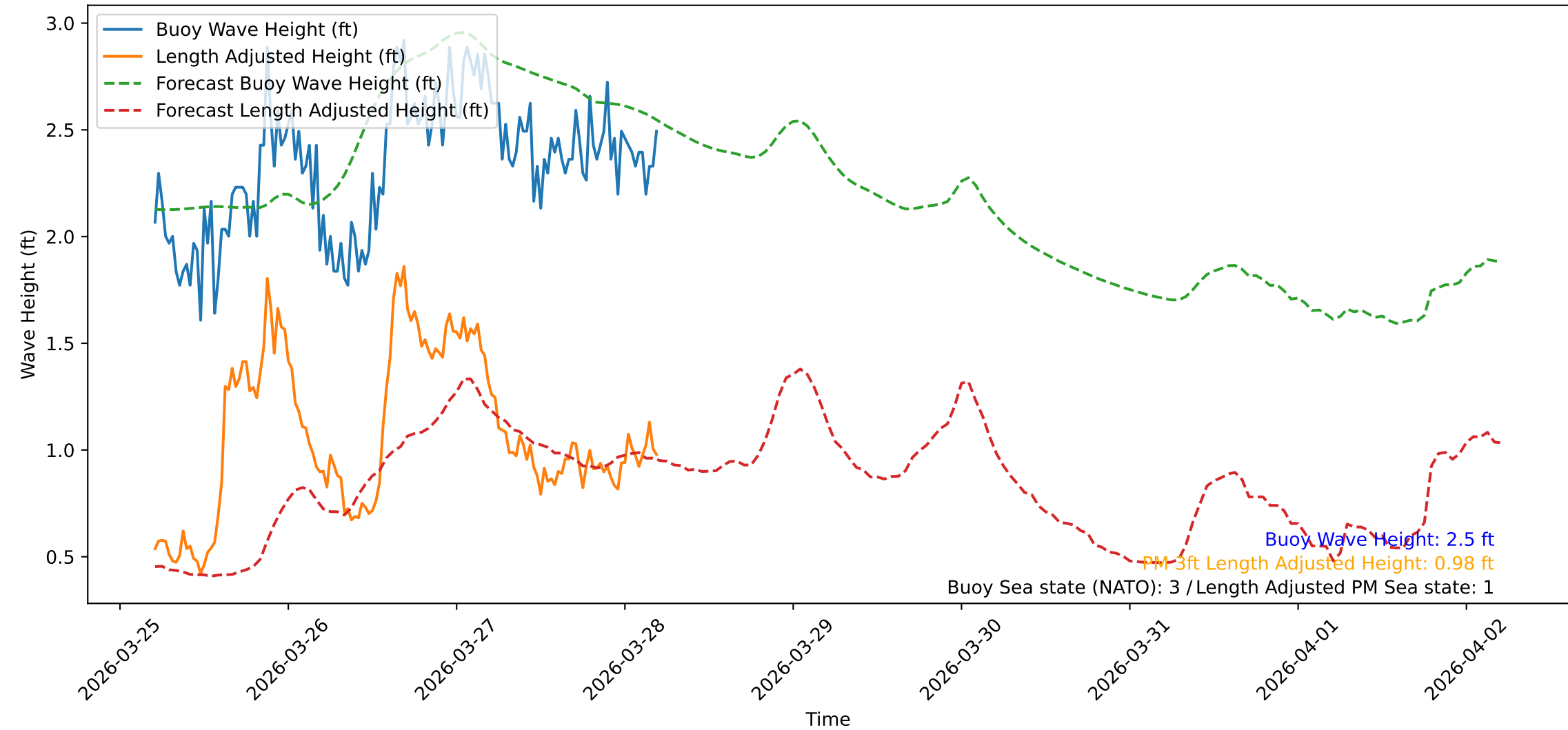
Wave Heights over Time for Oceanside Harbor at 2026-03-28 05:10:31
