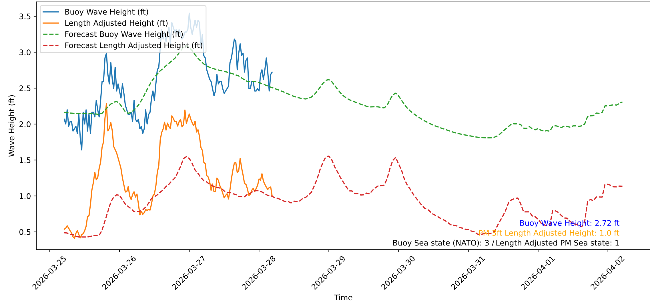
Wave Heights over Time for Green Beach at 2026-03-28 05:11:09
