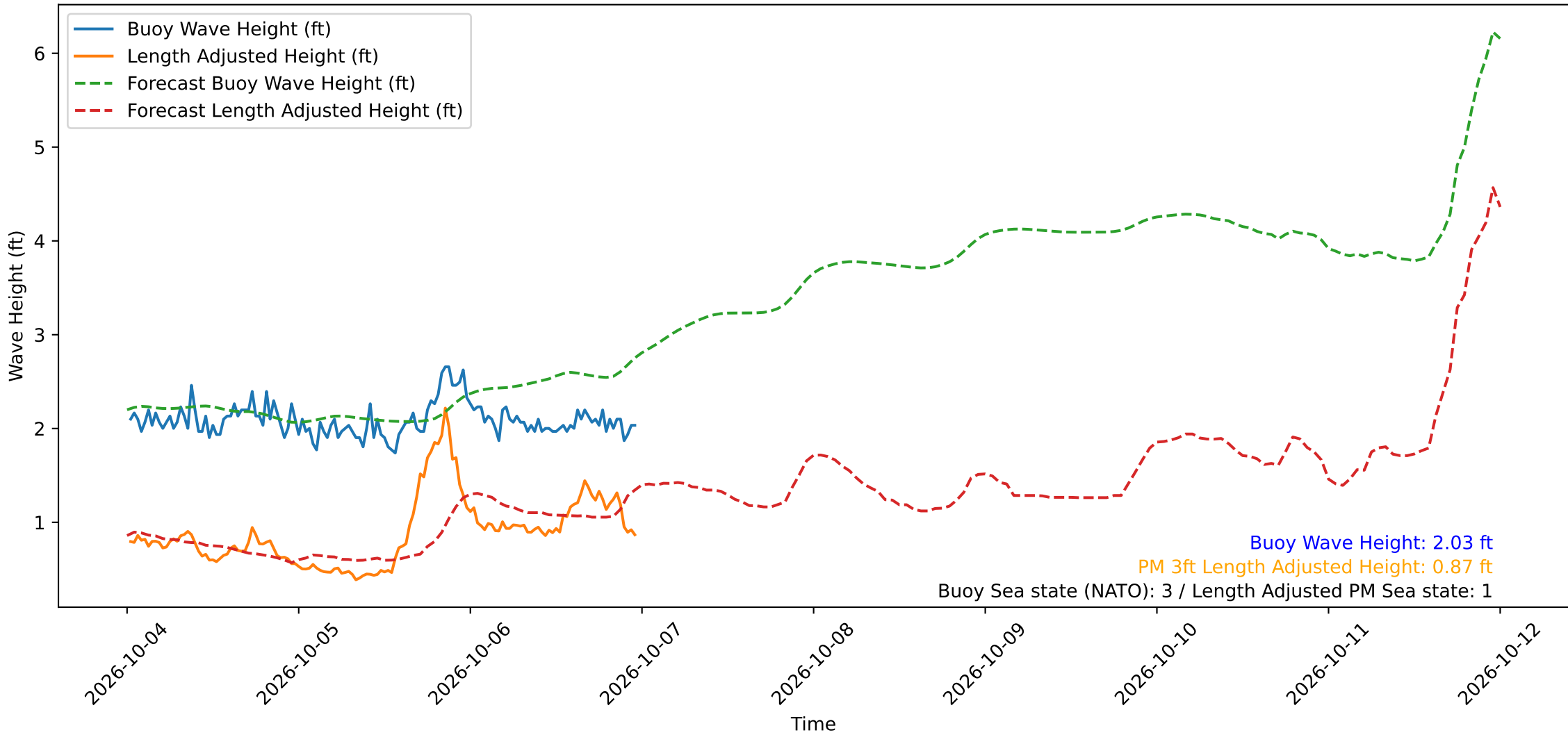
Wave Heights over Time for Red Beach at 2026-10-07 00:00:49
