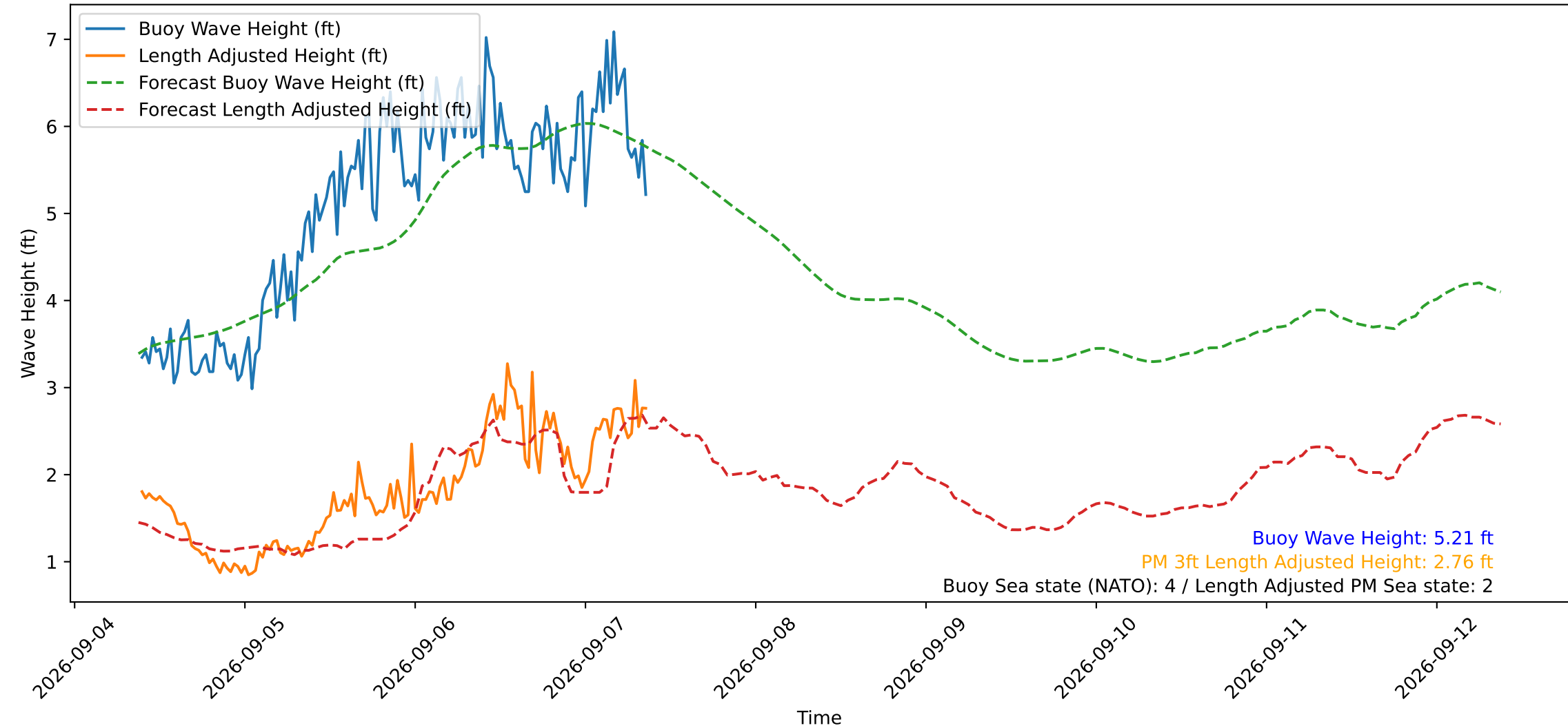
Wave Heights over Time for Oceanside Harbor at 2026-09-07 09:20:30
