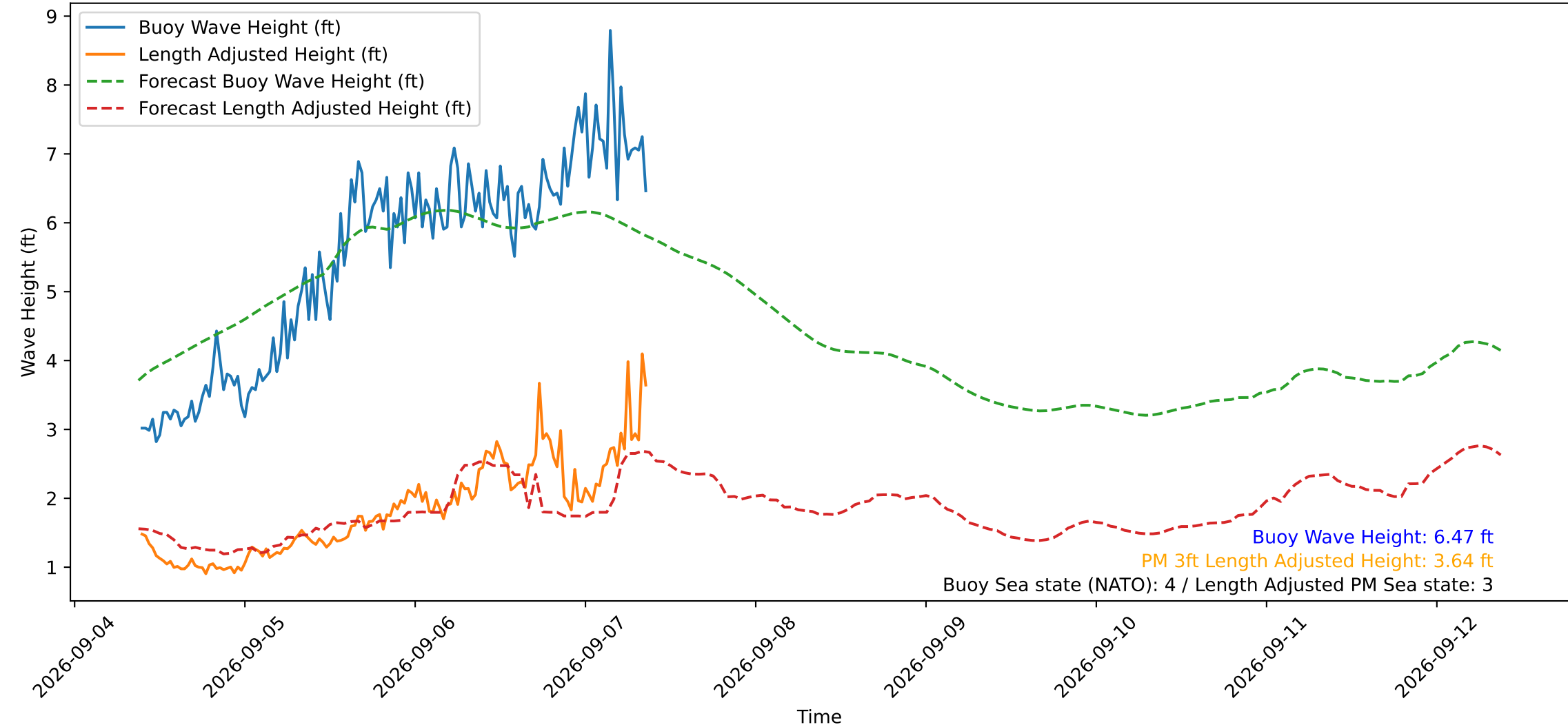
Wave Heights over Time for Green Beach at 2026-09-07 09:21:15
