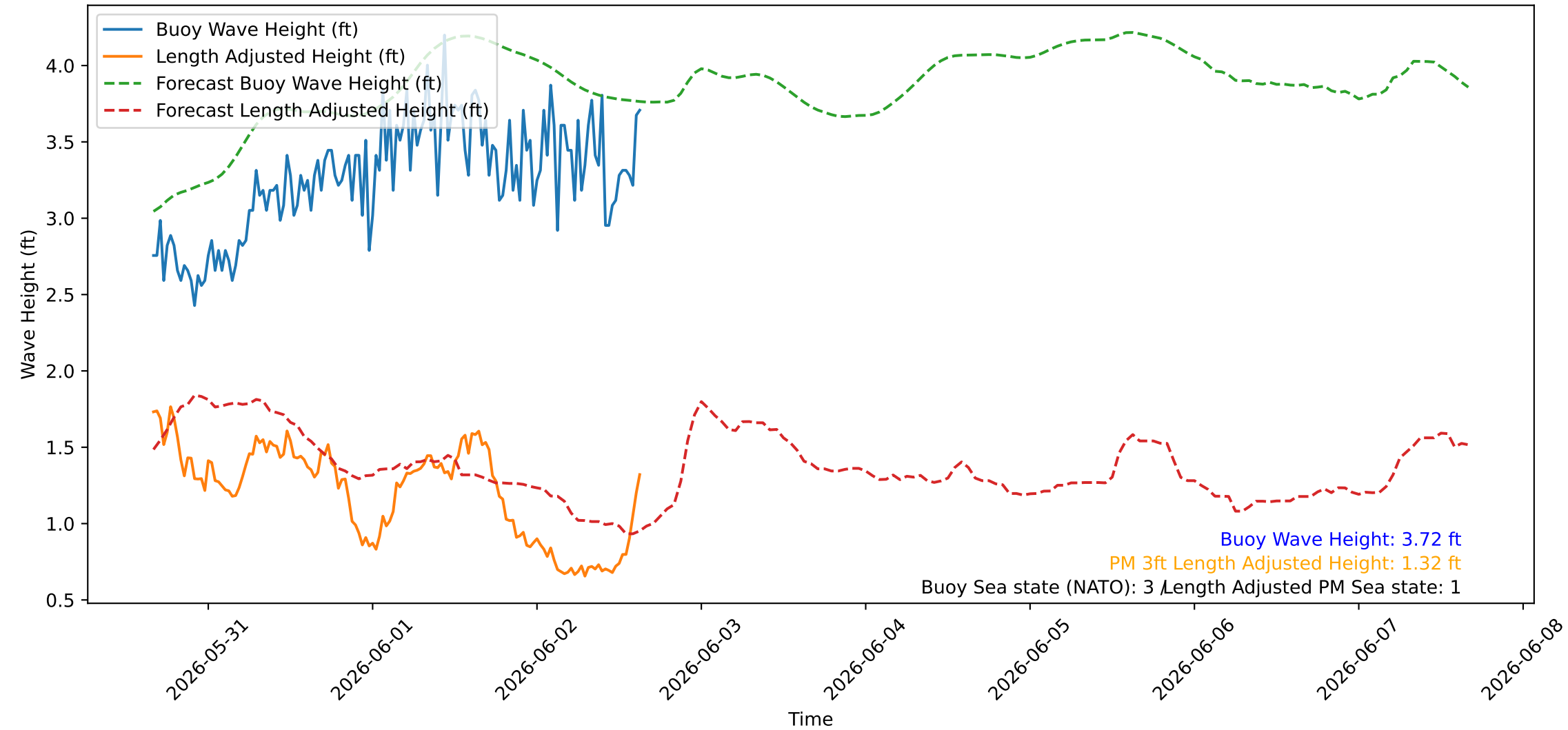
Wave Heights over Time for Red Beach at 2026-06-02 15:50:47
