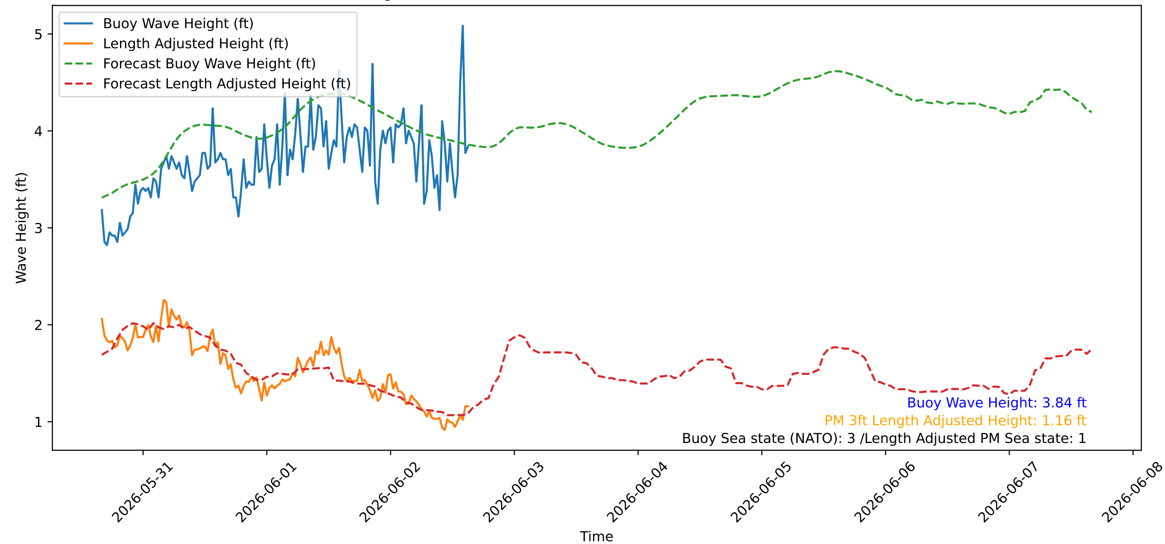
Wave Heights over Time for Oceanside Harbor at 2026-06-02 15:50:26
