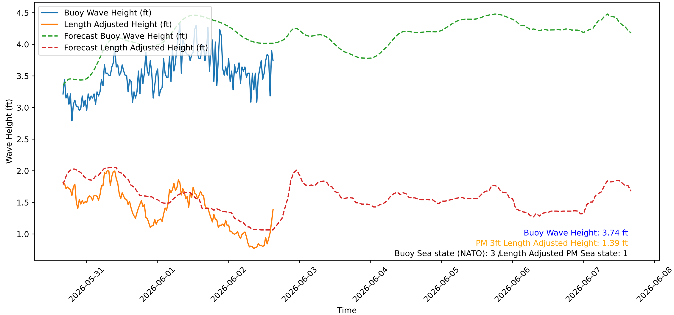
Wave Heights over Time for Green Beach at 2026-06-02 15:51:09
