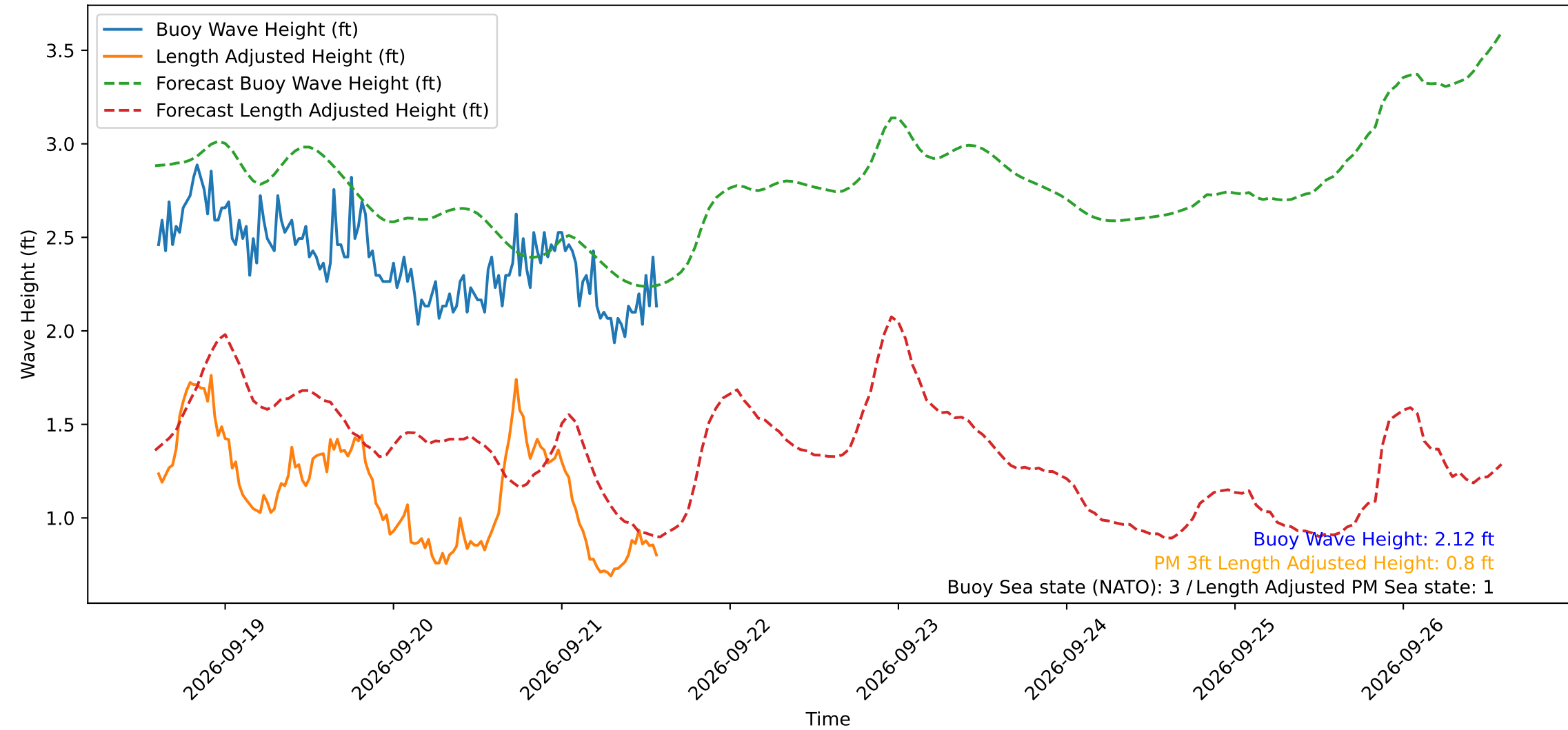
Wave Heights over Time for Red Beach at 2026-09-21 14:20:50
