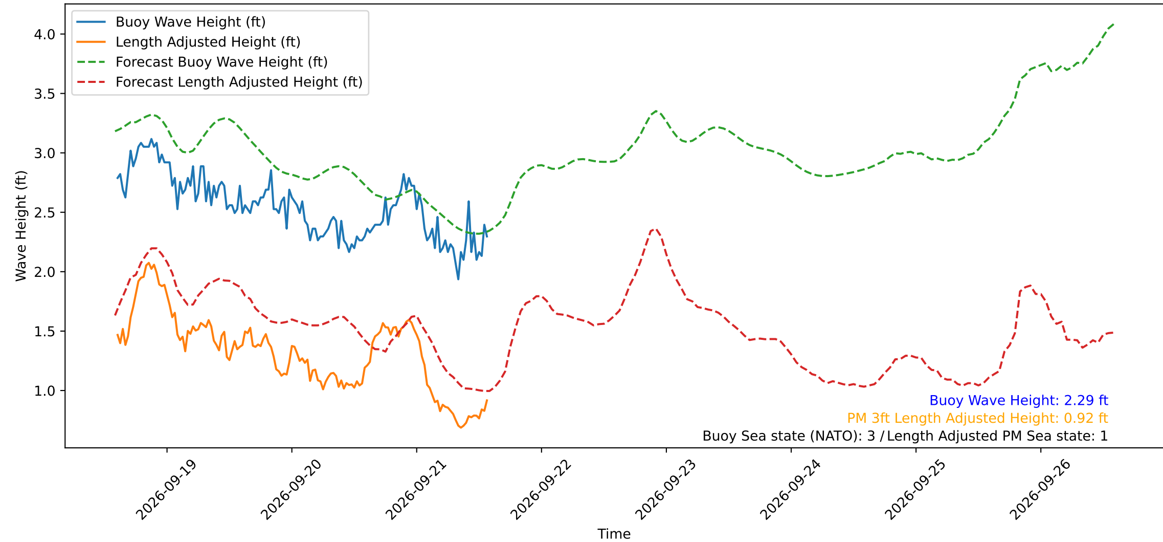
Wave Heights over Time for Green Beach at 2026-09-21 14:21:14
