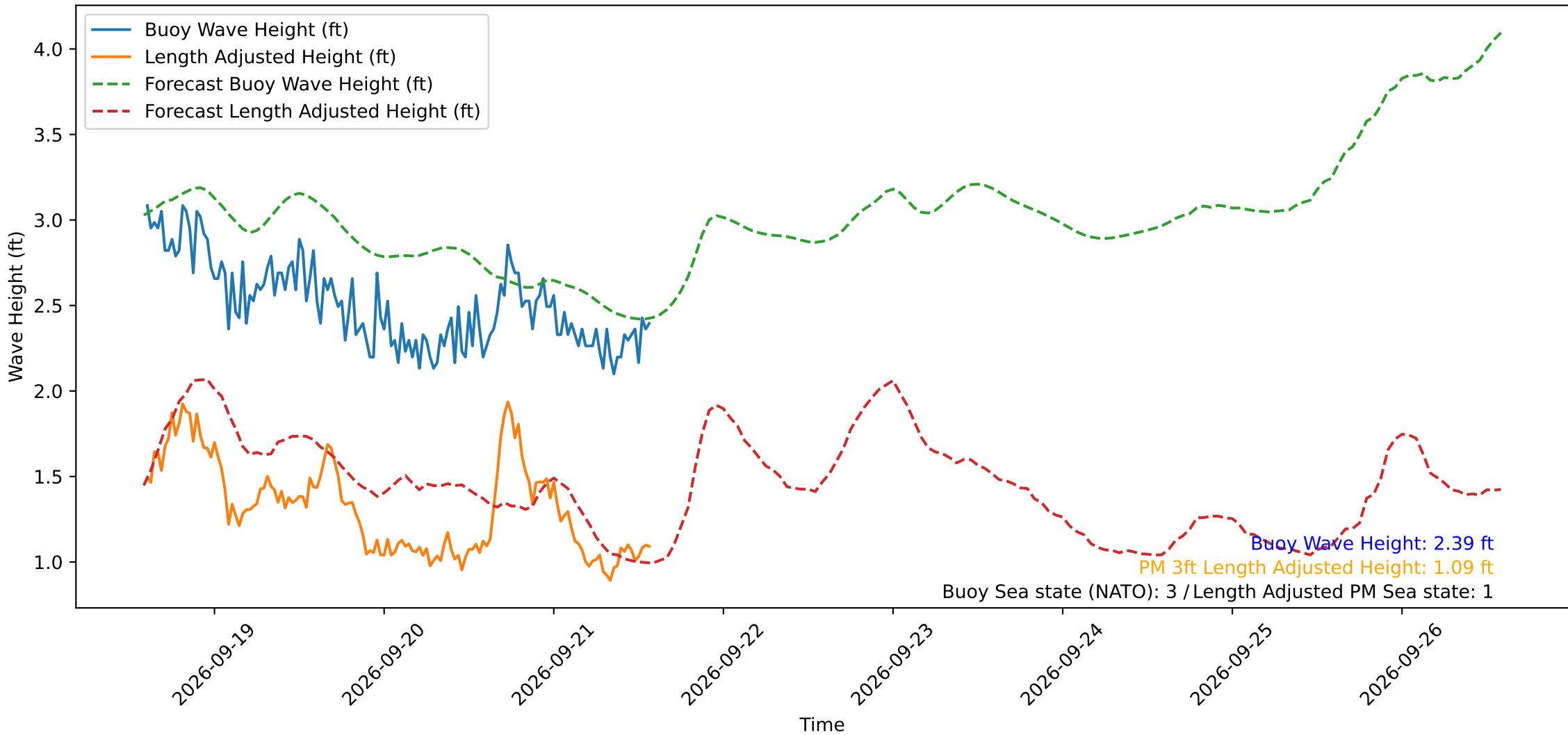
Wave Heights over Time for Oceanside Harbor at 2026-09-21 14:20:29
