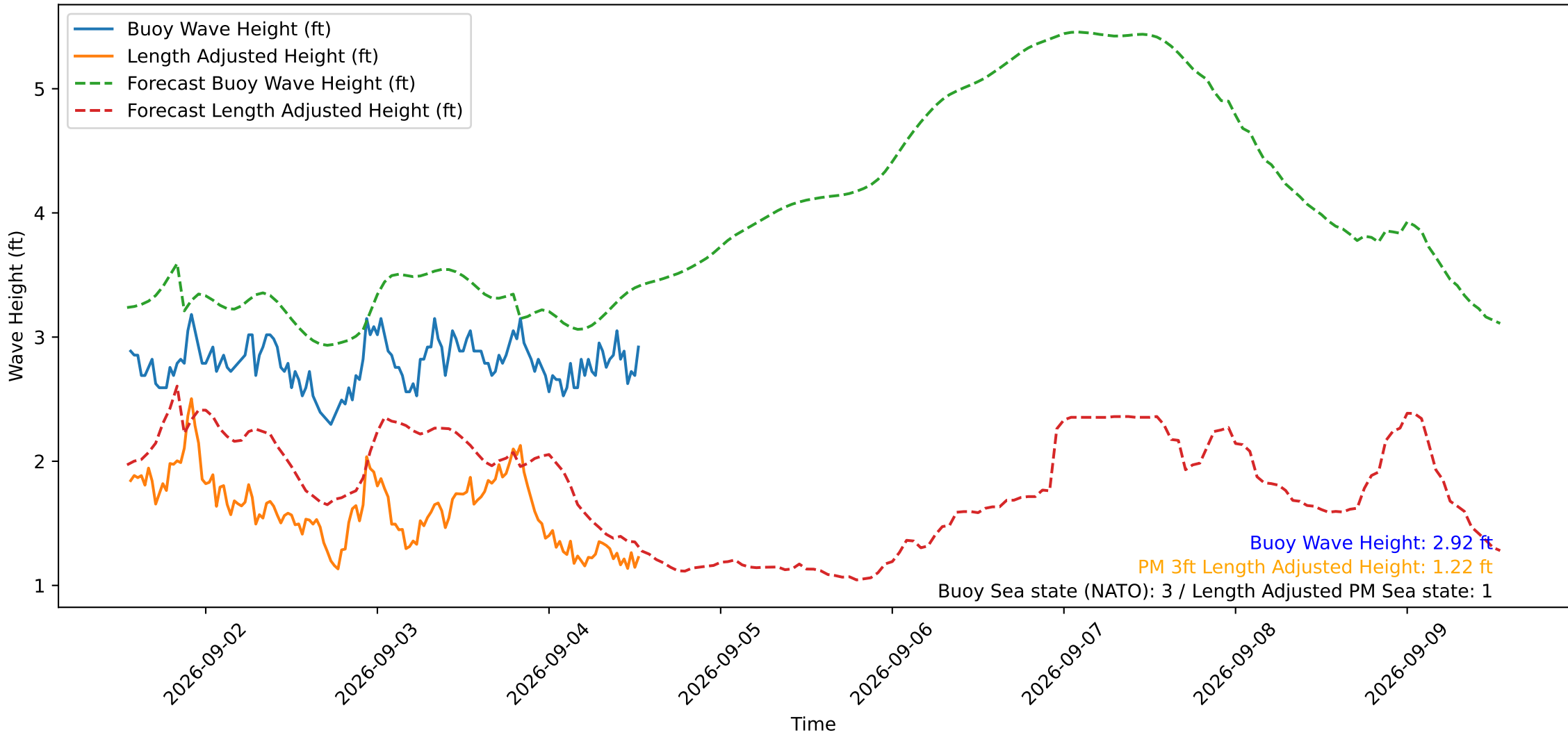
Wave Heights over Time for Red Beach at 2026-09-04 13:20:50
