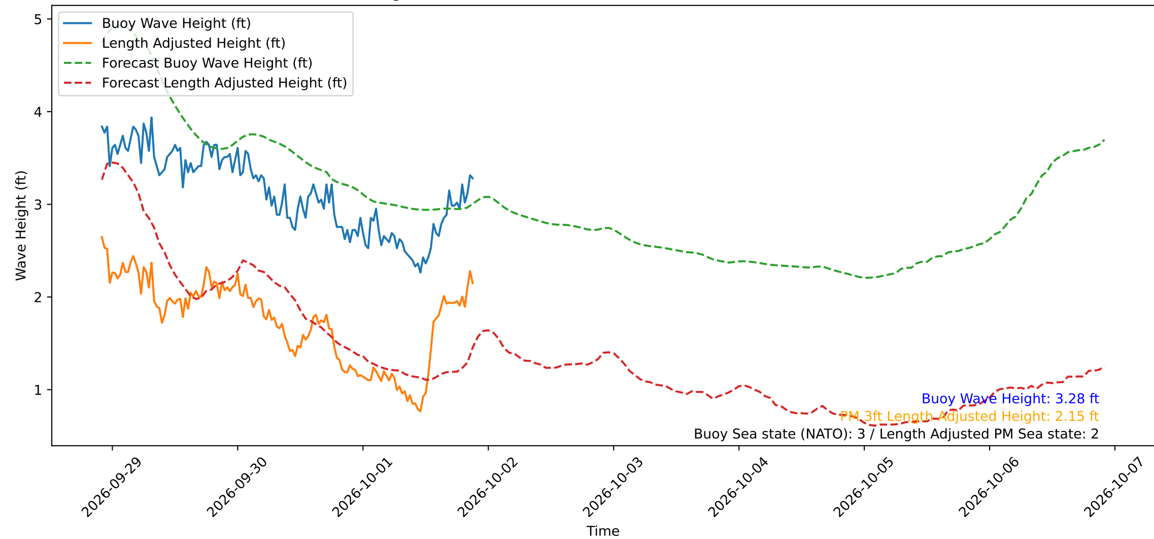
Wave Heights over Time for Oceanside Harbor at 2026-10-01 22:00:29
