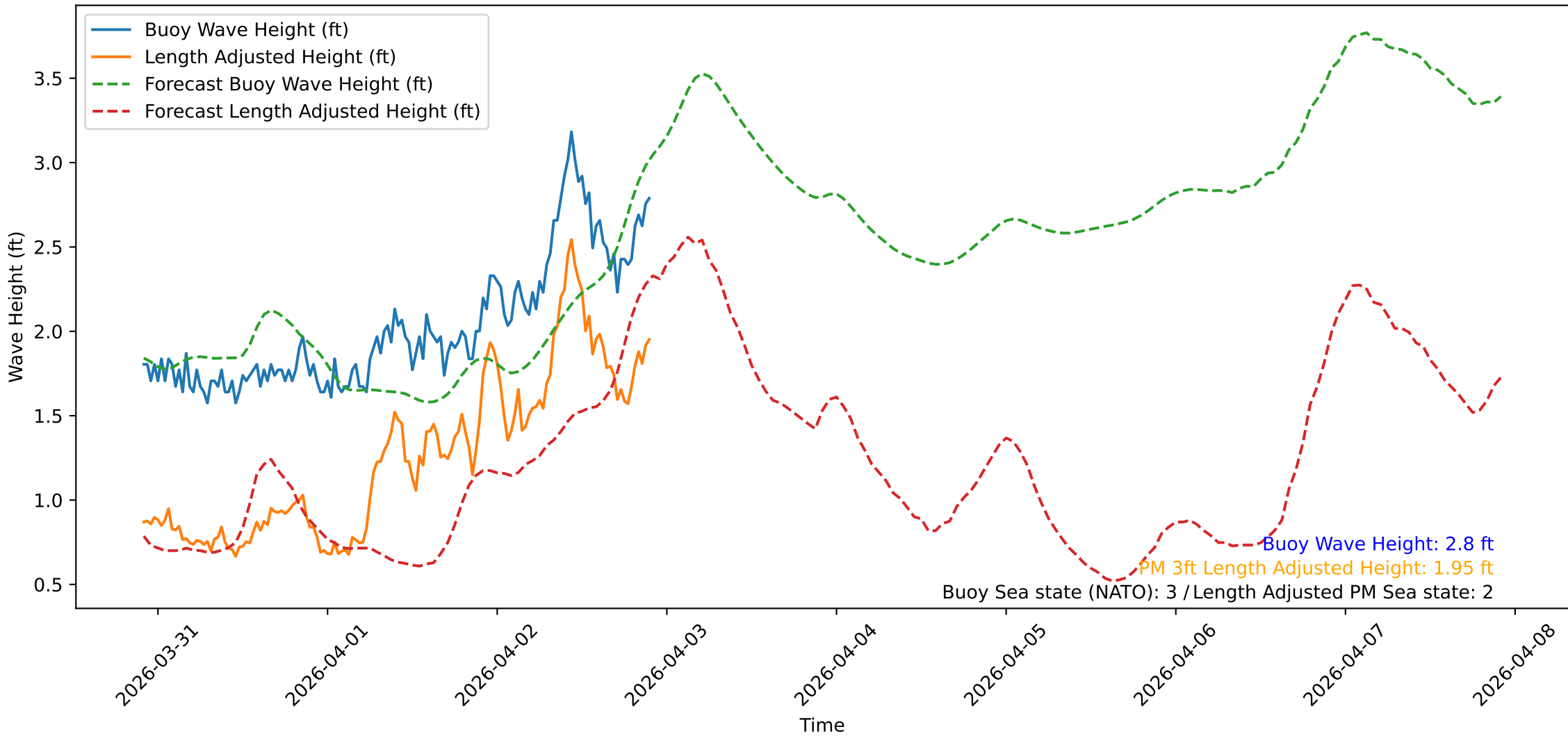
Wave Heights over Time for Oceanside Harbor at 2026-04-02 22:00:31
