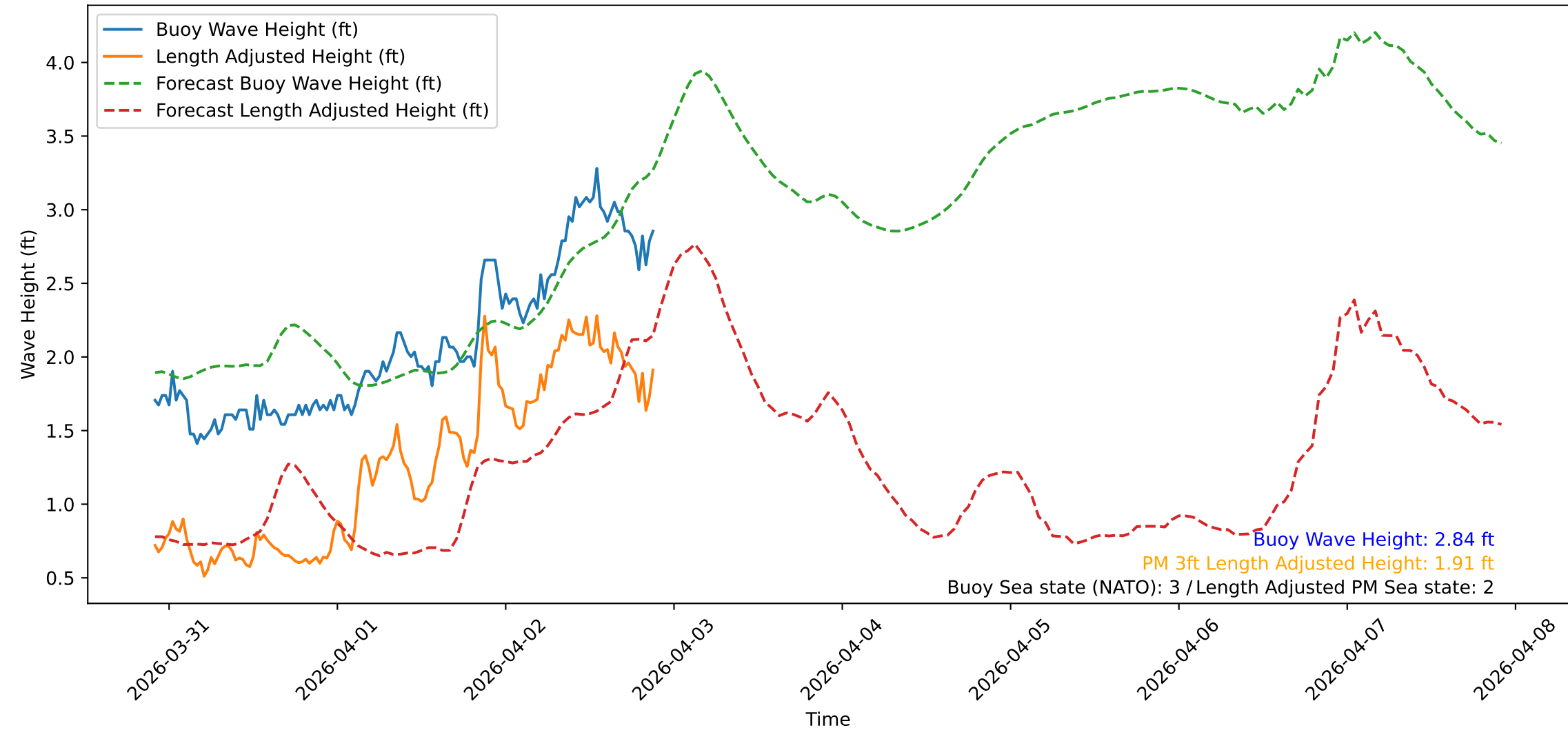
Wave Heights over Time for Green Beach at 2026-04-02 22:01:10
