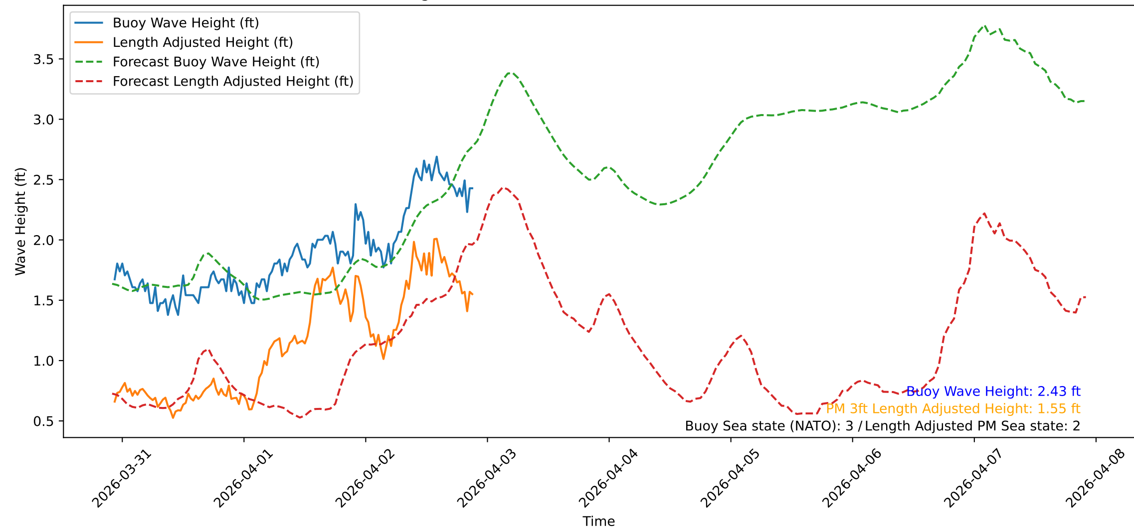
Wave Heights over Time for Red Beach at 2026-04-02 22:00:47
