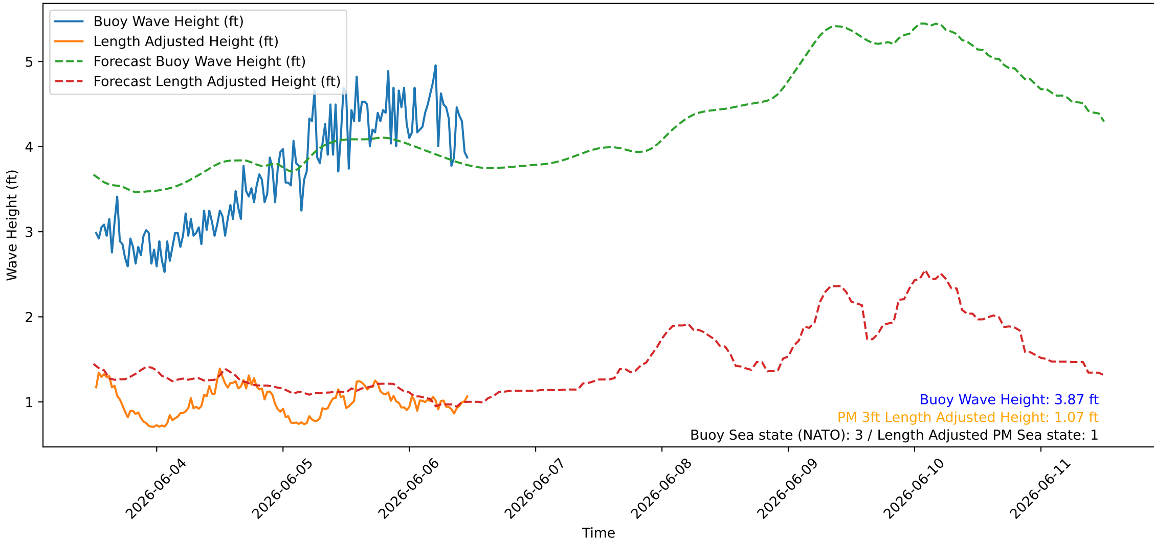
Wave Heights over Time for Red Beach at 2026-06-06 12:00:44
