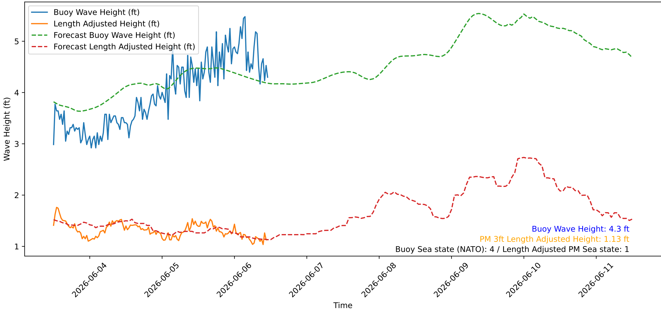
Wave Heights over Time for Oceanside Harbor at 2026-06-06 12:00:25
