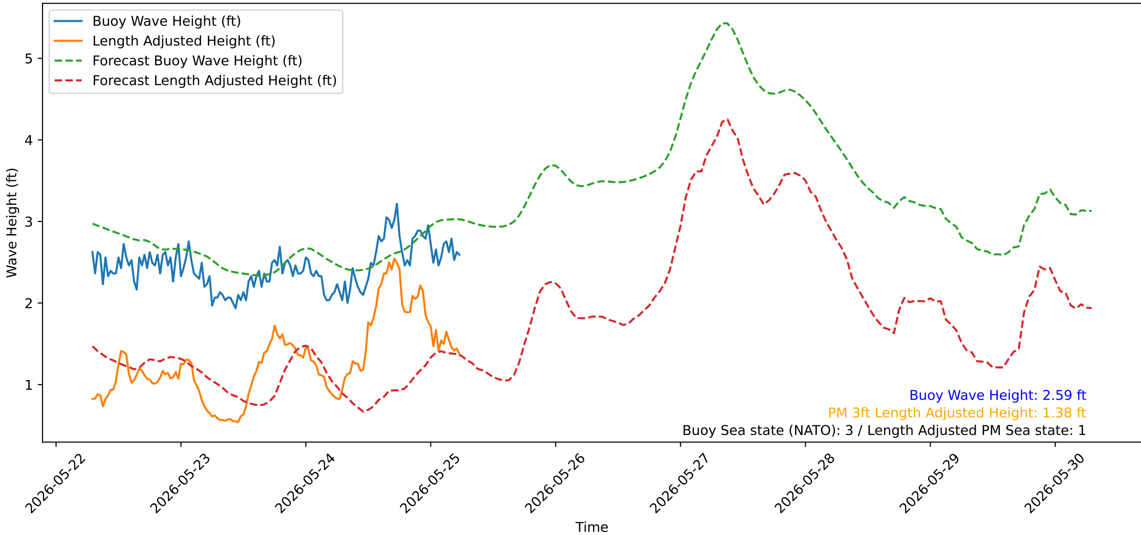
Wave Heights over Time for Red Beach at 2026-05-25 06:40:50
