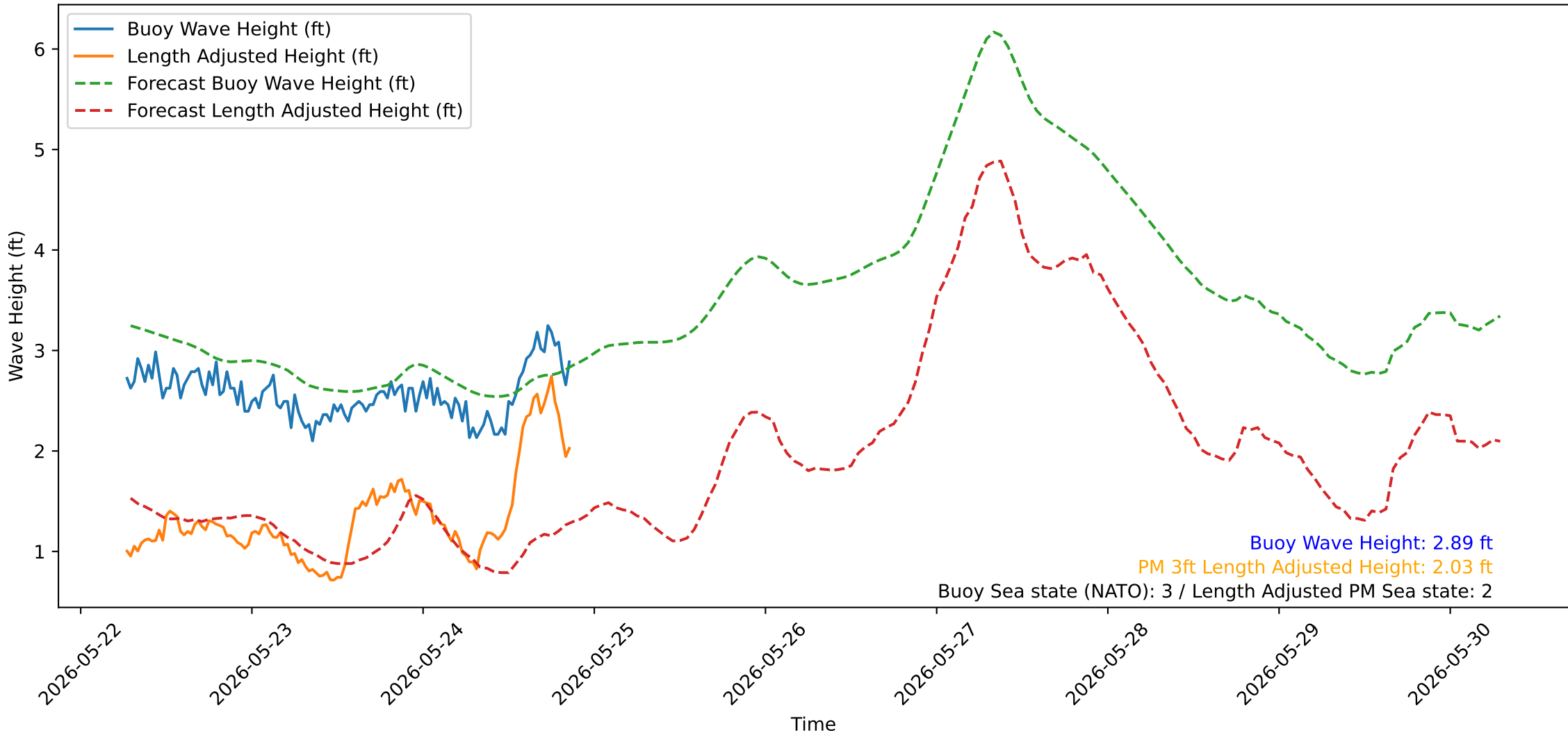
Wave Heights over Time for Oceanside Harbor at 2026-05-25 06:40:31
