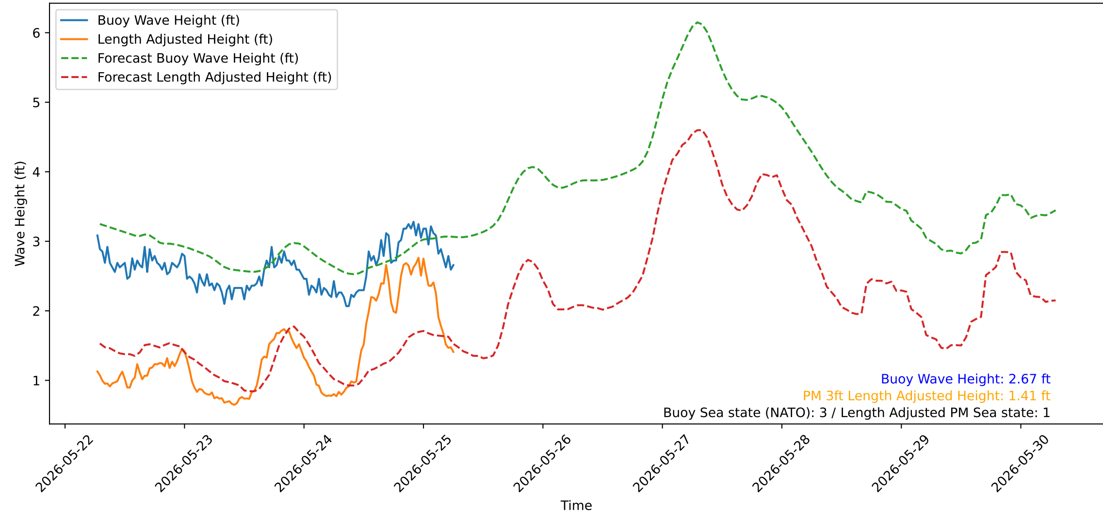
Wave Heights over Time for Green Beach at 2026-05-25 06:41:13
