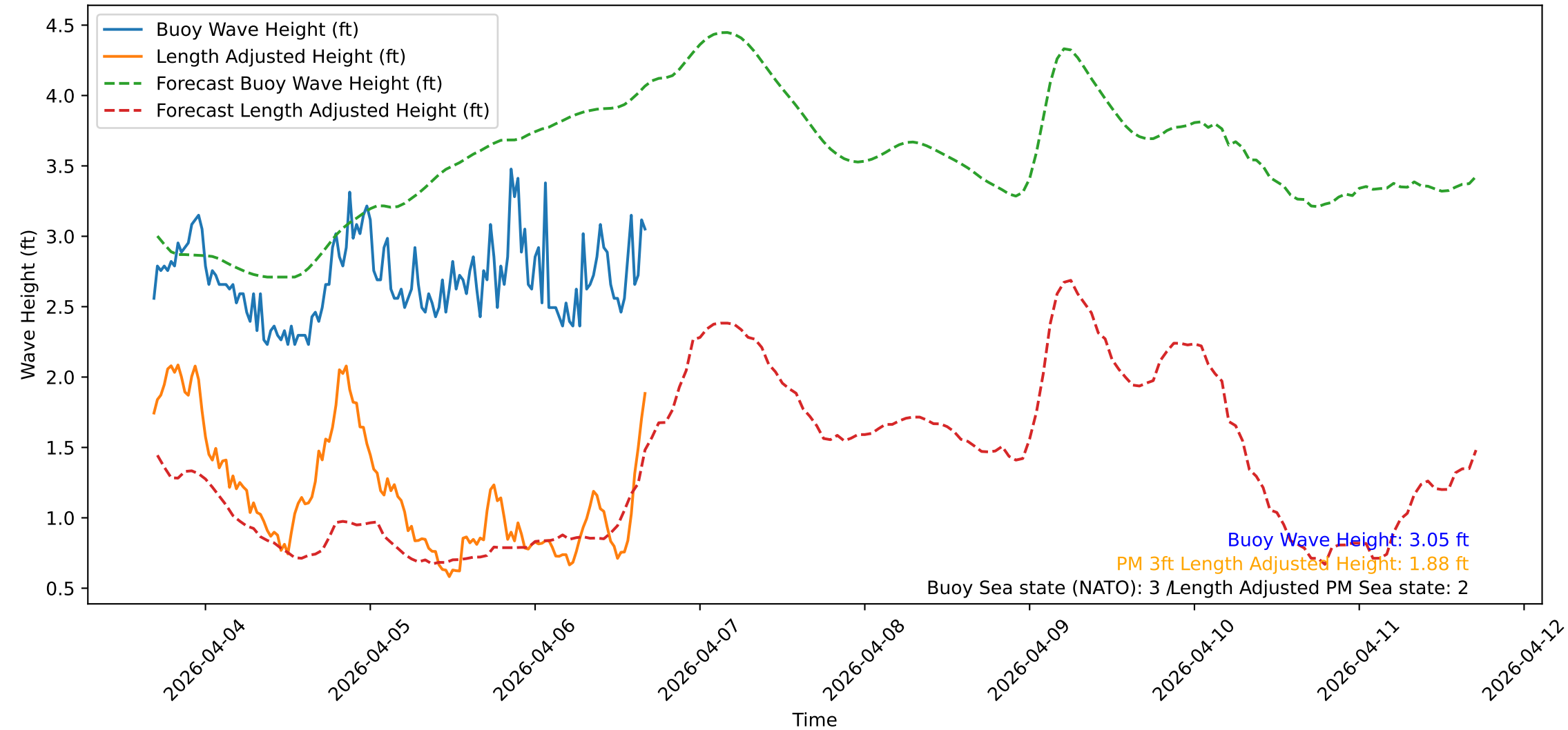
Wave Heights over Time for Green Beach at 2026-04-06 16:41:10
