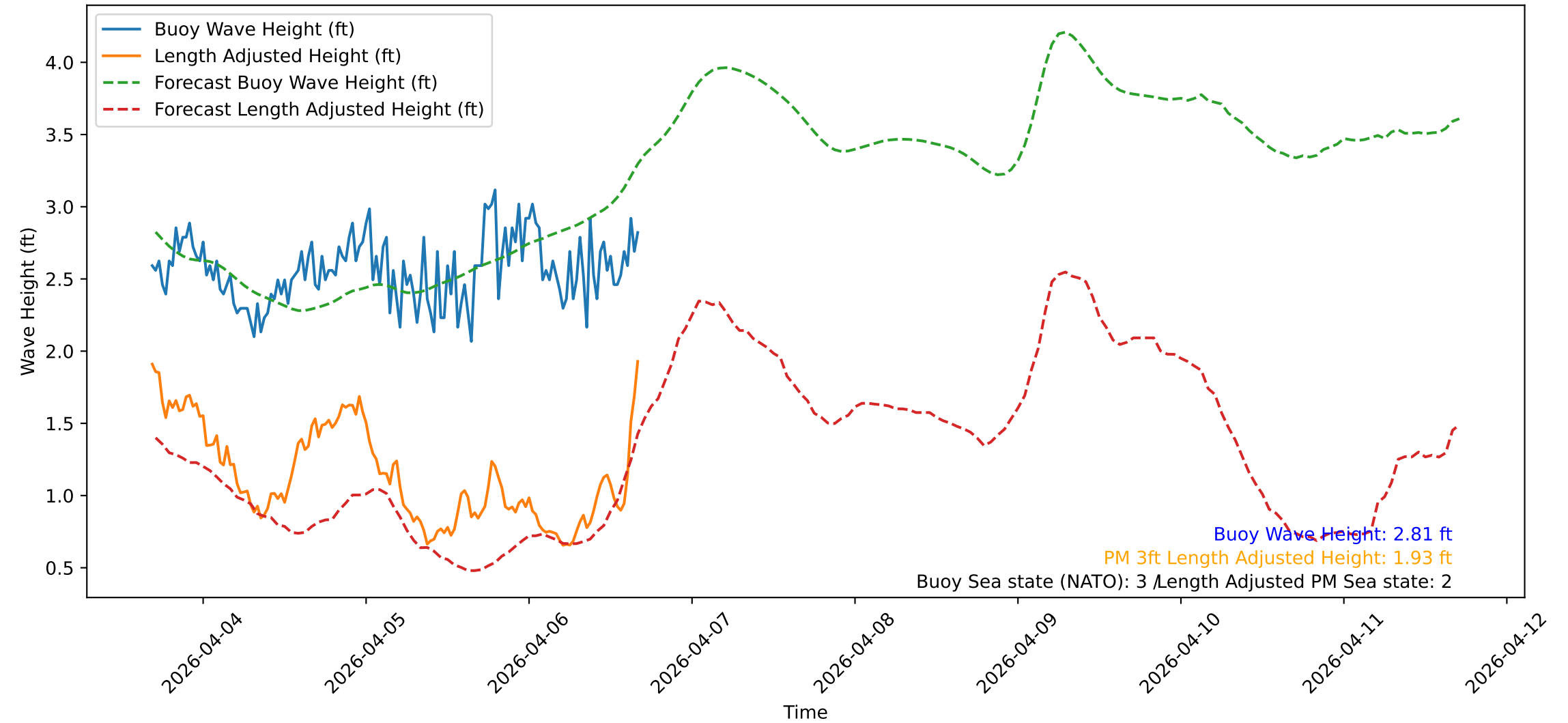
Wave Heights over Time for Oceanside Harbor at 2026-04-06 16:40:31
