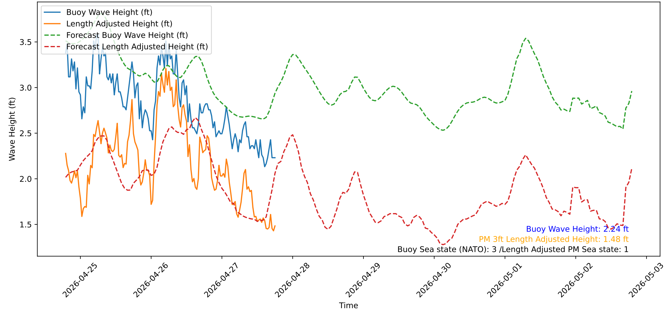
Wave Heights over Time for Green Beach at 2026-04-27 18:51:14
