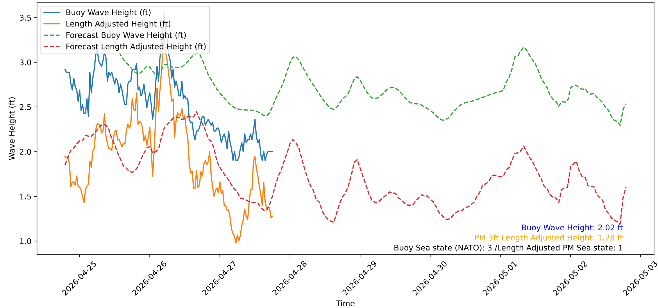
Wave Heights over Time for Red Beach at 2026-04-27 18:50:52
