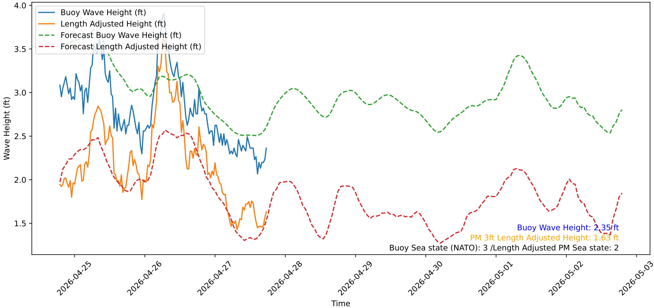
Wave Heights over Time for Oceanside Harbor at 2026-04-27 18:50:31
