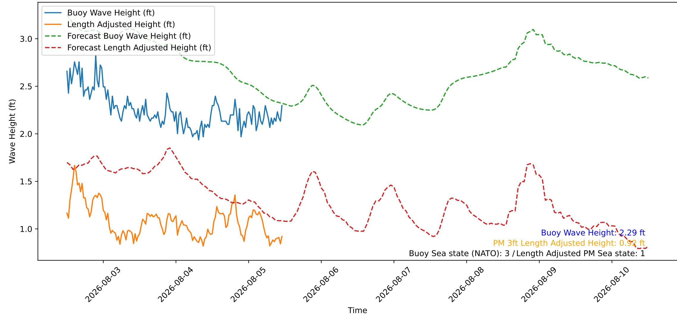
Wave Heights over Time for Green Beach at 2026-08-05 11:51:09
