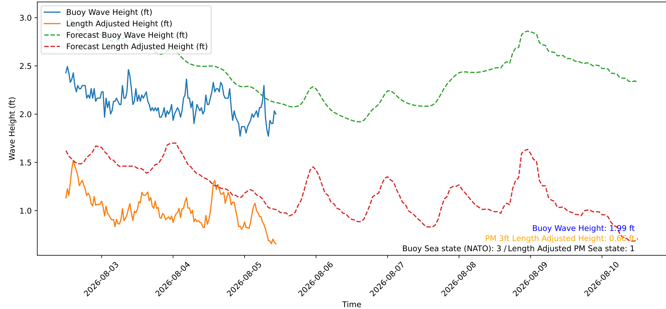
Wave Heights over Time for Red Beach at 2026-08-05 11:50:47
