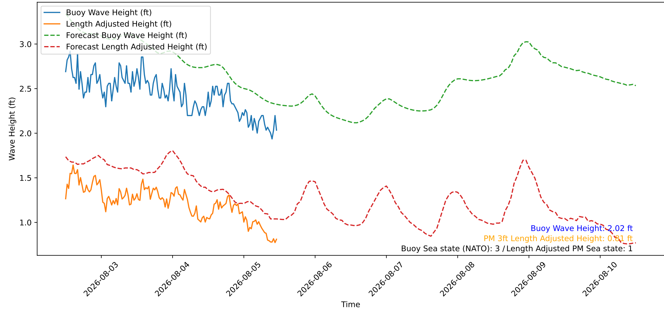
Wave Heights over Time for Oceanside Harbor at 2026-08-05 11:50:26
