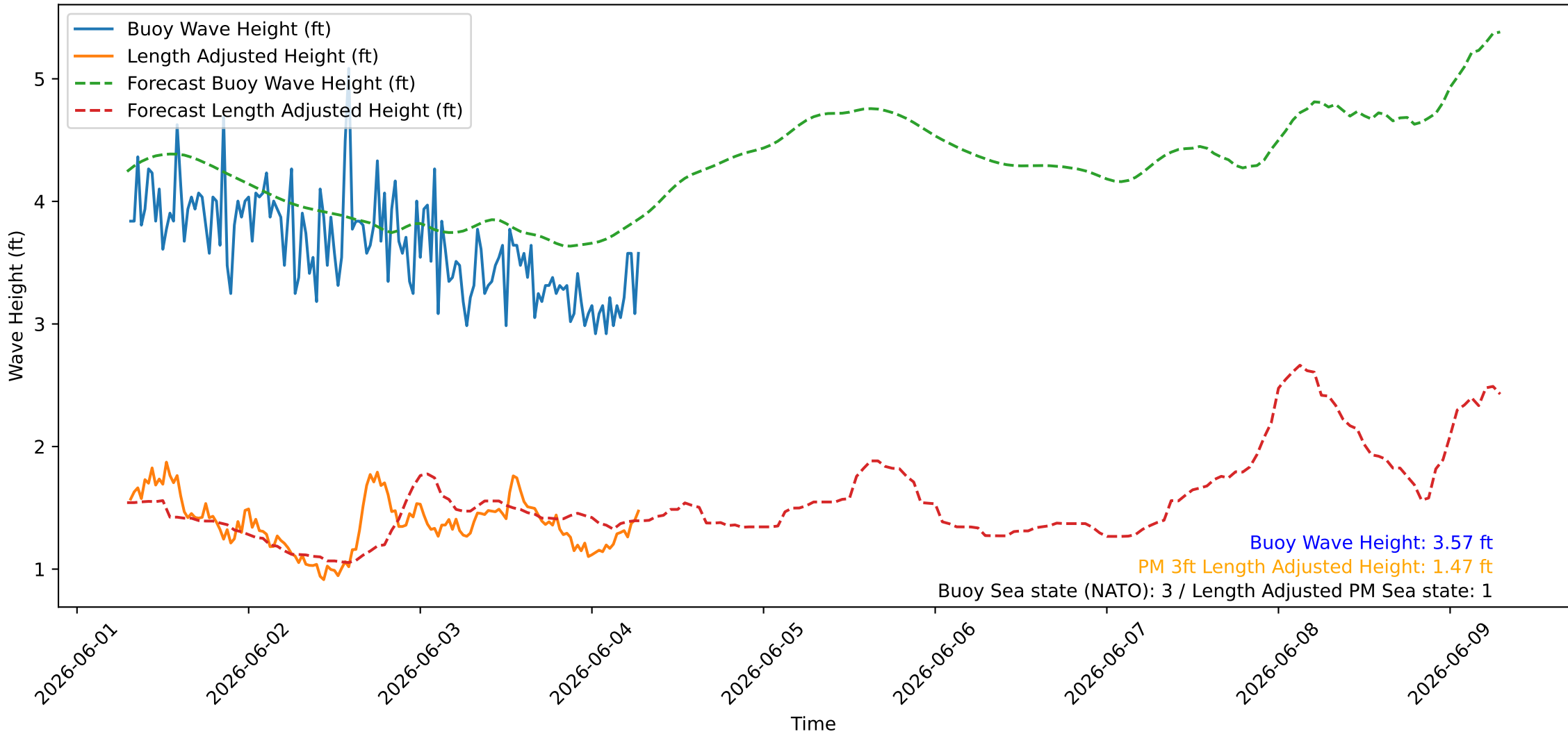
Wave Heights over Time for Oceanside Harbor at 2026-06-04 07:20:26
