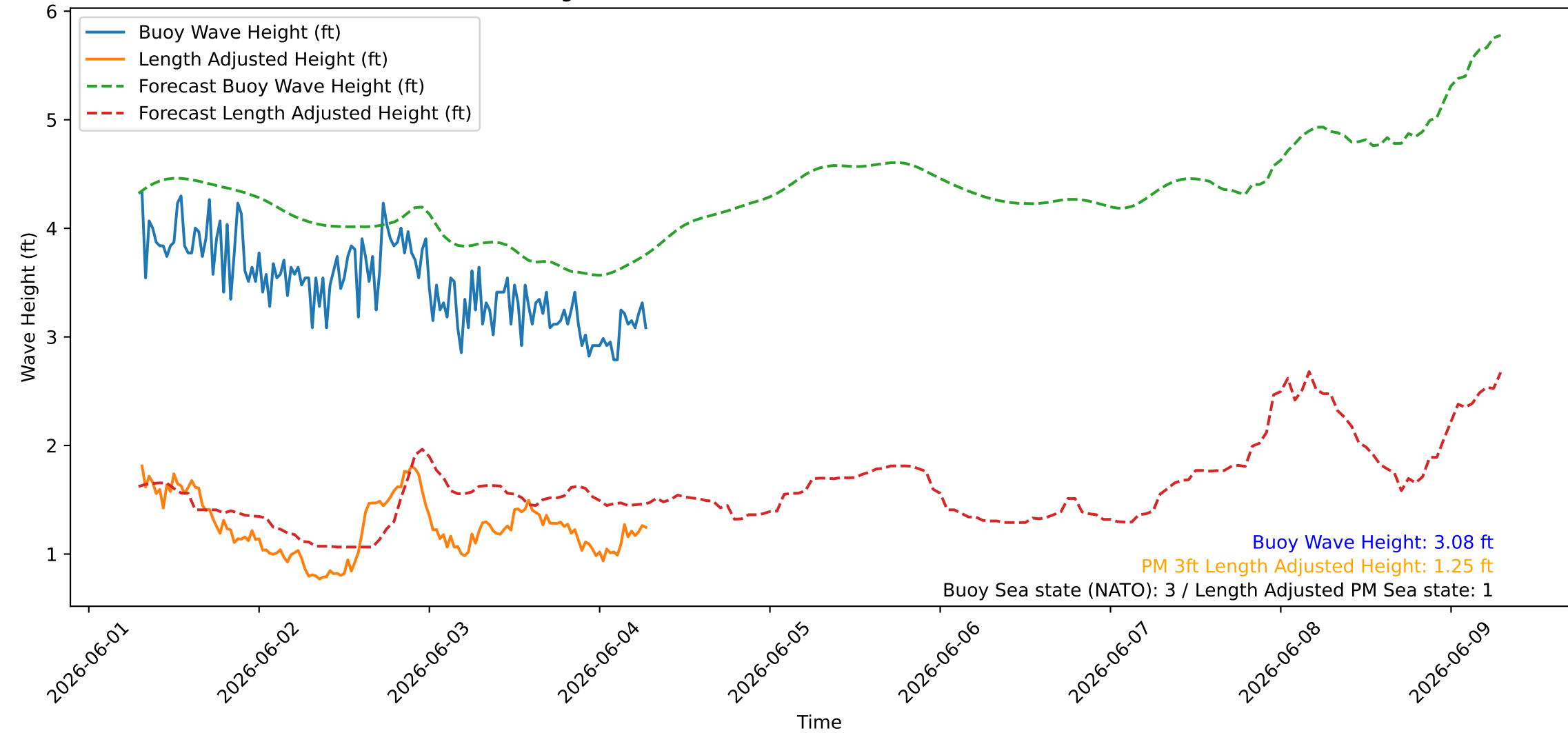
Wave Heights over Time for Green Beach at 2026-06-04 07:21:10
