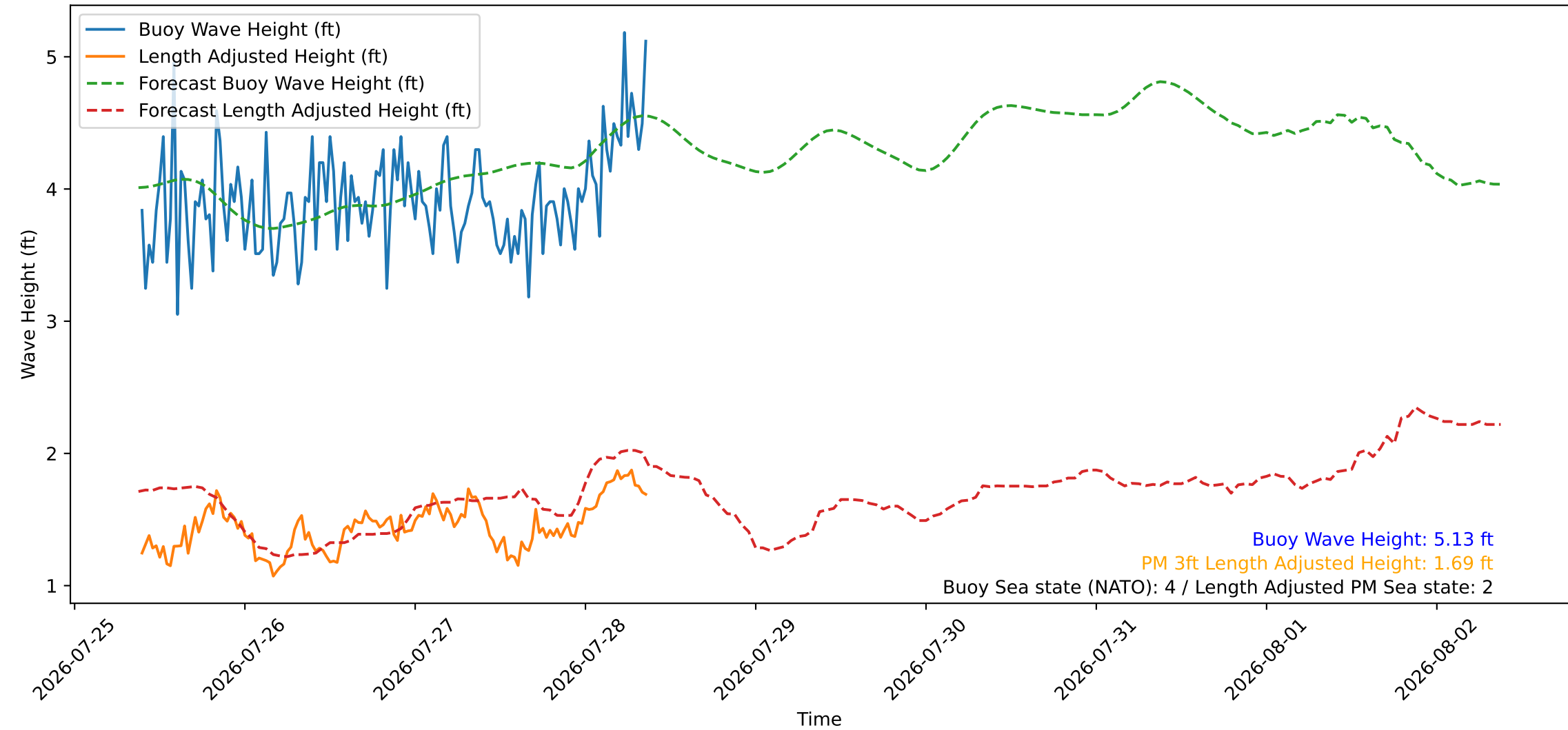
Wave Heights over Time for Oceanside Harbor at 2026-07-28 09:20:27
