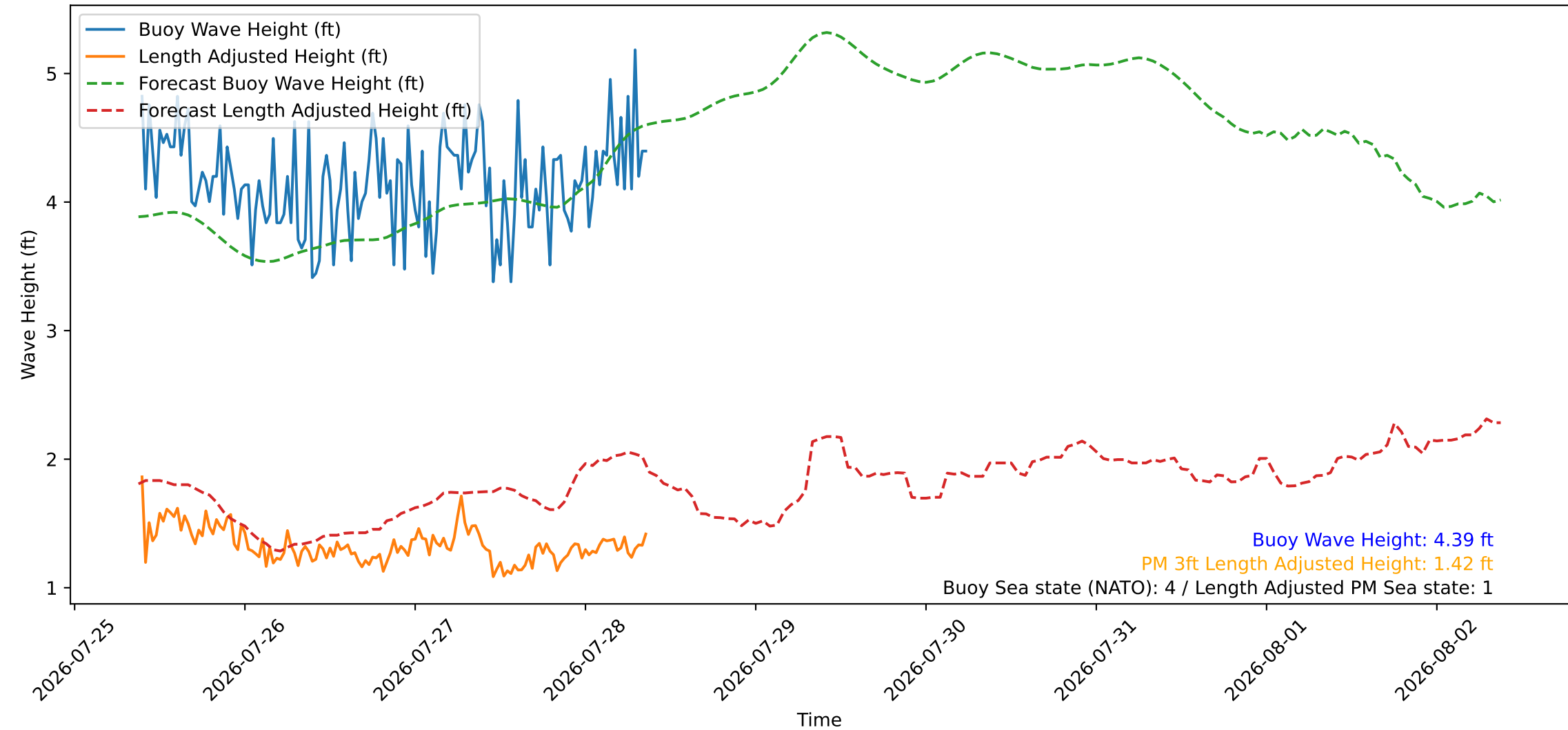
Wave Heights over Time for Green Beach at 2026-07-28 09:21:12
