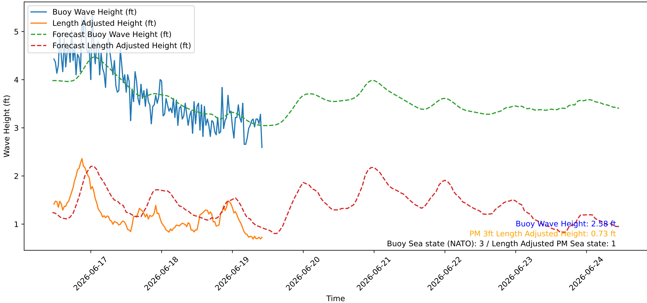
Wave Heights over Time for Red Beach at 2026-06-19 11:00:45
