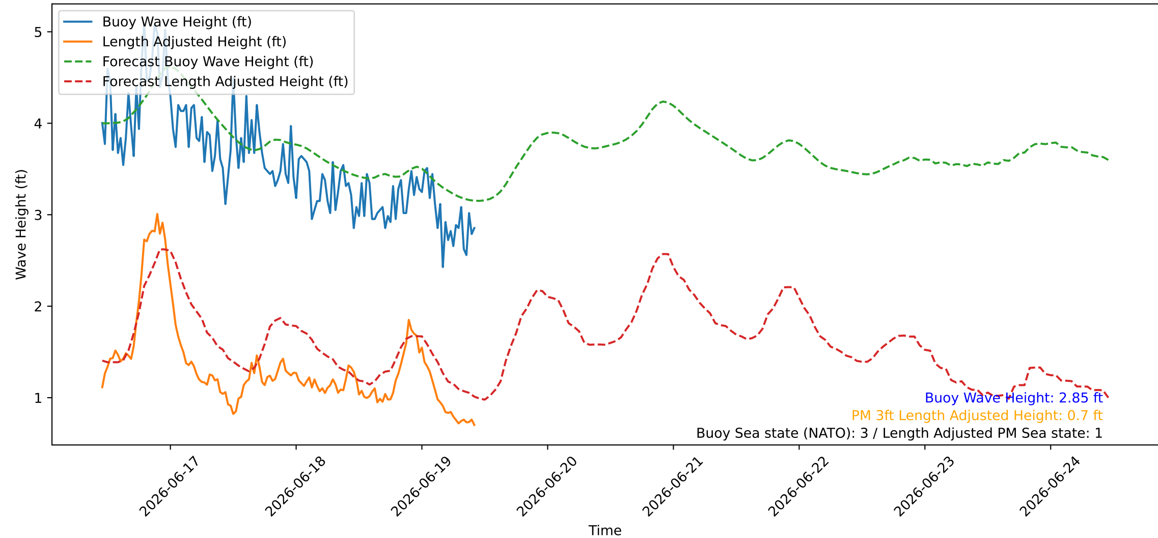
Wave Heights over Time for Green Beach at 2026-06-19 11:01:07
