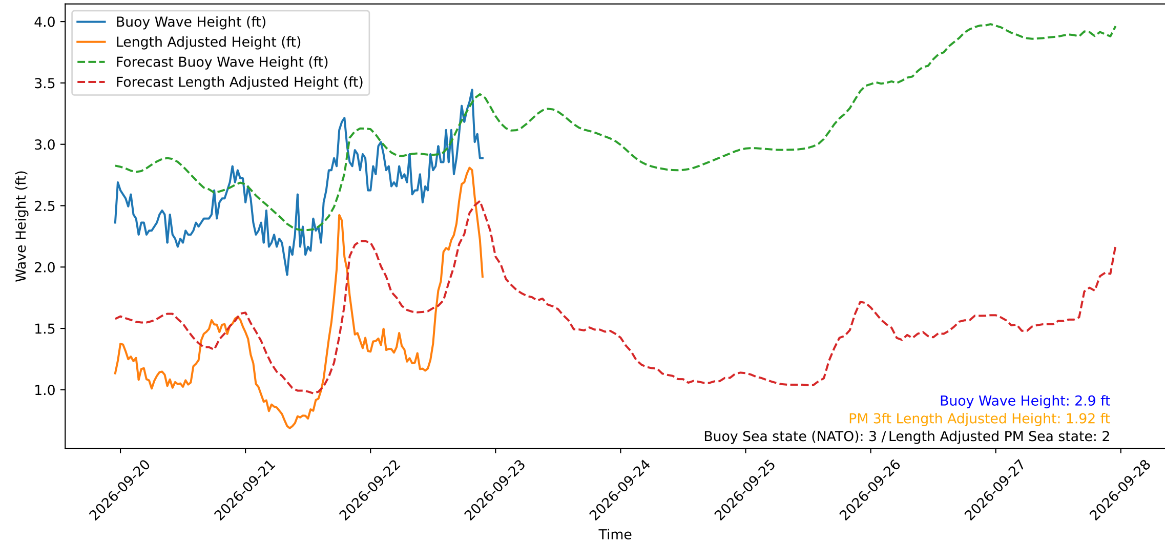
Wave Heights over Time for Green Beach at 2026-09-22 22:31:12
