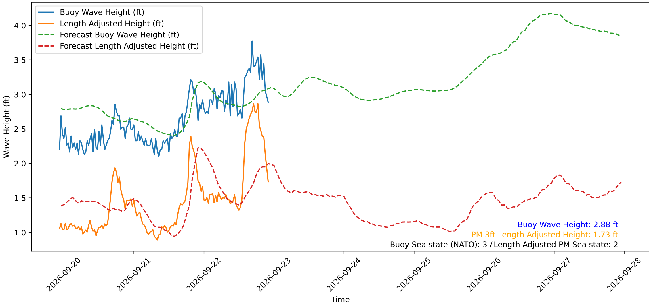
Wave Heights over Time for Oceanside Harbor at 2026-09-22 22:30:29
