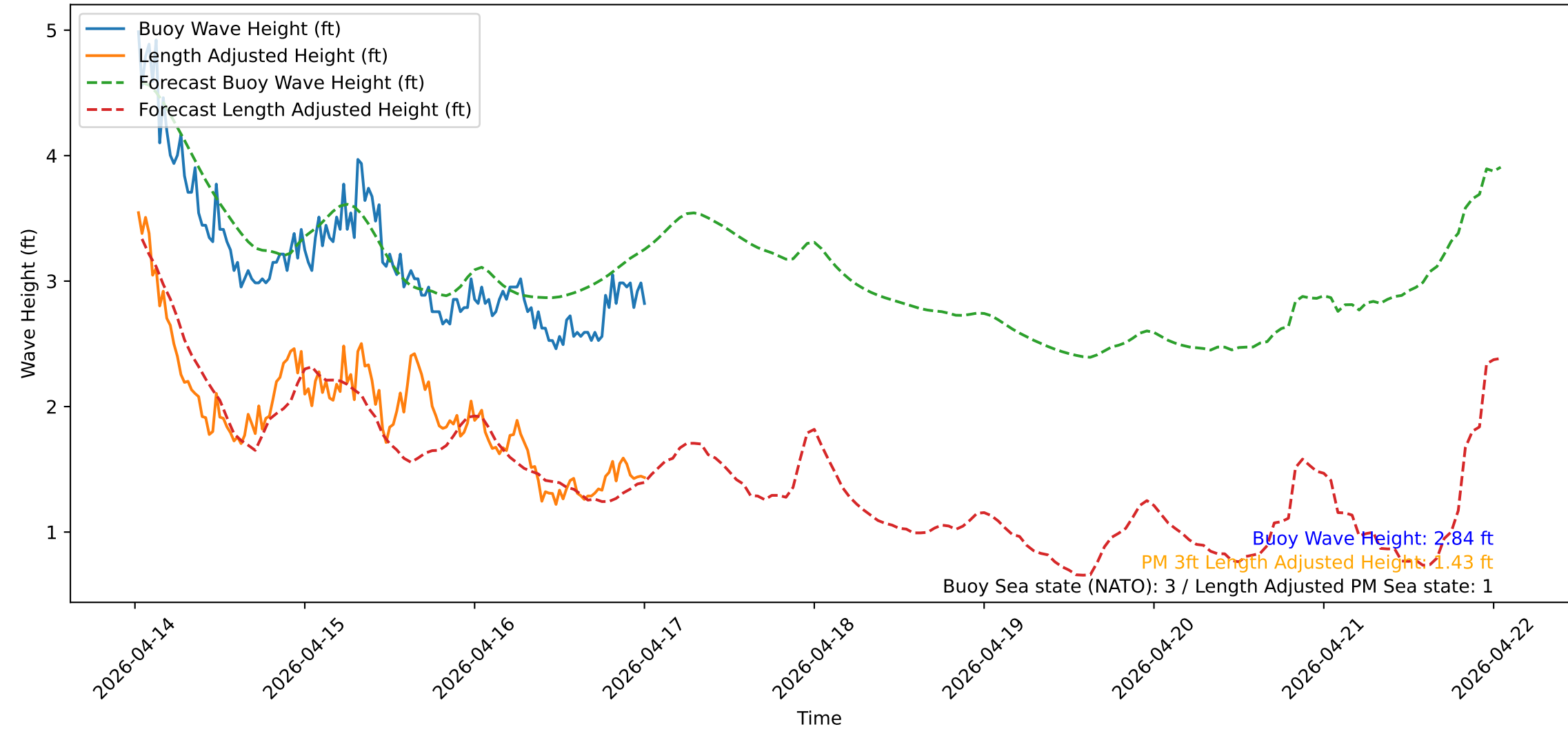
Wave Heights over Time for Green Beach at 2026-04-17 00:41:14
