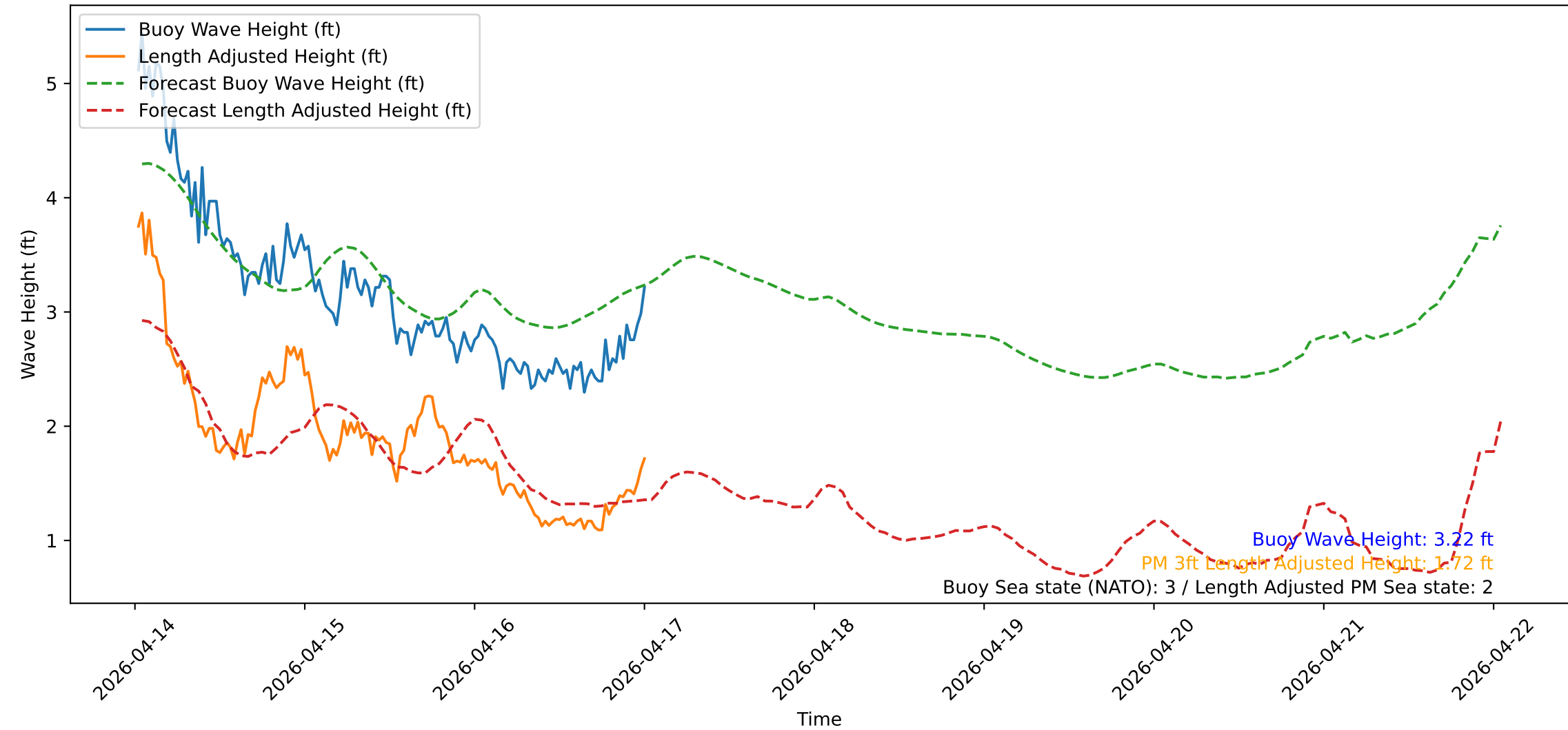
Wave Heights over Time for Oceanside Harbor at 2026-04-17 00:40:32
