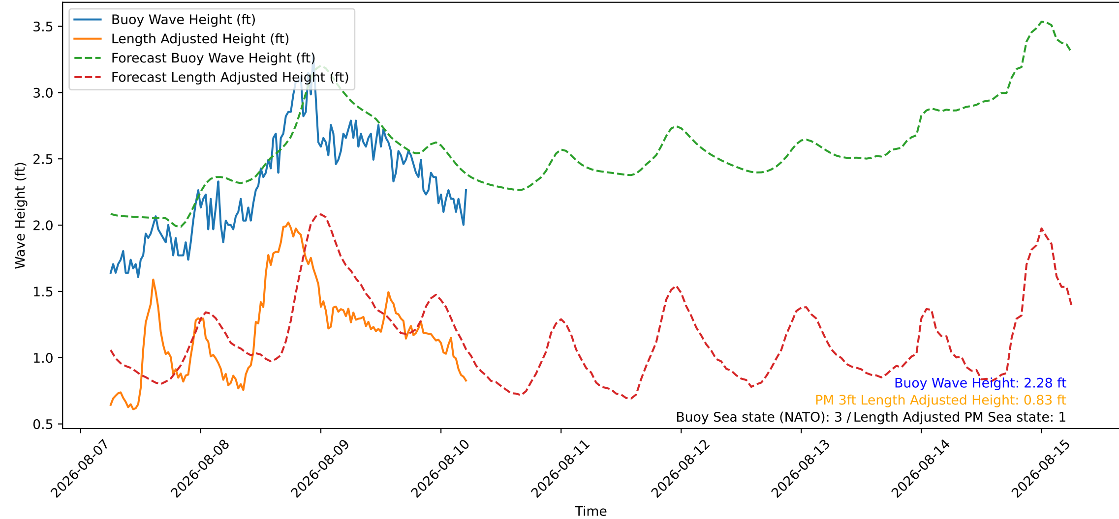
Wave Heights over Time for Red Beach at 2026-08-10 05:40:46
