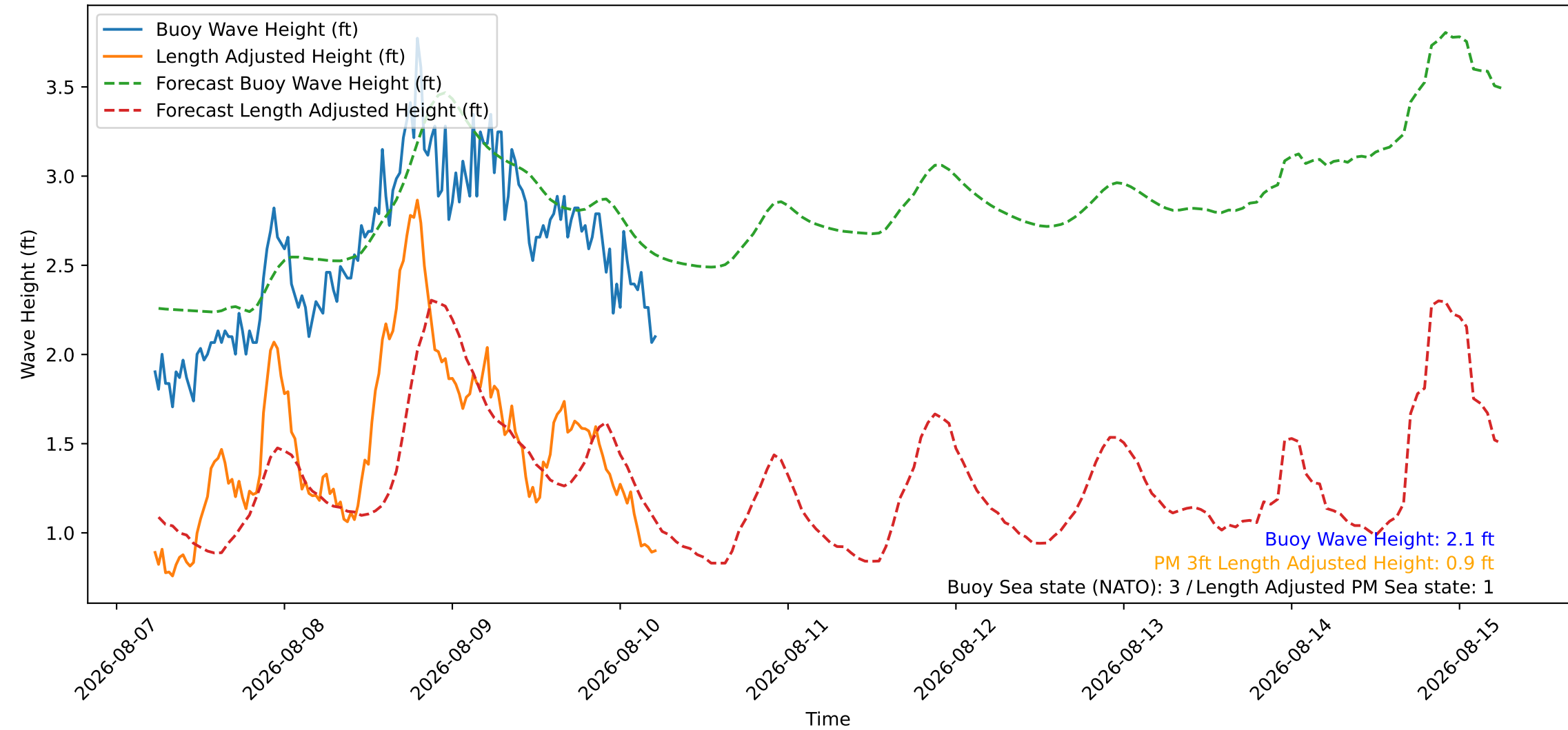
Wave Heights over Time for Green Beach at 2026-08-10 05:41:09
