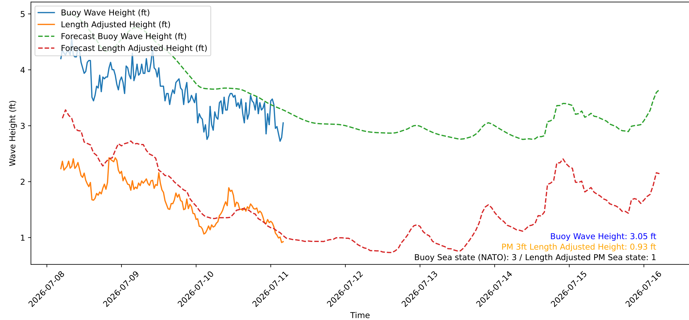
Wave Heights over Time for Green Beach at 2026-07-11 04:41:08
