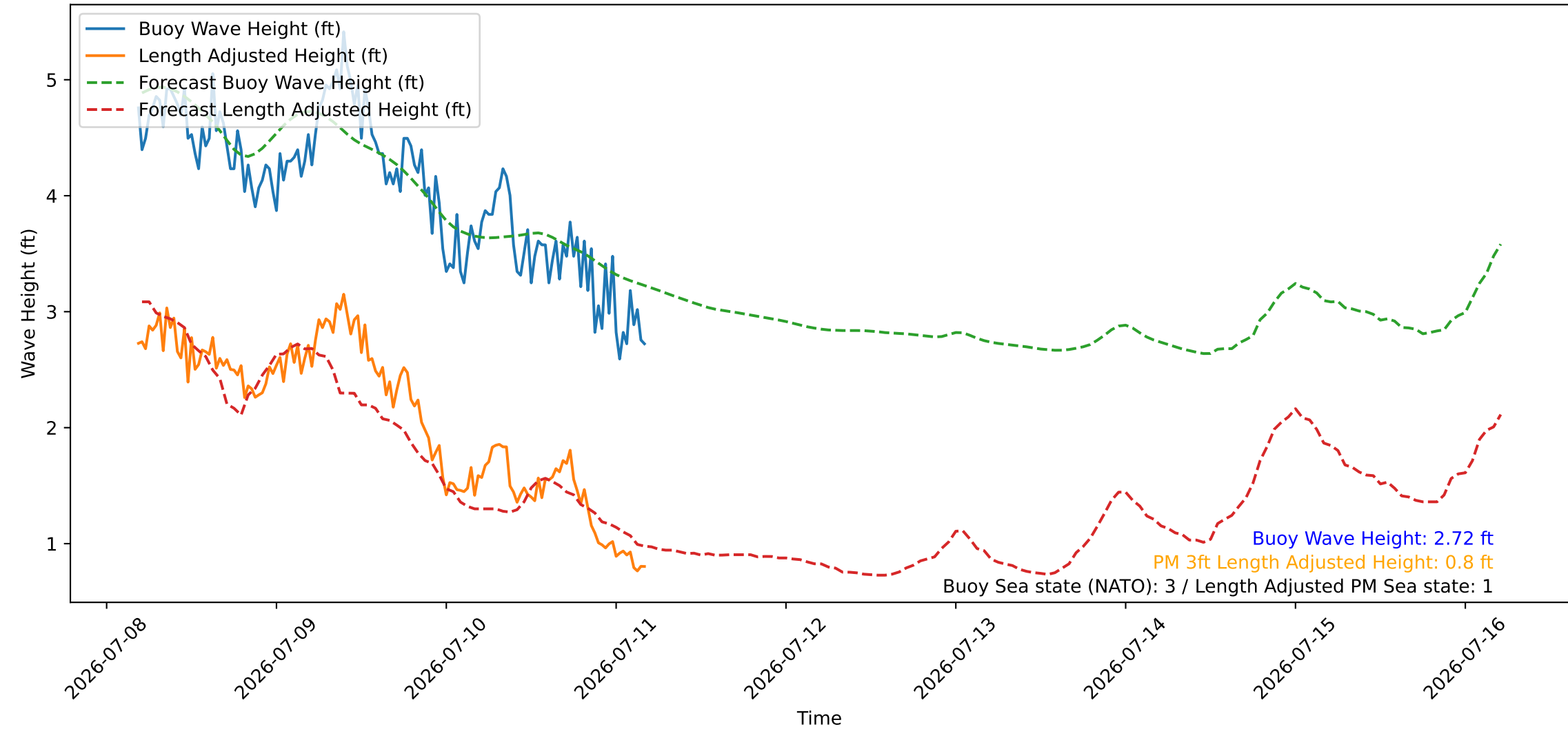
Wave Heights over Time for Oceanside Harbor at 2026-07-11 04:40:26
