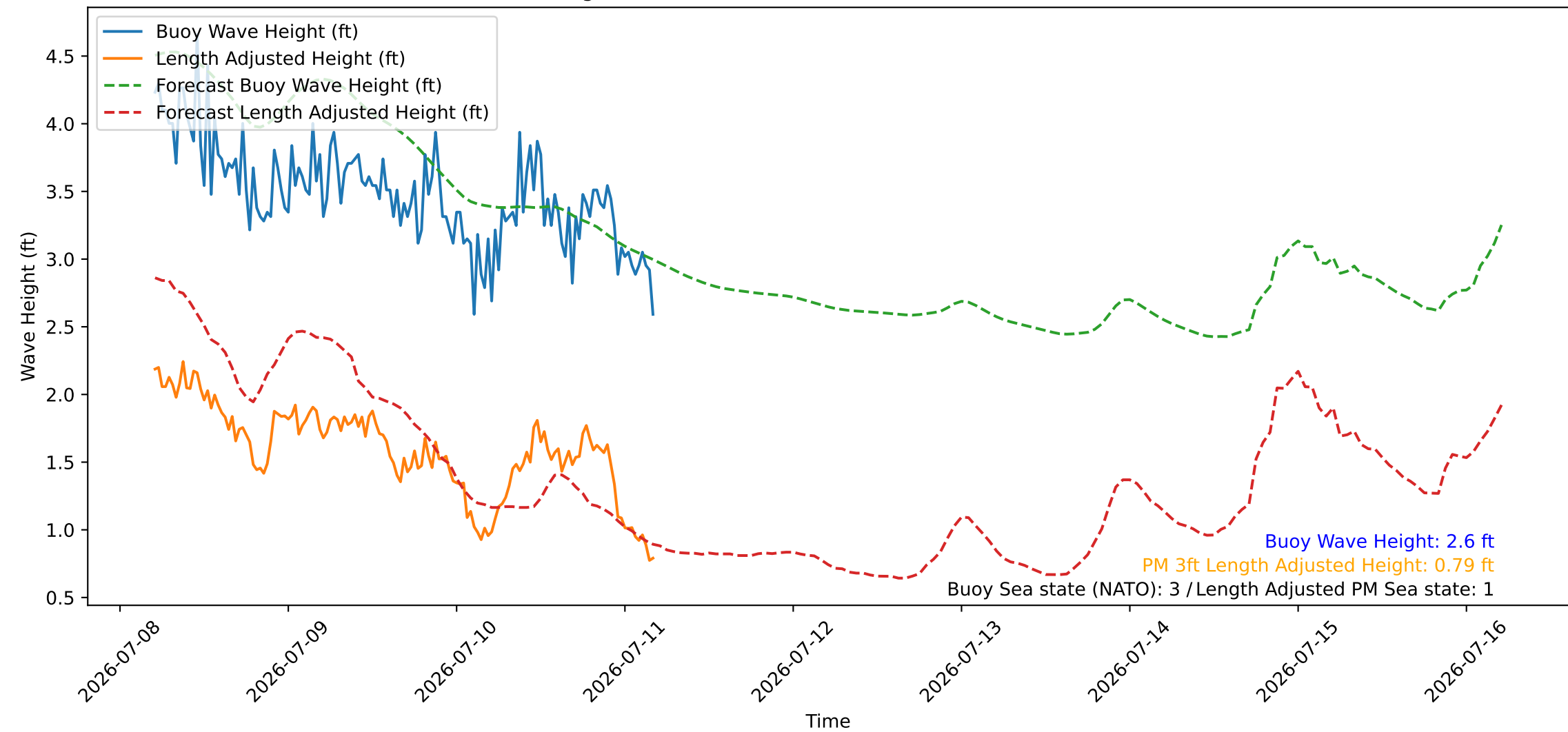
Wave Heights over Time for Red Beach at 2026-07-11 04:40:46
