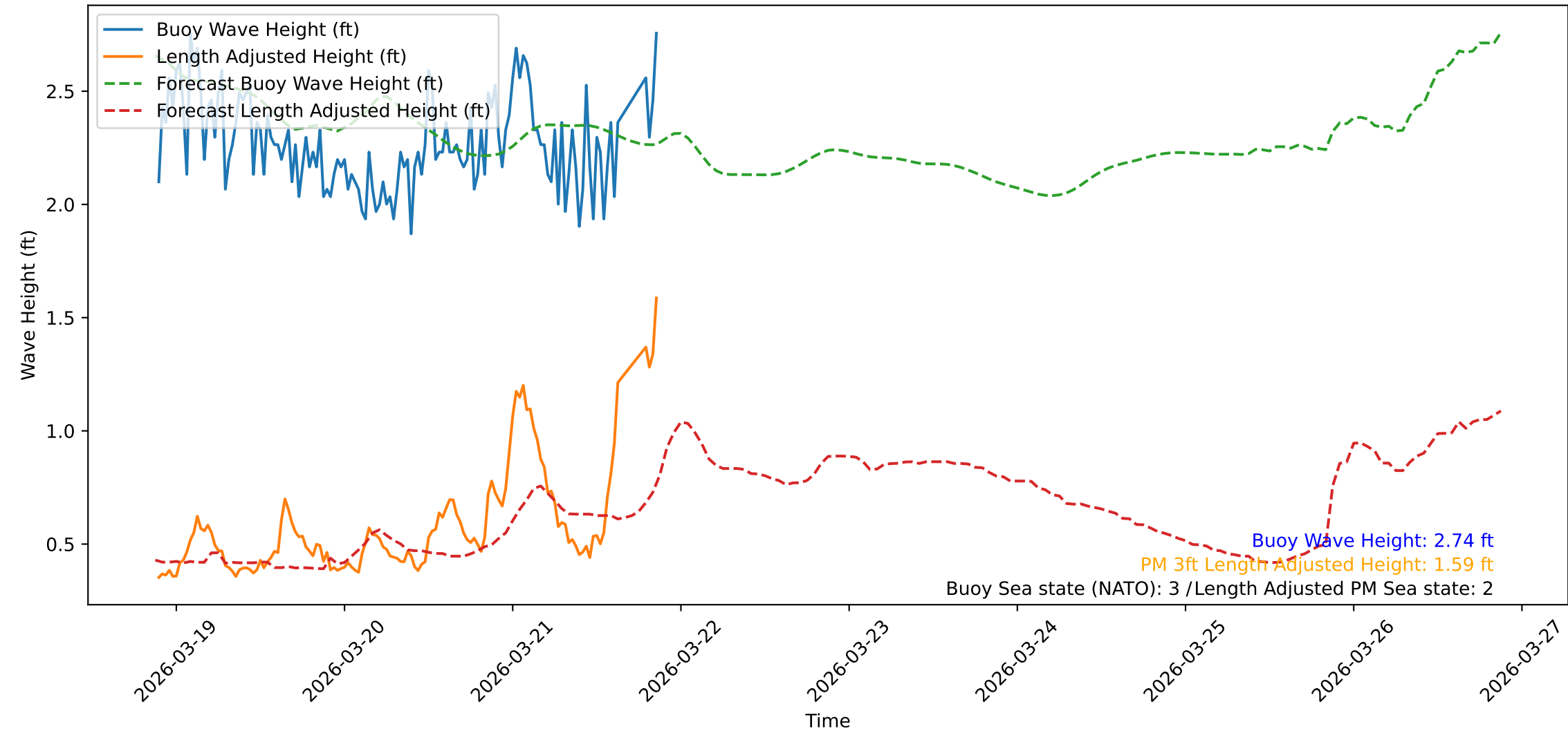
Wave Heights over Time for Red Beach at 2026-03-21 21:10:47
