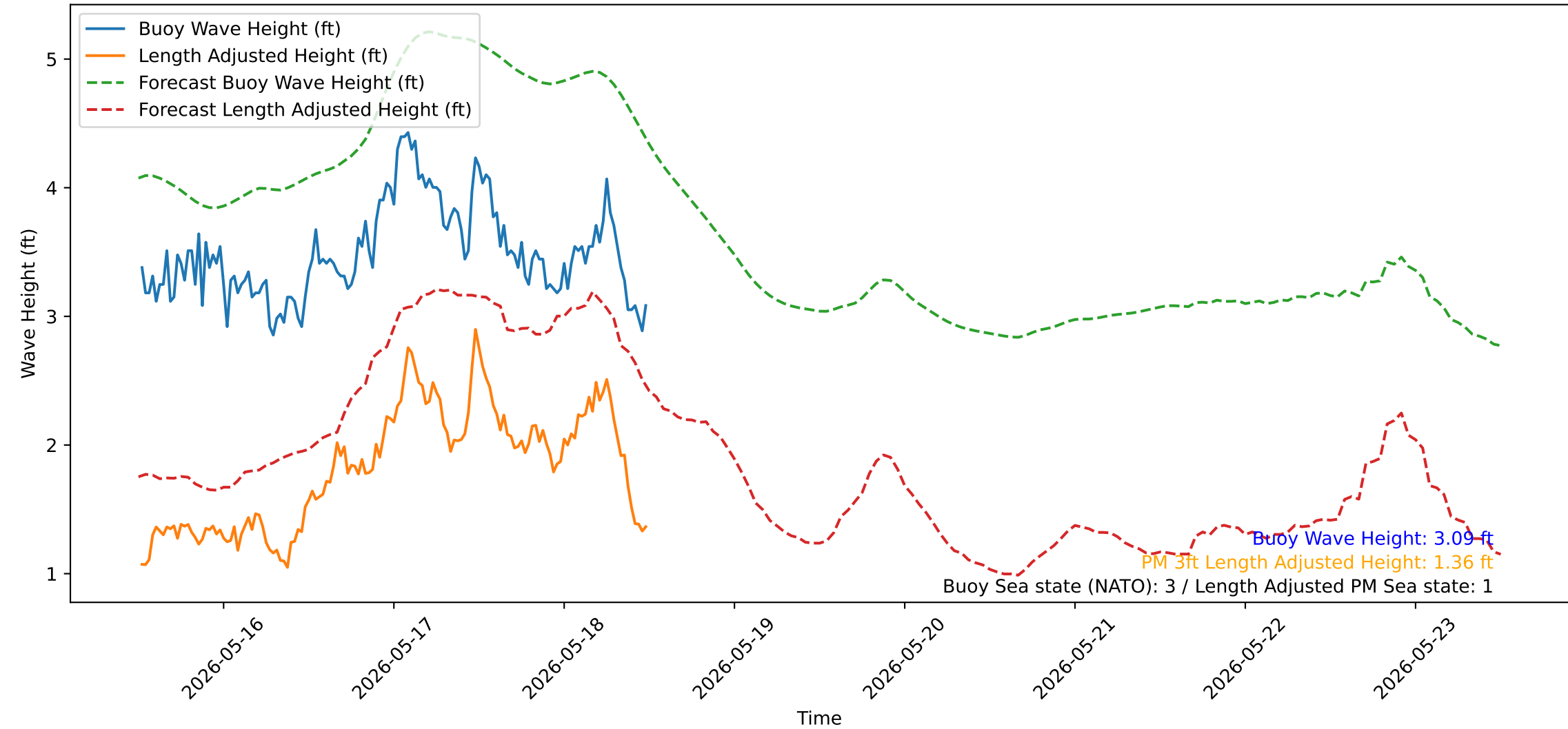
Wave Heights over Time for Green Beach at 2026-05-18 12:21:15
