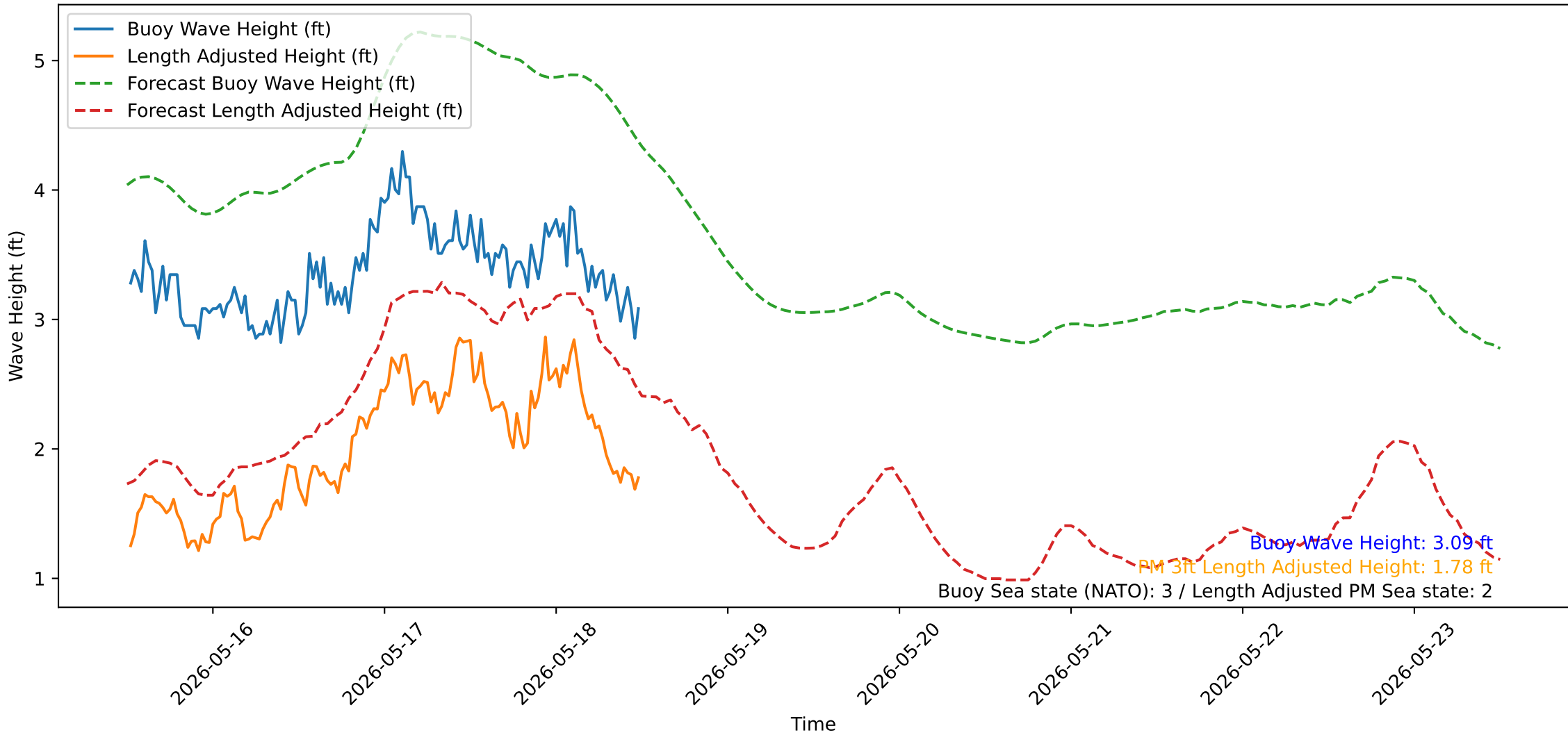
Wave Heights over Time for Oceanside Harbor at 2026-05-18 12:20:32
