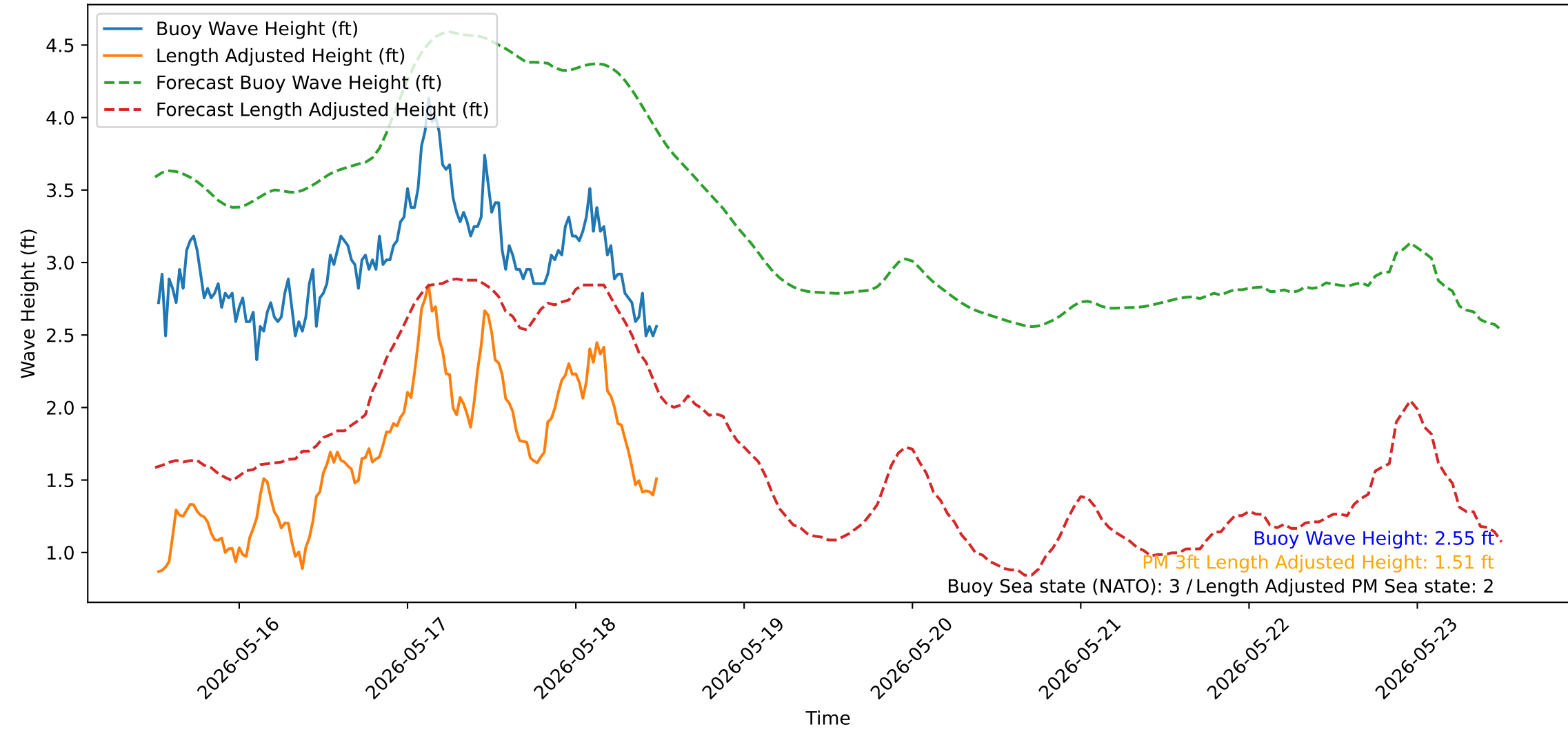
Wave Heights over Time for Red Beach at 2026-05-18 12:20:52
