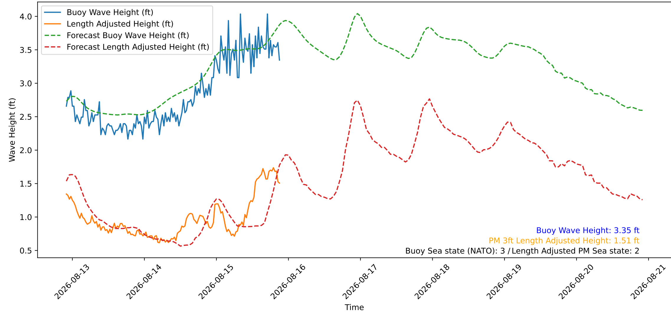
Wave Heights over Time for Red Beach at 2026-08-15 21:50:47
