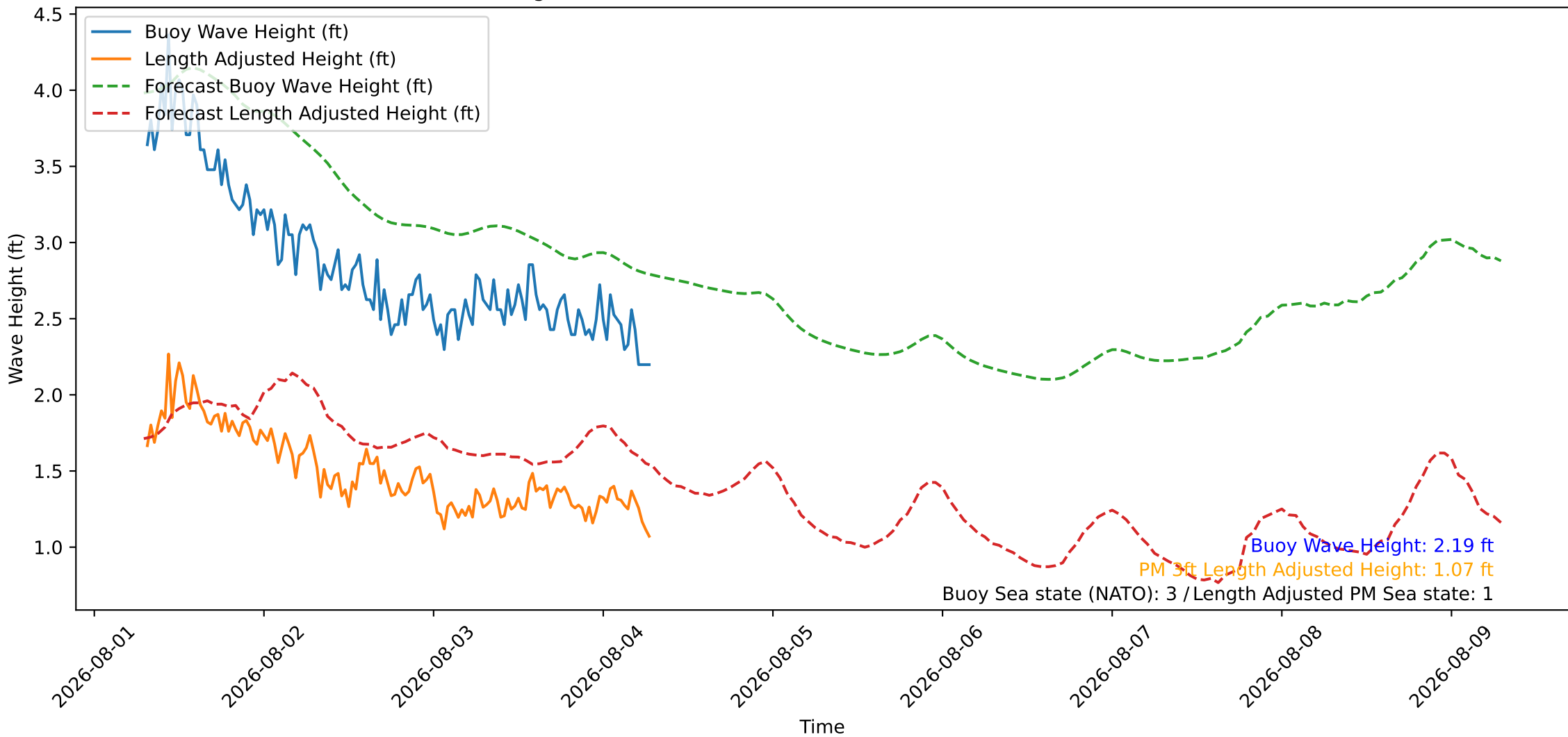
Wave Heights over Time for Oceanside Harbor at 2026-08-04 07:20:26
