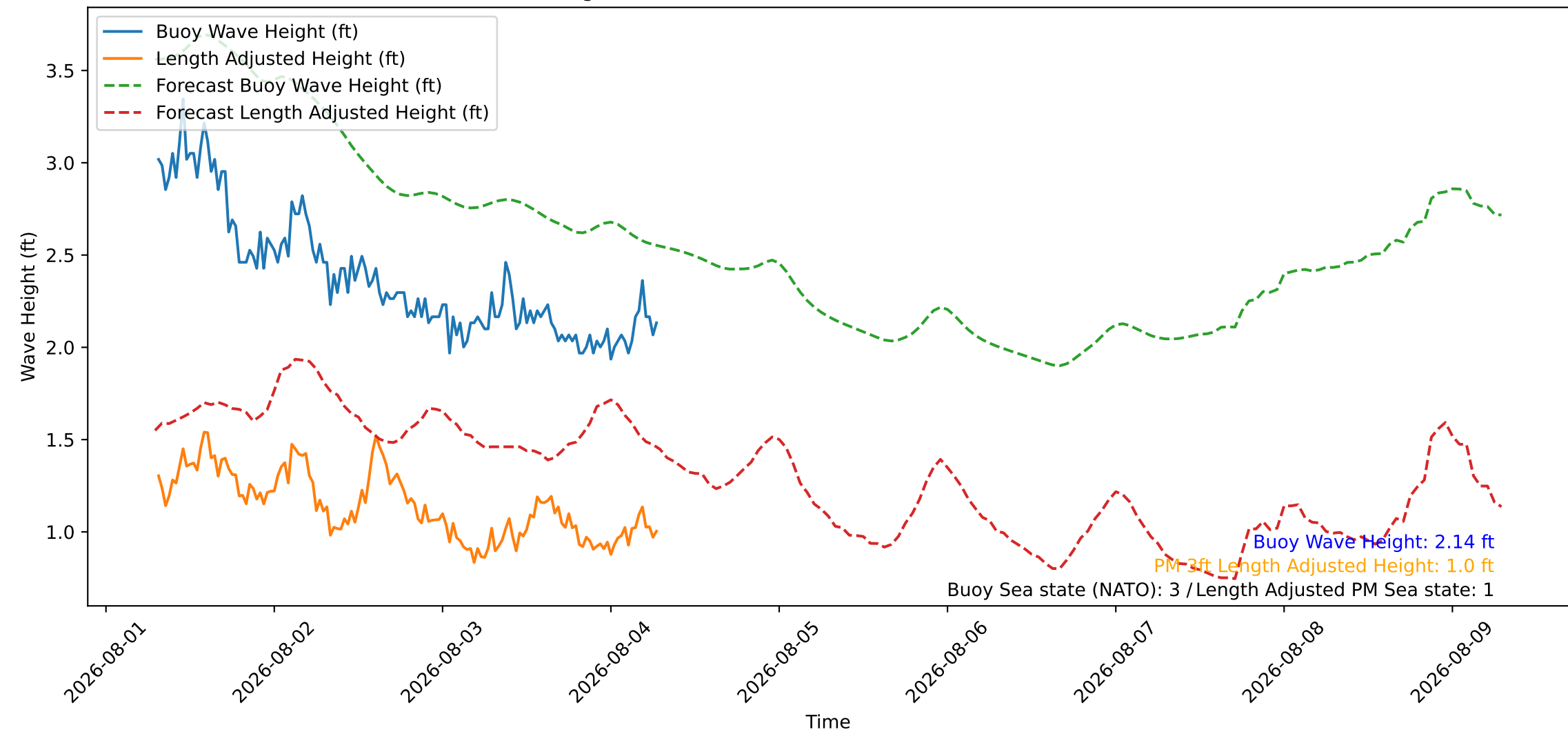
Wave Heights over Time for Red Beach at 2026-08-04 07:20:46
