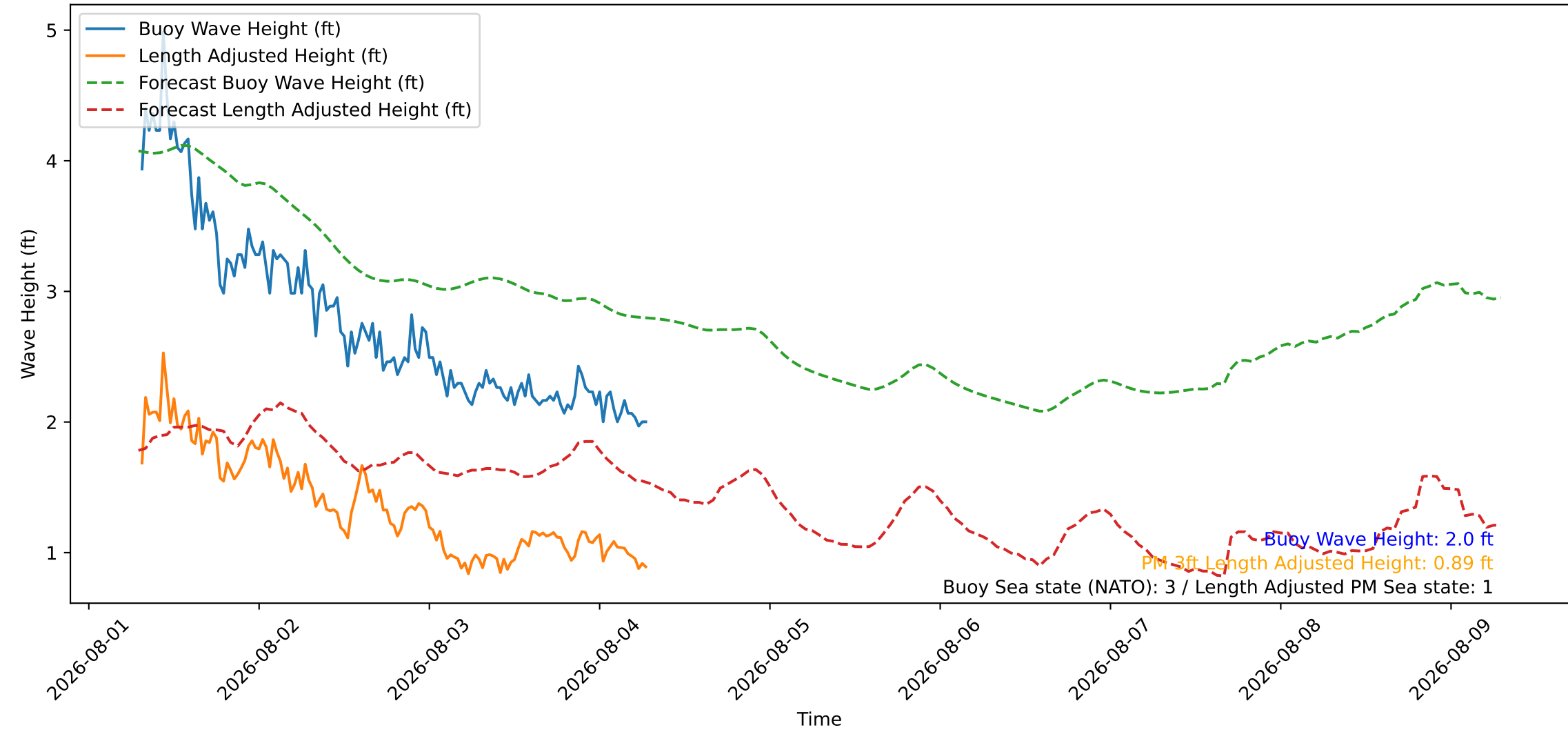
Wave Heights over Time for Green Beach at 2026-08-04 07:21:09
