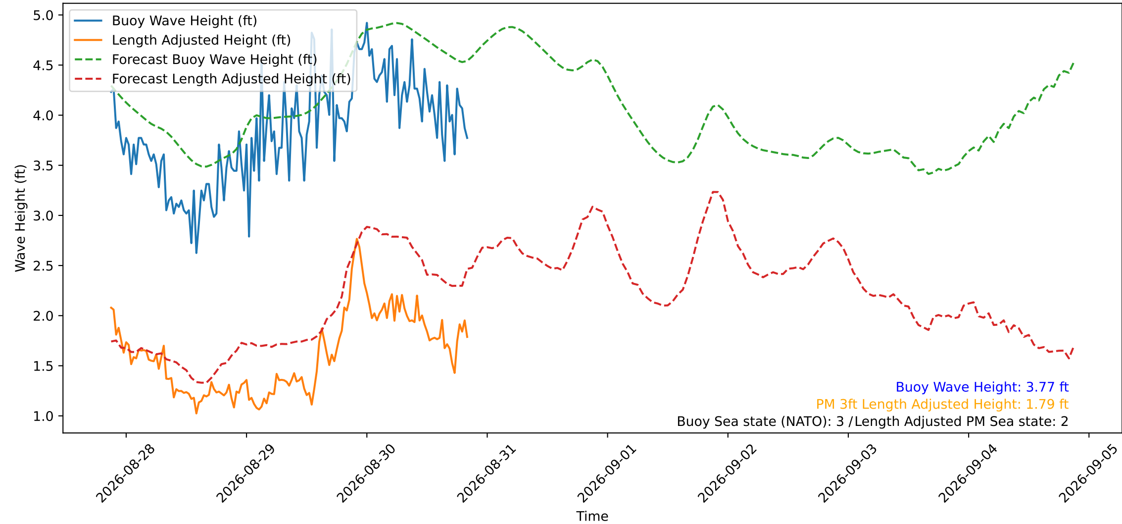
Wave Heights over Time for Green Beach at 2026-08-30 20:41:12
