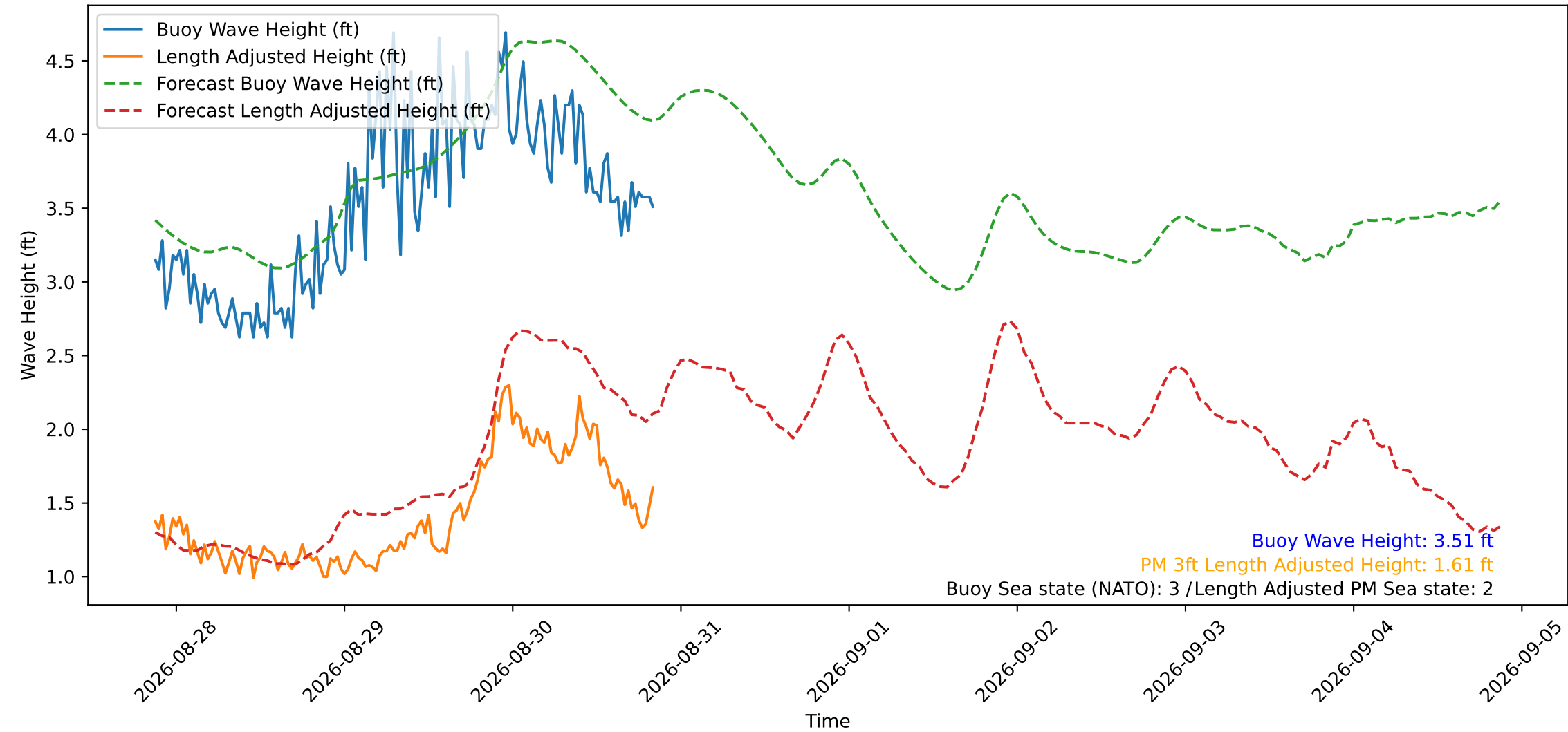
Wave Heights over Time for Red Beach at 2026-08-30 20:40:50
