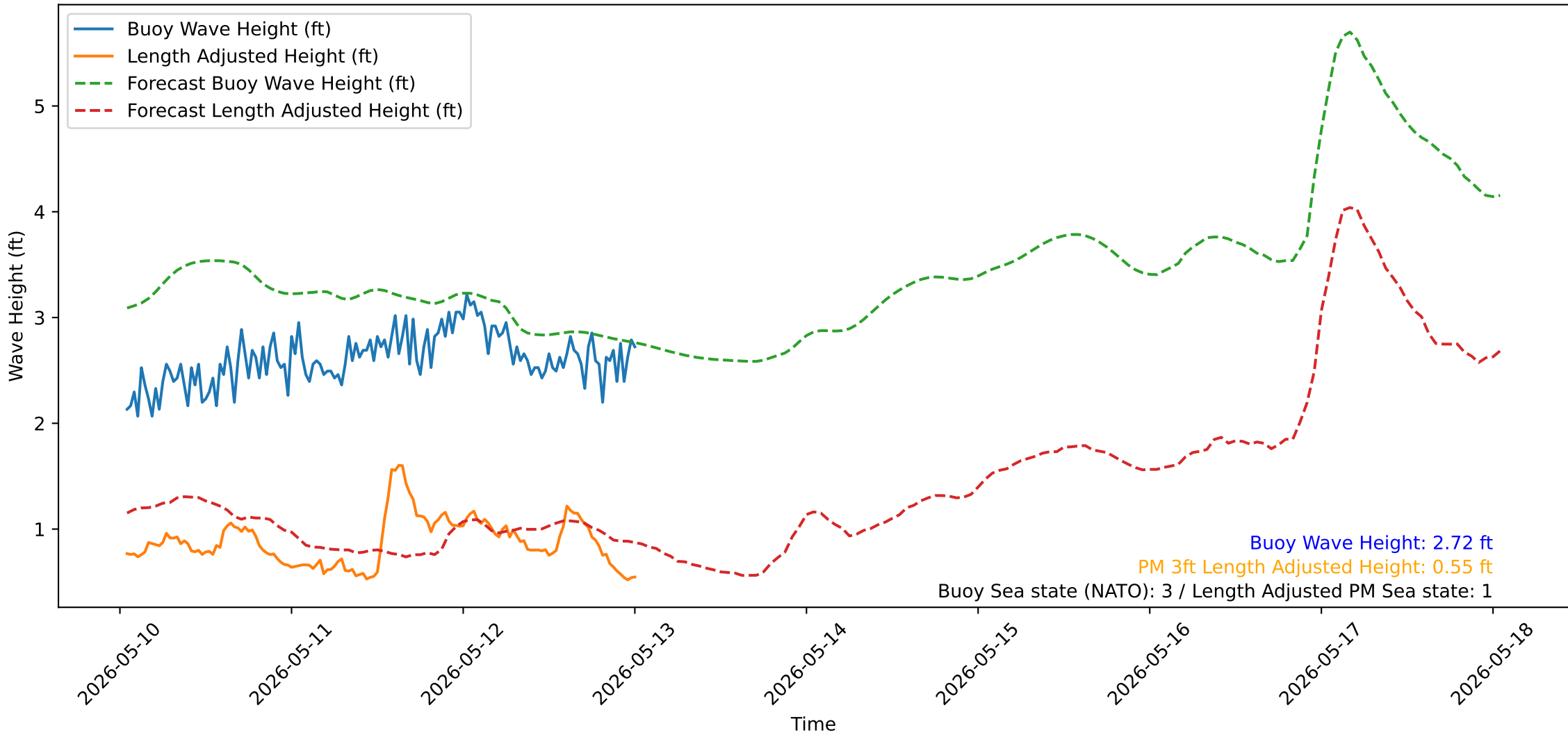
Wave Heights over Time for Red Beach at 2026-05-13 00:50:52
