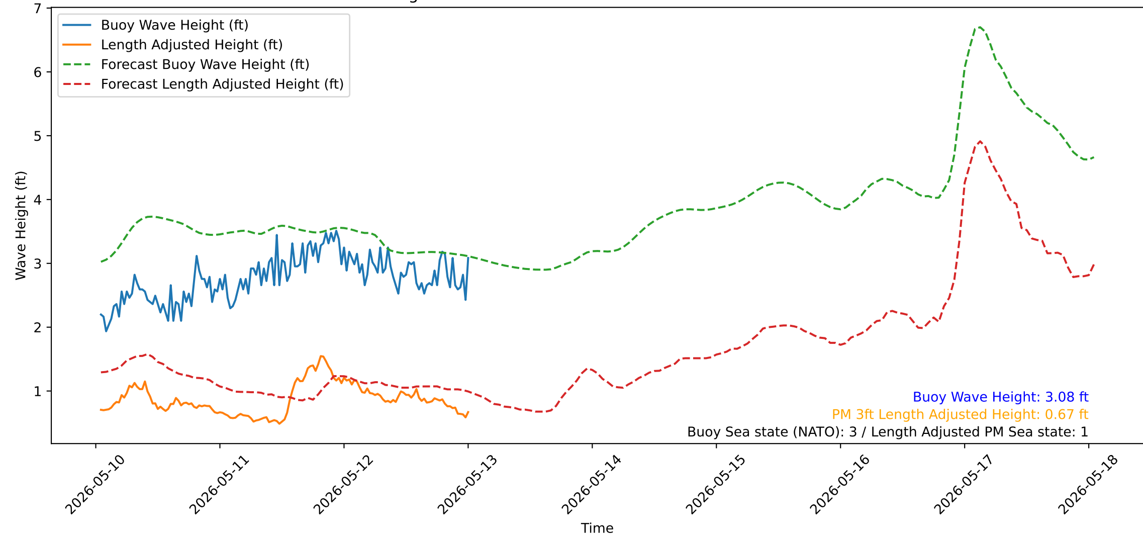
Wave Heights over Time for Green Beach at 2026-05-13 00:51:14
